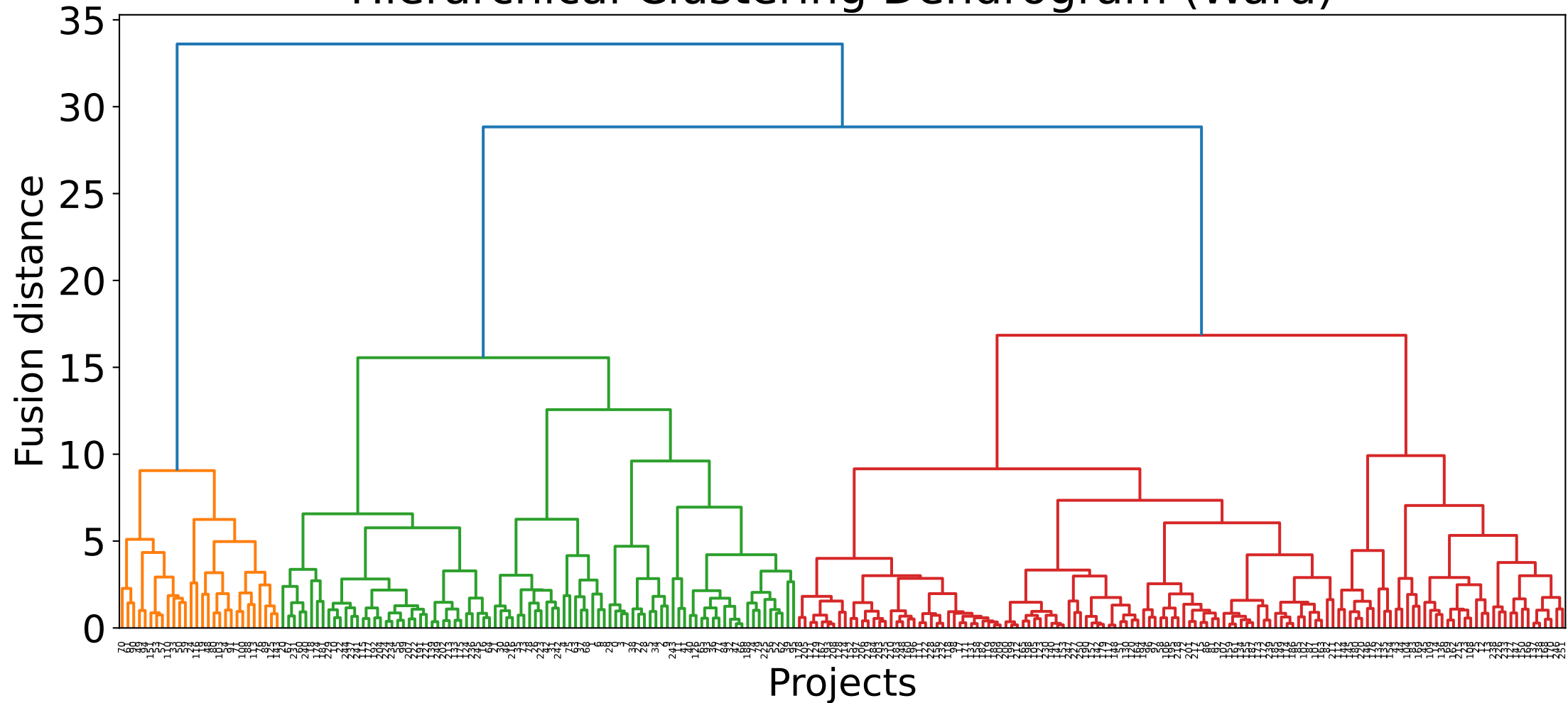
Hierarchical Clustering Dendrogram (Ward)
