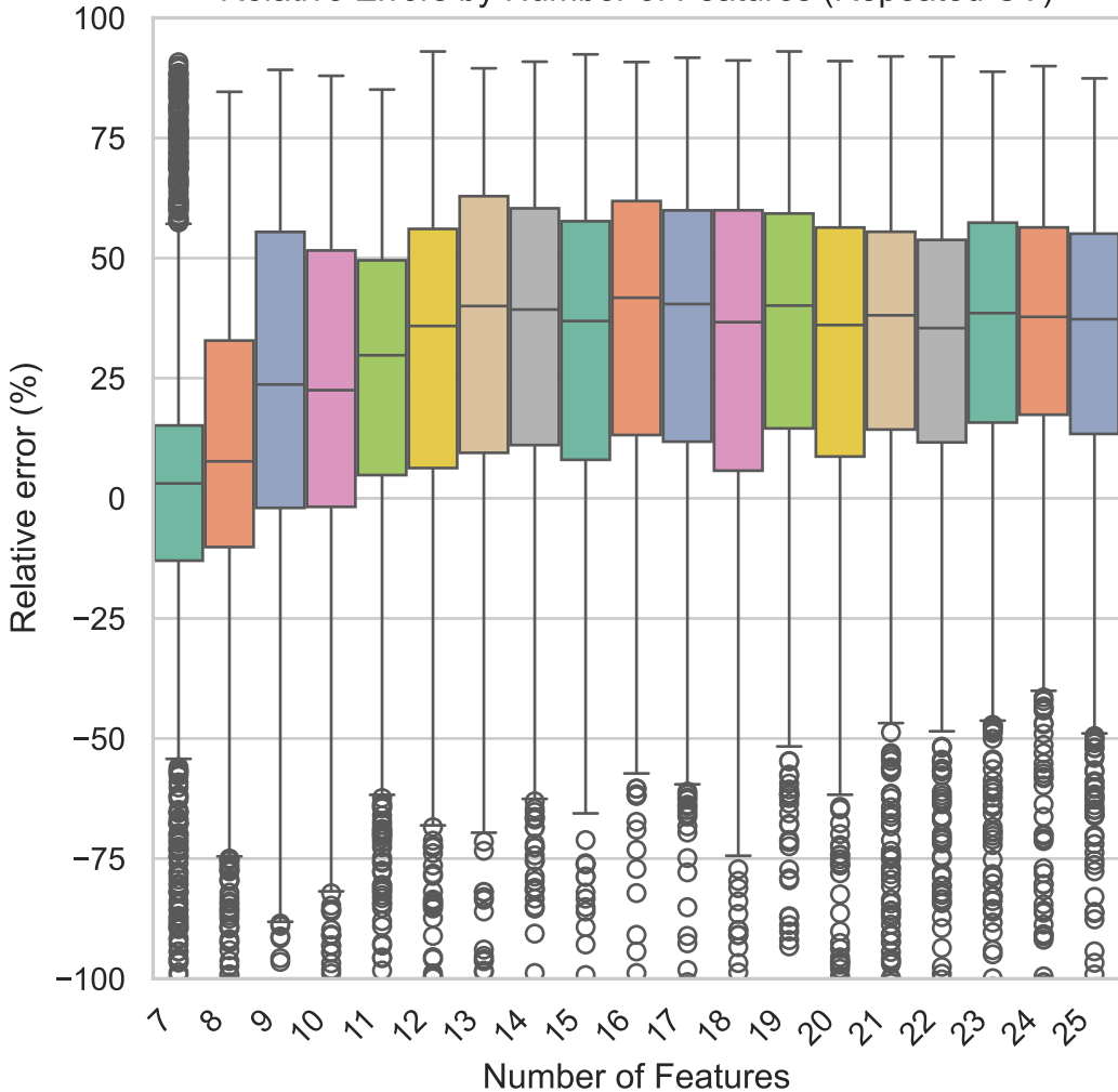
Relative Errors by Number of Features (Repeated CV)
