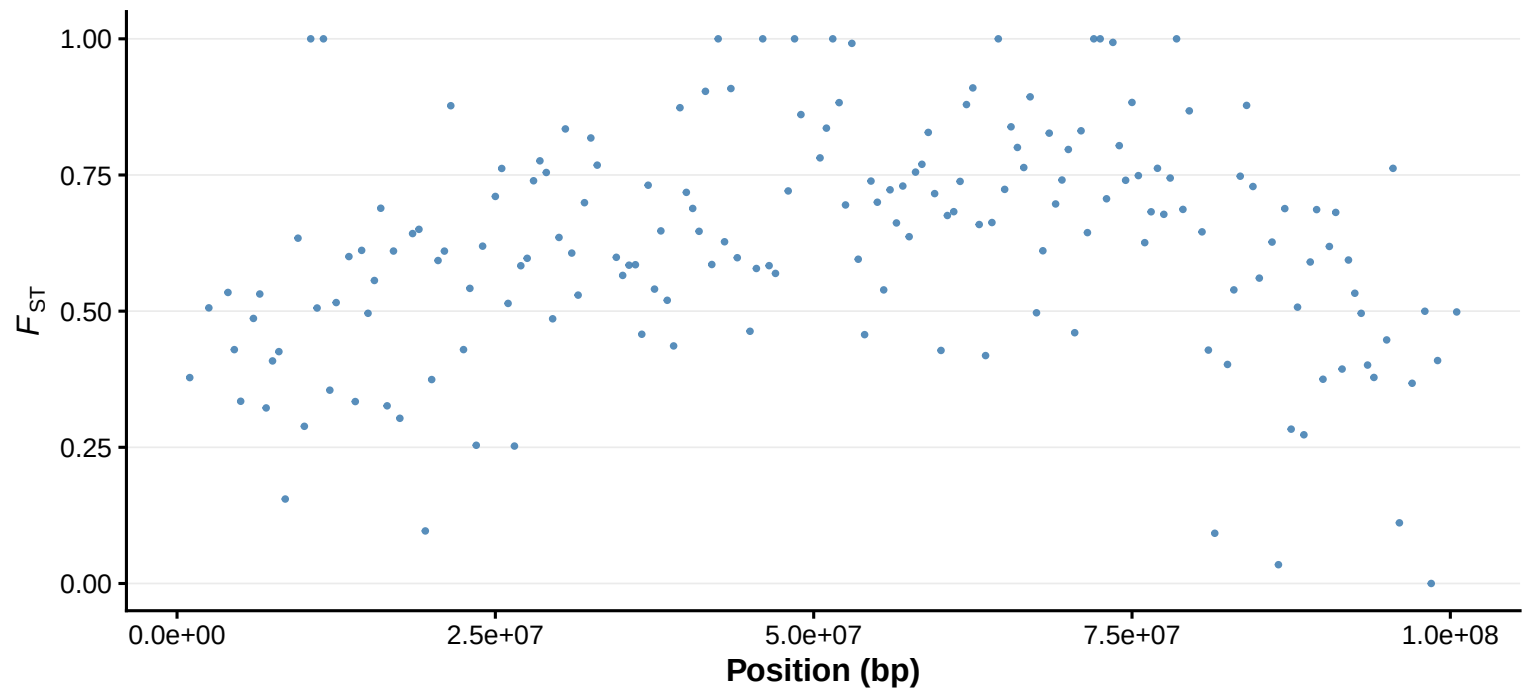
fst CRT RR vs YCT Omy05
