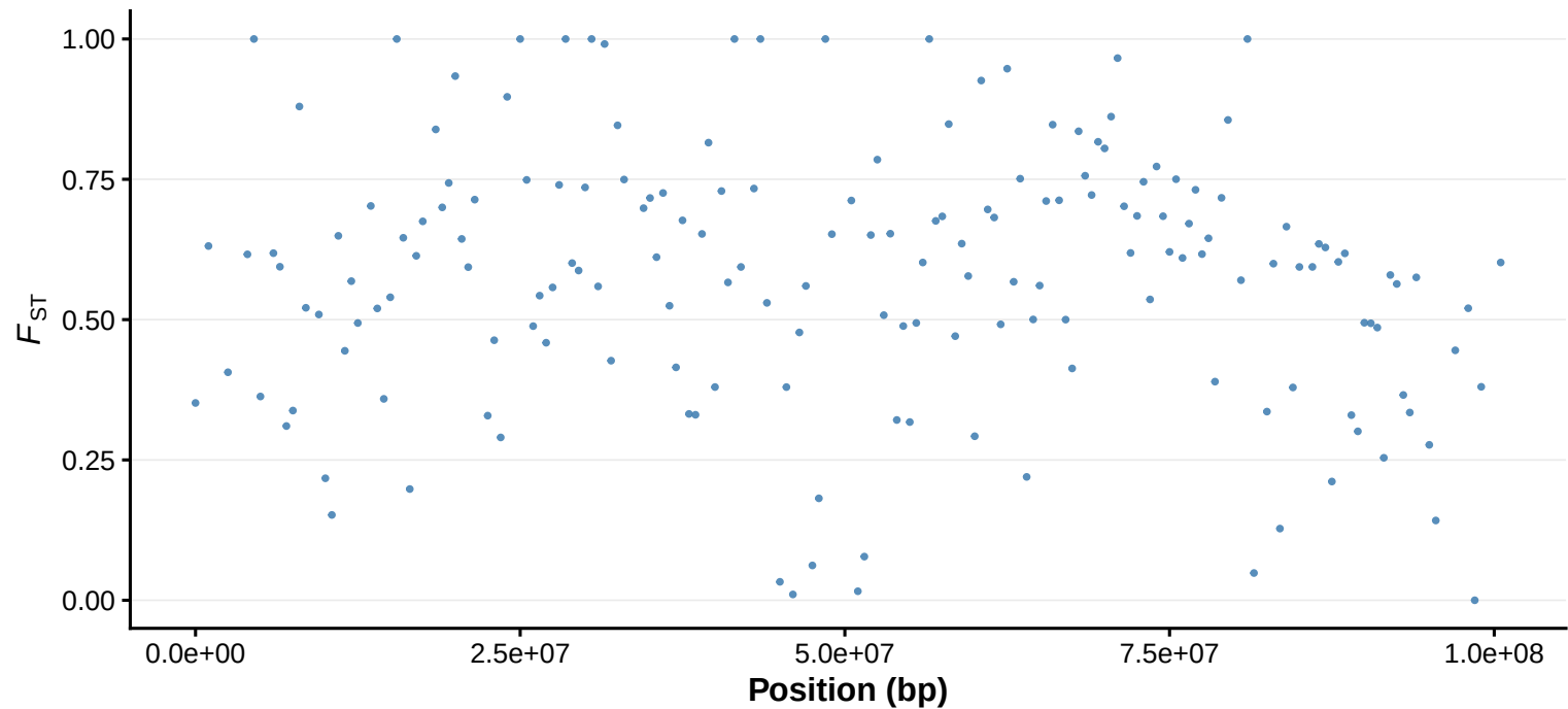
fst WCT vs YCT Omy05
