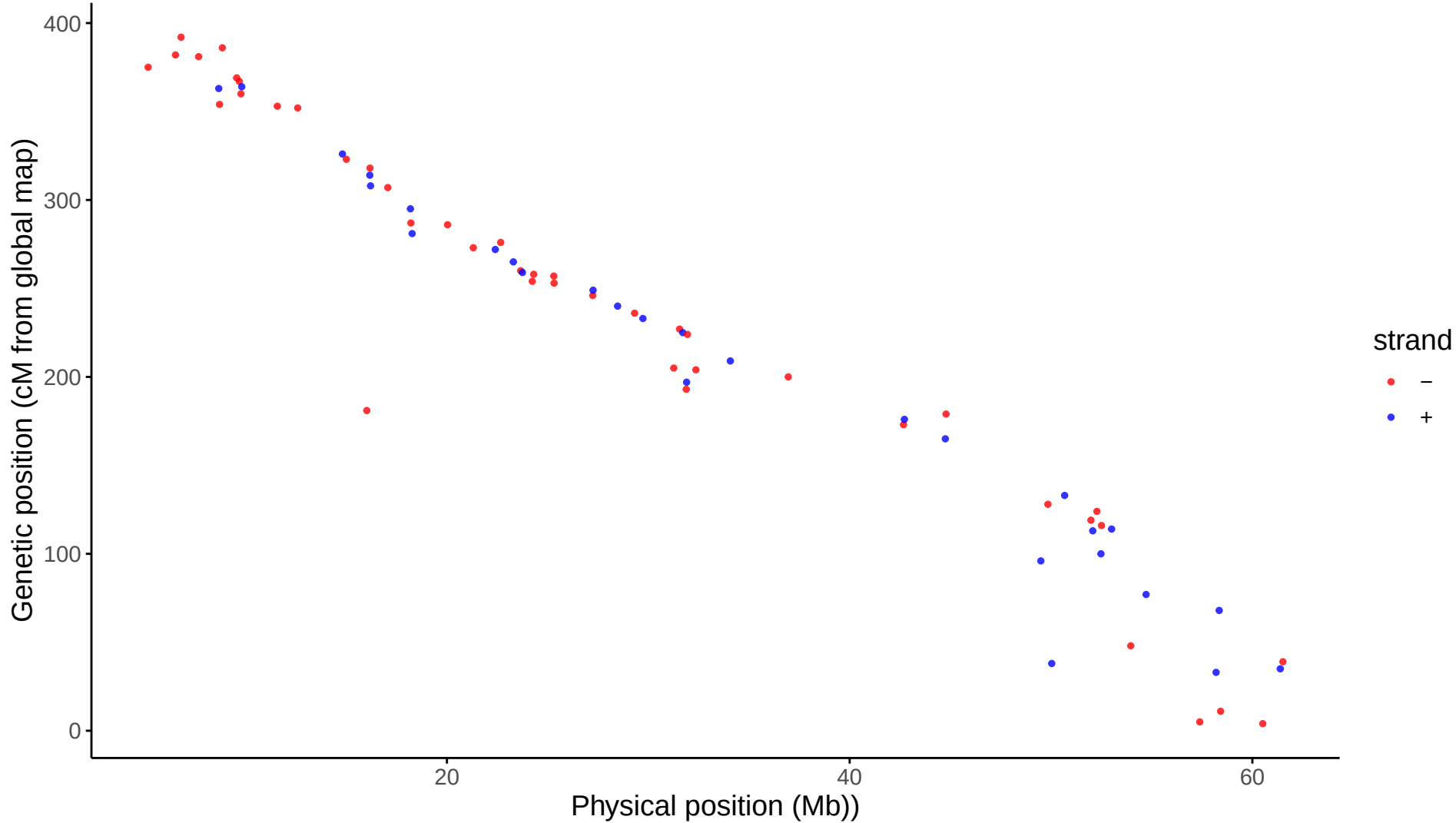
Wolf: LG15 markers aligned to Omy15
