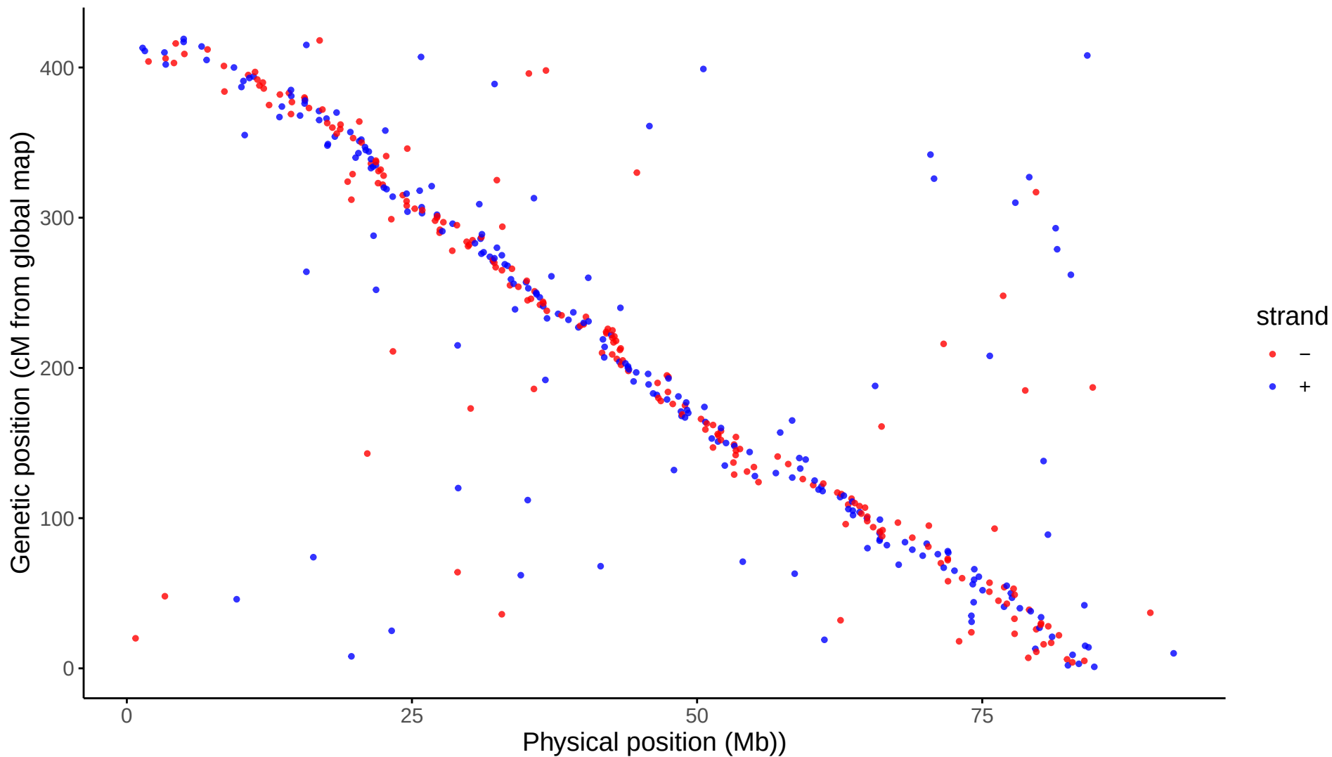
Global: LG01 markers aligned to Omy01
