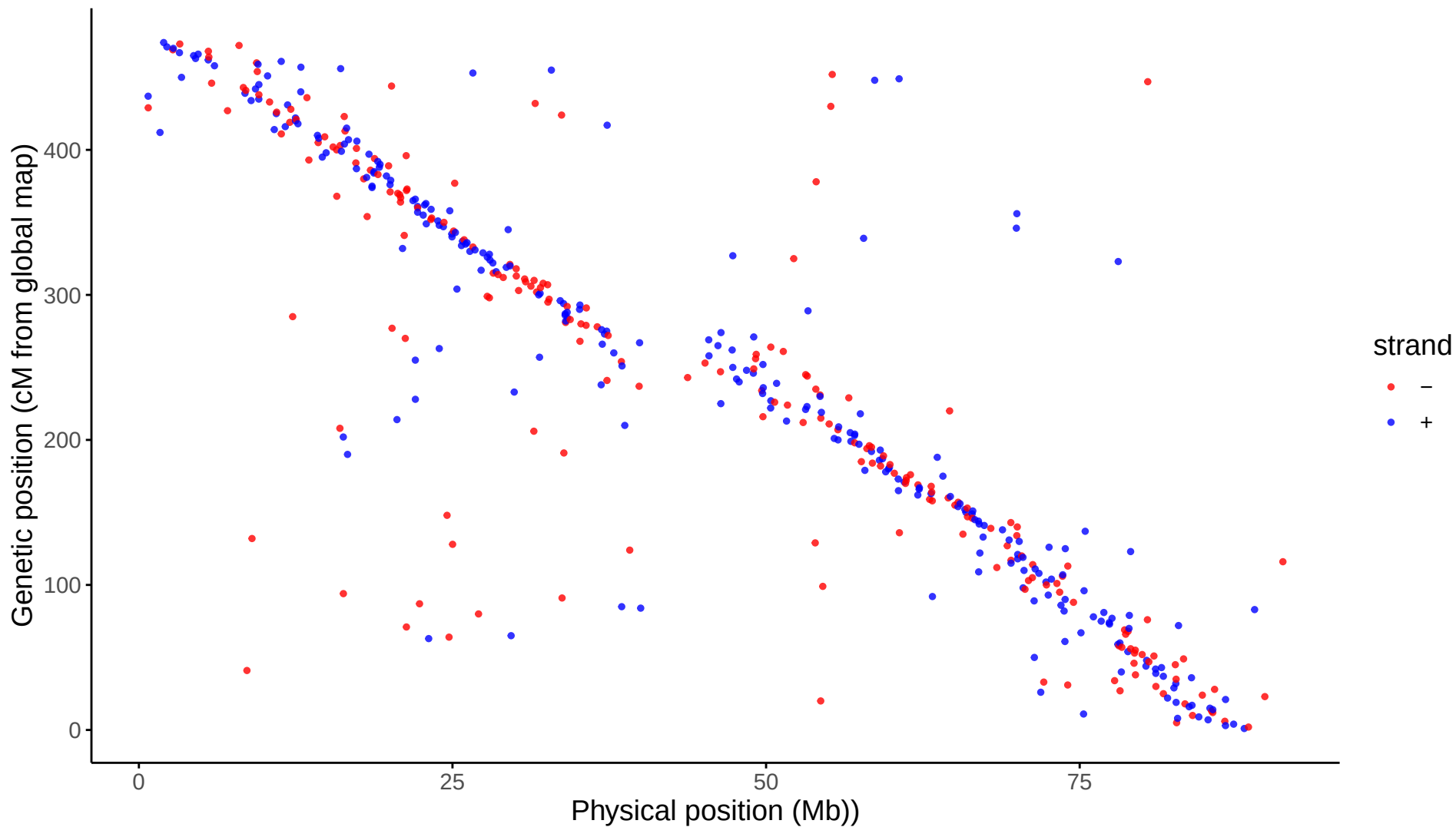
Global: LG08 markers aligned to Omy08
