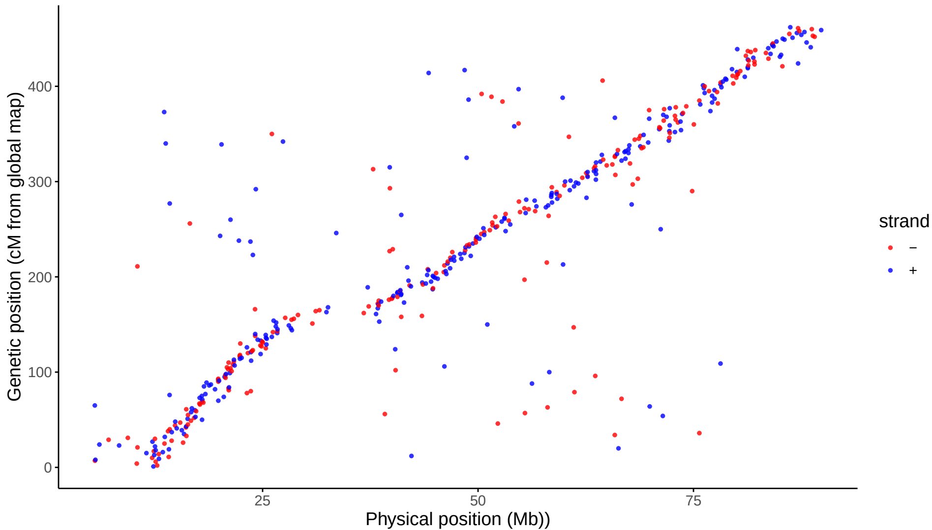
Global: LG07 markers aligned to Omy07
