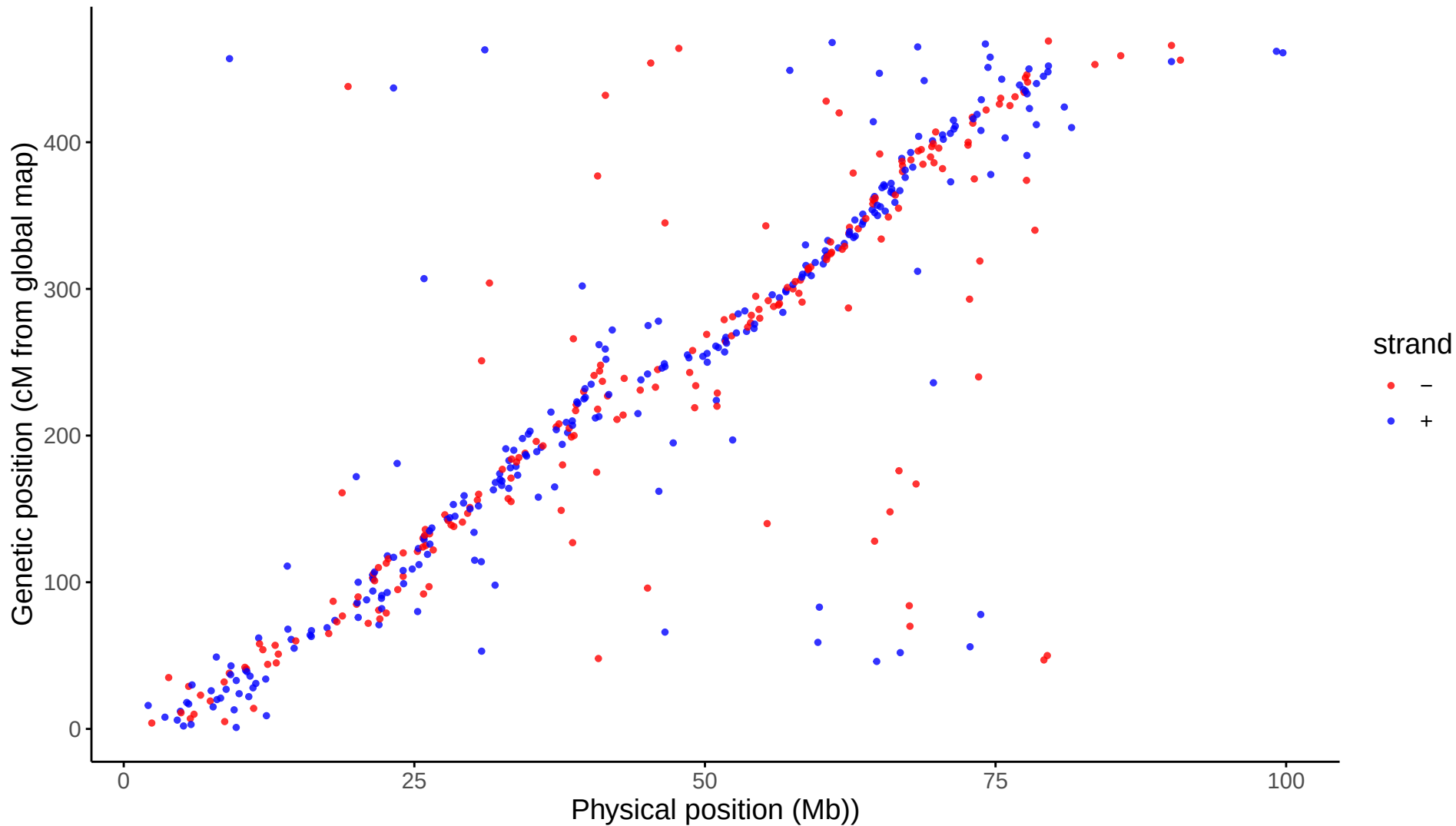
Global: LG06 markers aligned to Omy06
