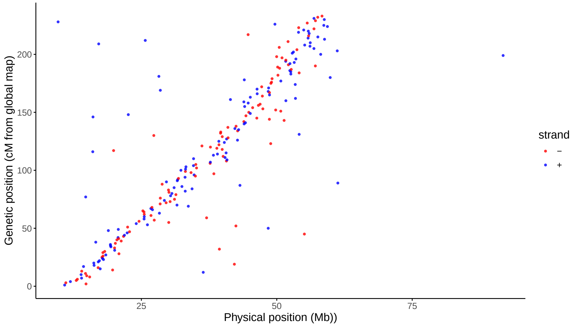
Global: LG23 markers aligned to Omy23
