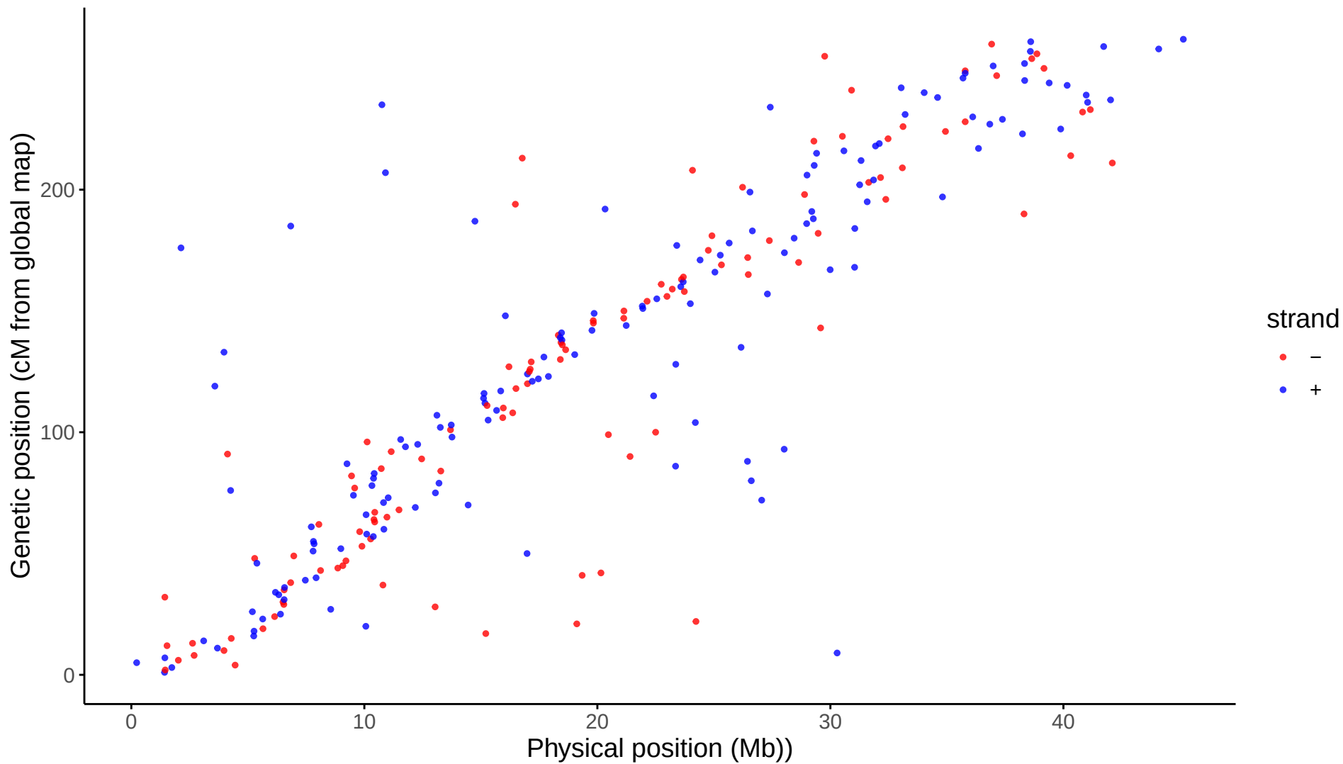
Global: LG24 markers aligned to Omy24
