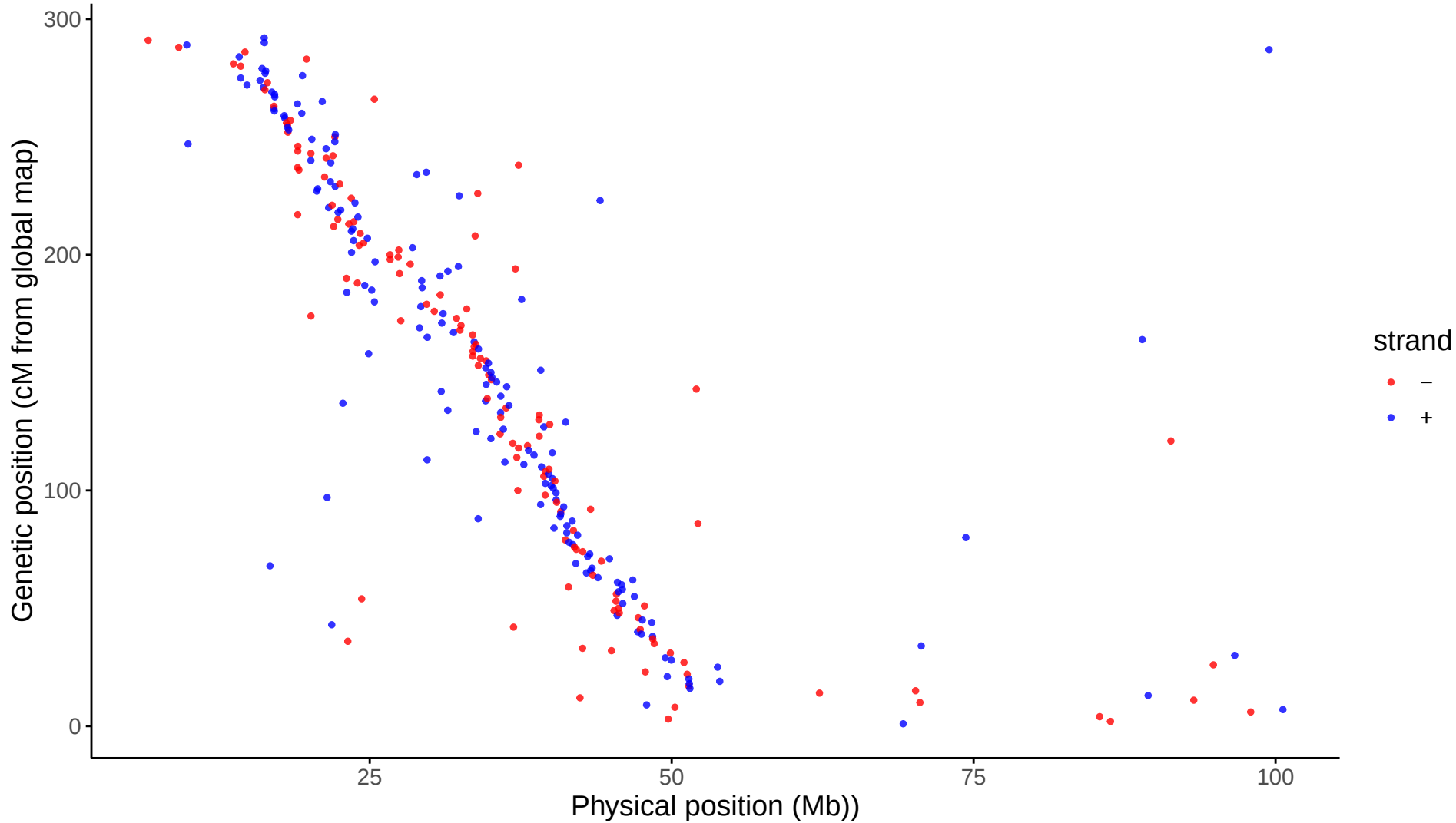
Global: LG13 markers aligned to Omy13
