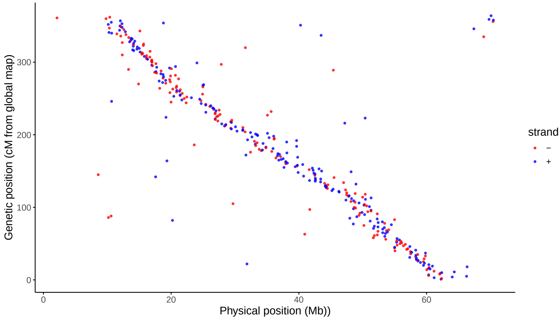
Global: LG19 markers aligned to Omy19
