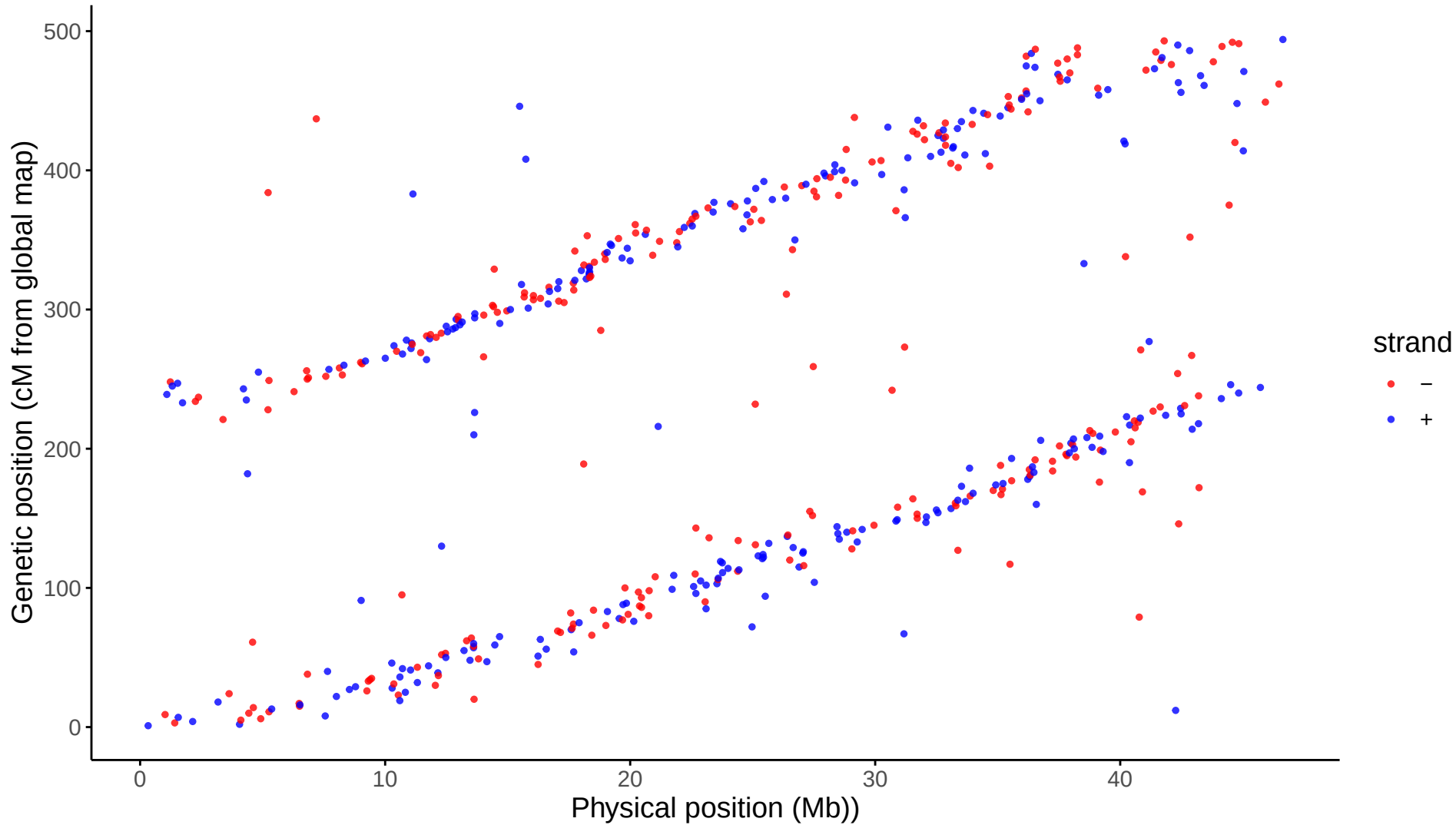
Global: LG04 markers aligned to Omy04
