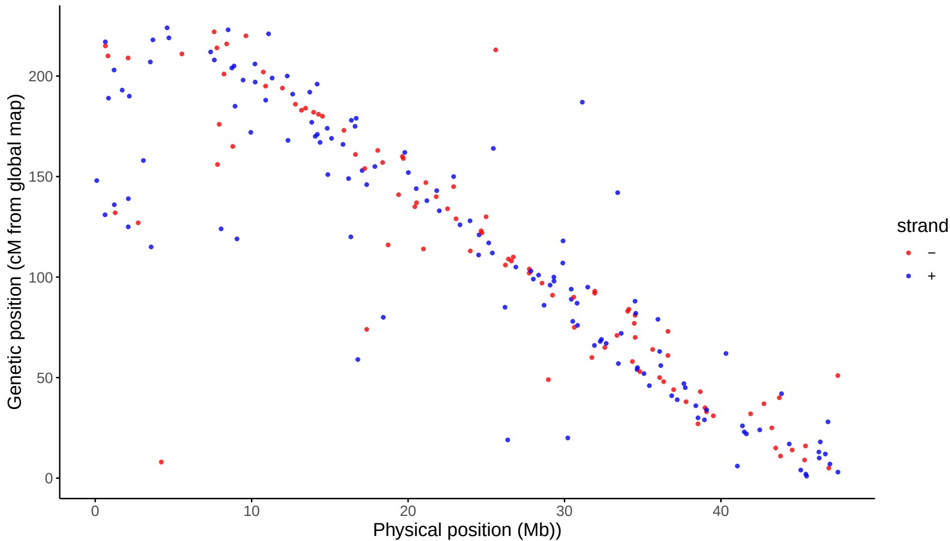
Global: LG29 markers aligned to Omy29
