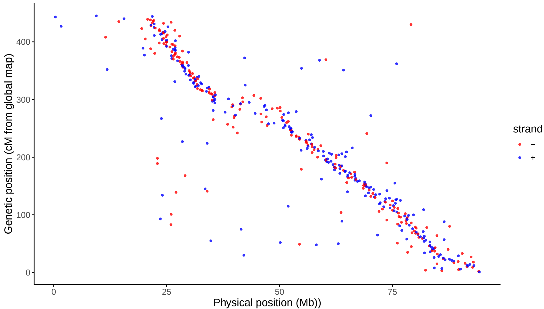
Global: LG17 markers aligned to Omy17
