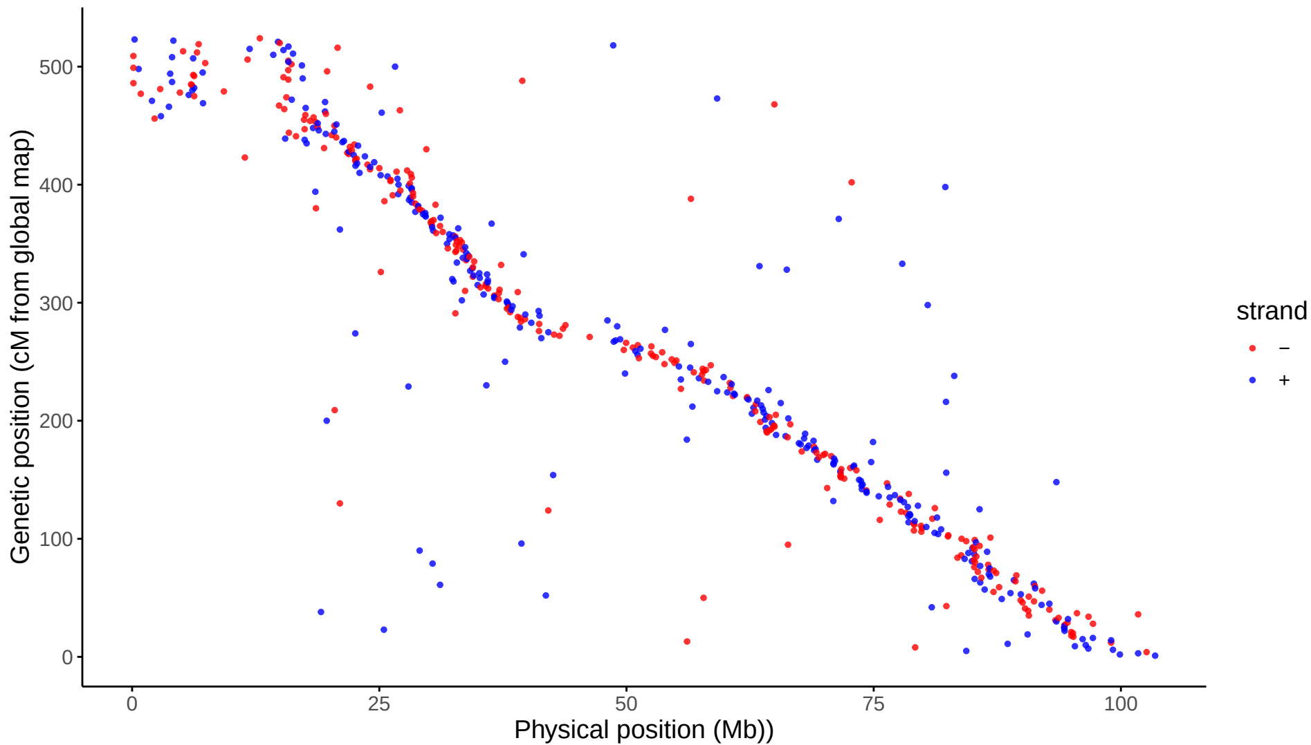
Global: LG02 markers aligned to Omy02
