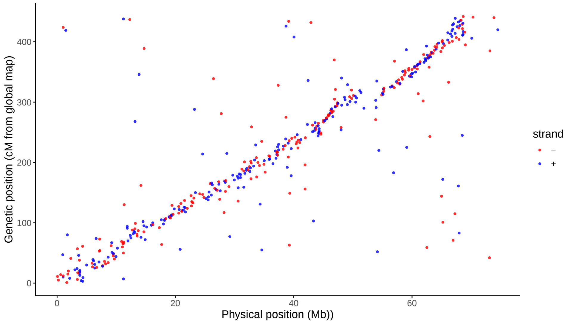
Global: LG10 markers aligned to Omy10
