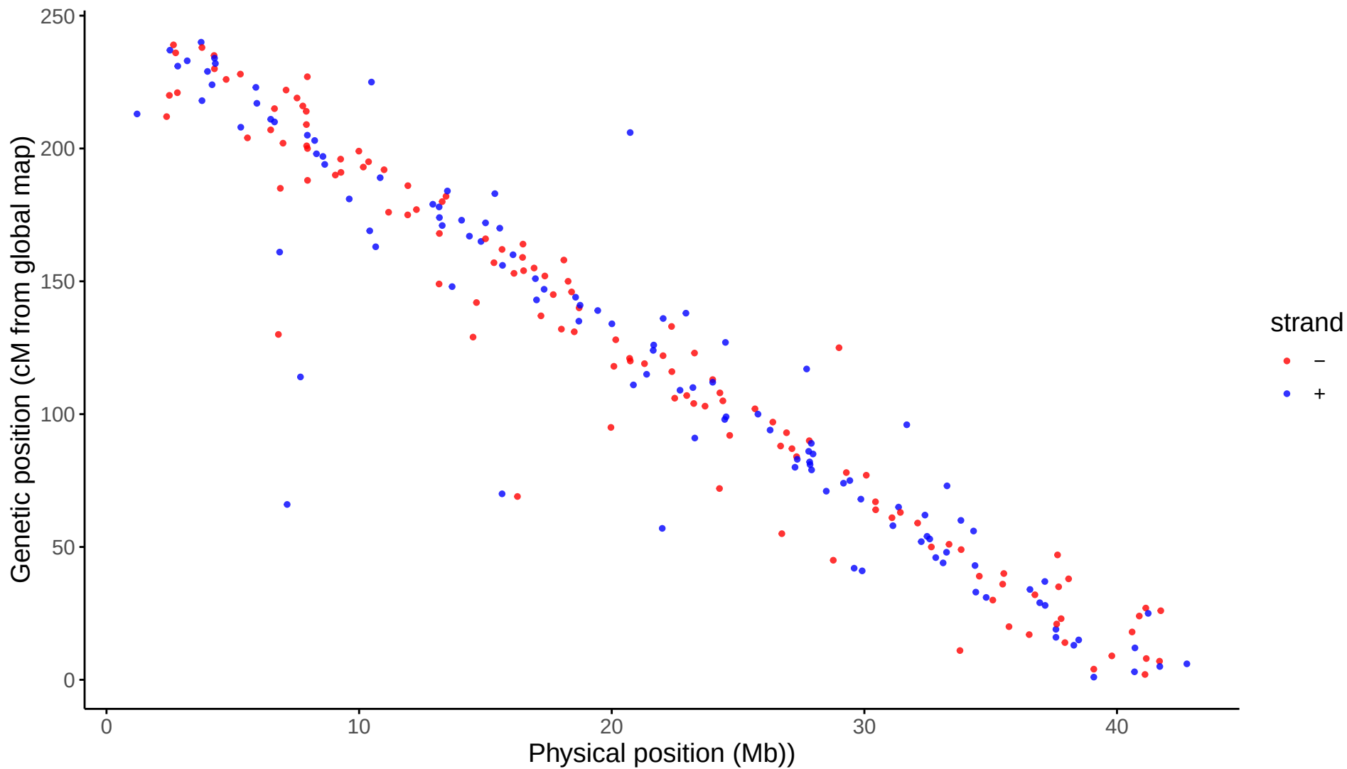
Global: LG28 markers aligned to Omy28
