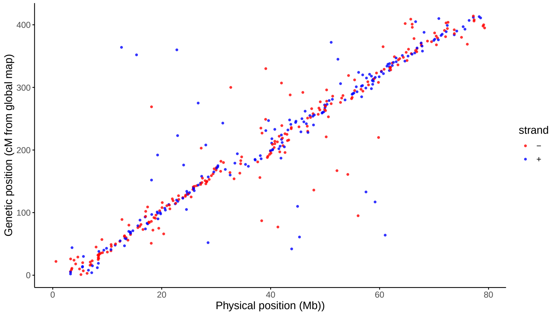
Global: LG09 markers aligned to Omy09
