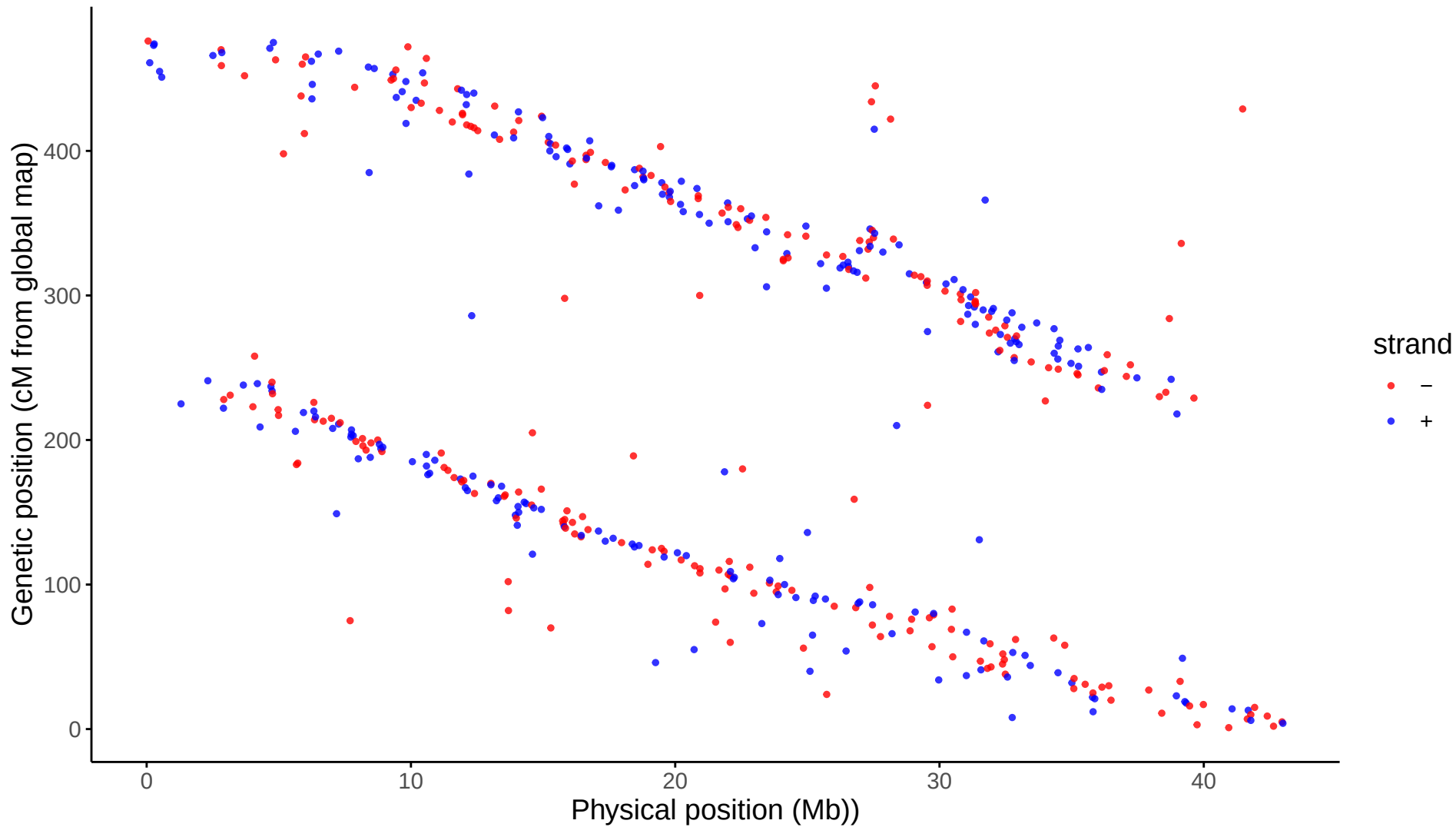
Global: LG14 markers aligned to Omy14
