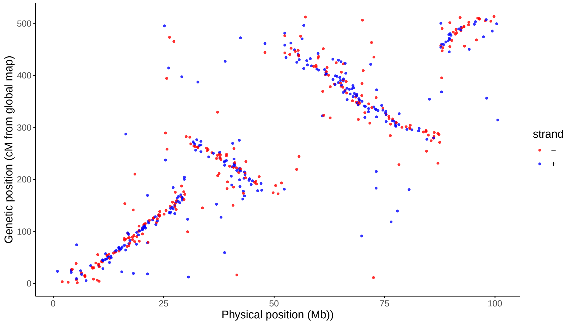
Global: LG05 markers aligned to Omy05
