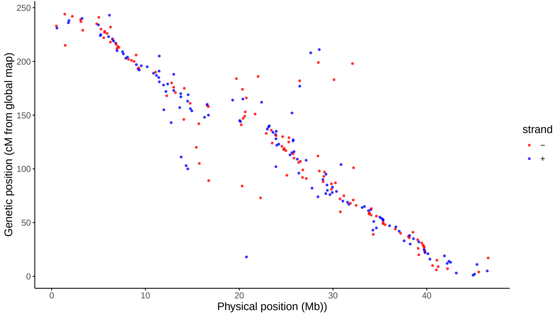
Global: LG20 markers aligned to Omy20
