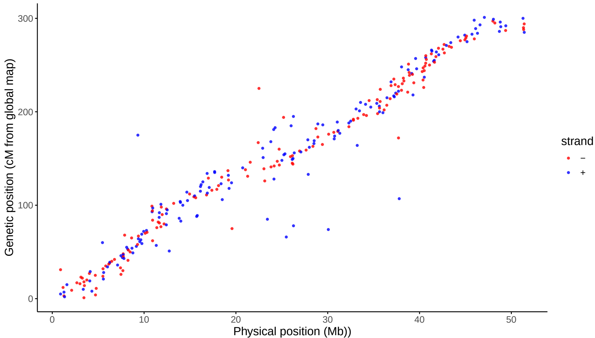
Global: LG22 markers aligned to Omy22
