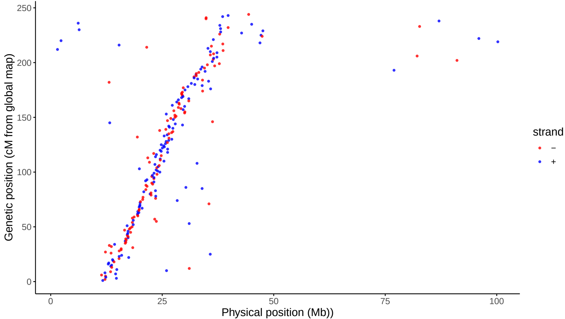
Global: LG26 markers aligned to Omy26
