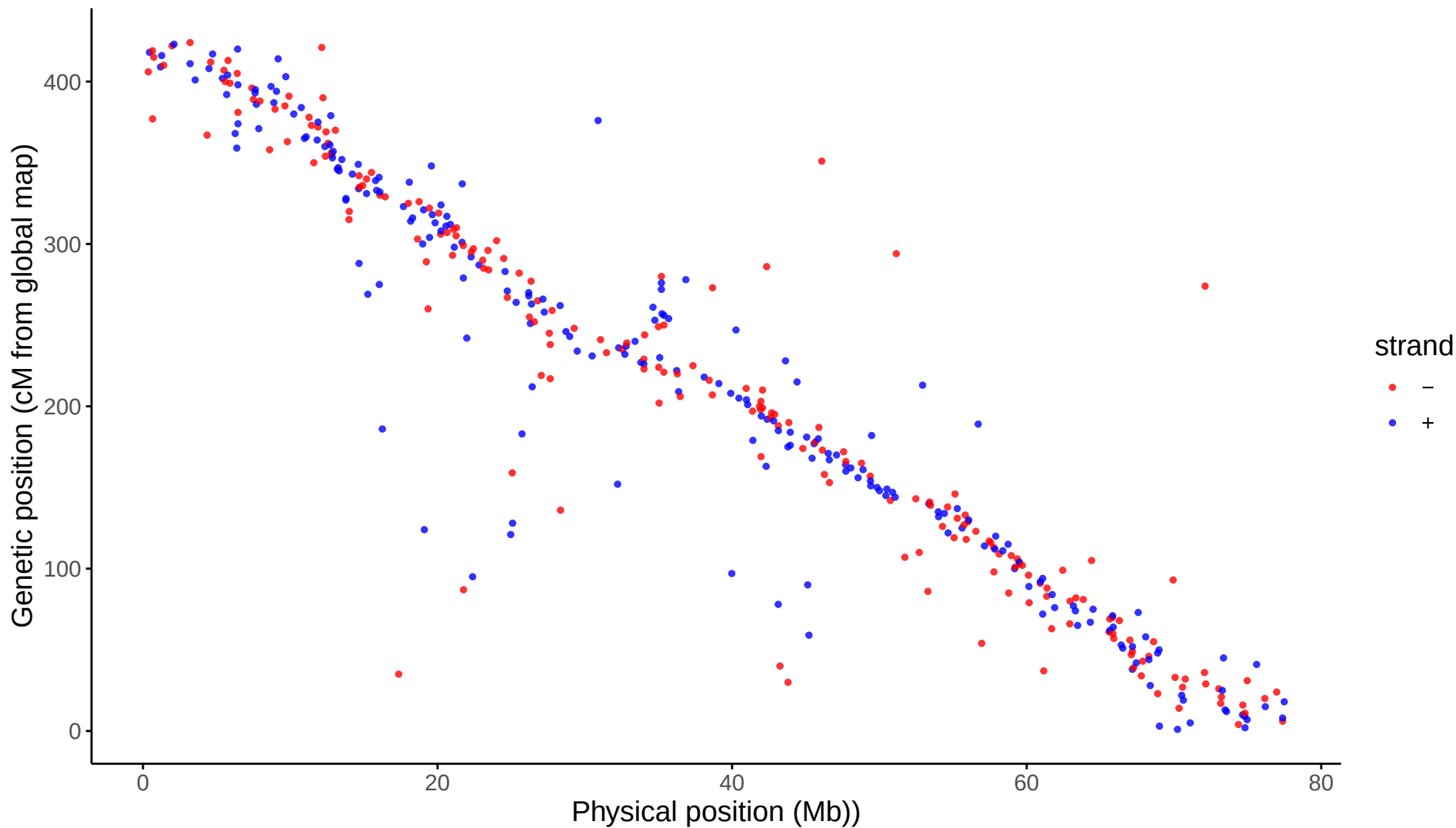
Global: LG16 markers aligned to Omy16
