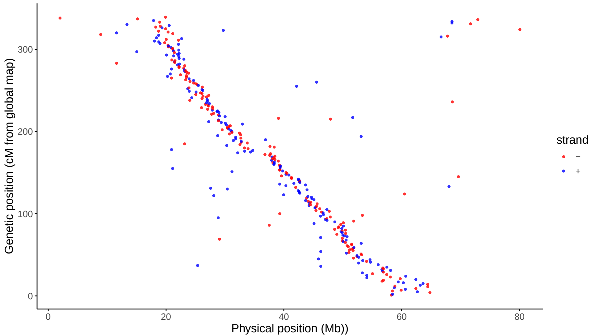
Global: LG21 markers aligned to Omy21
