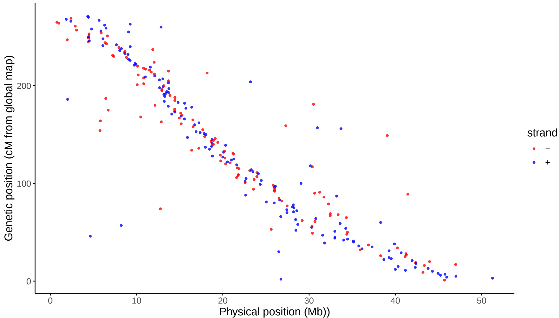
Global: LG27 markers aligned to Omy27
