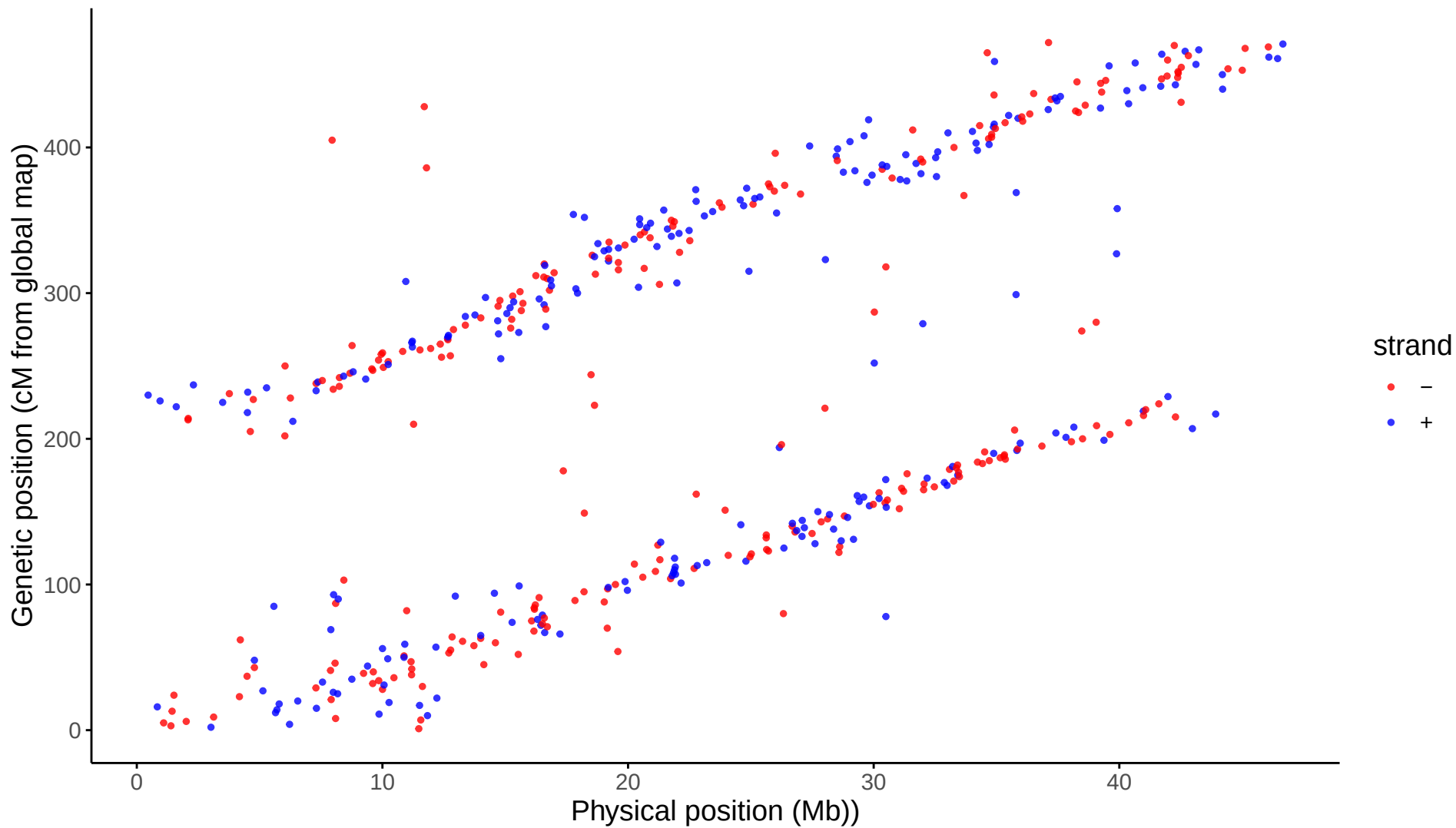
Global: LG25 markers aligned to Omy25
