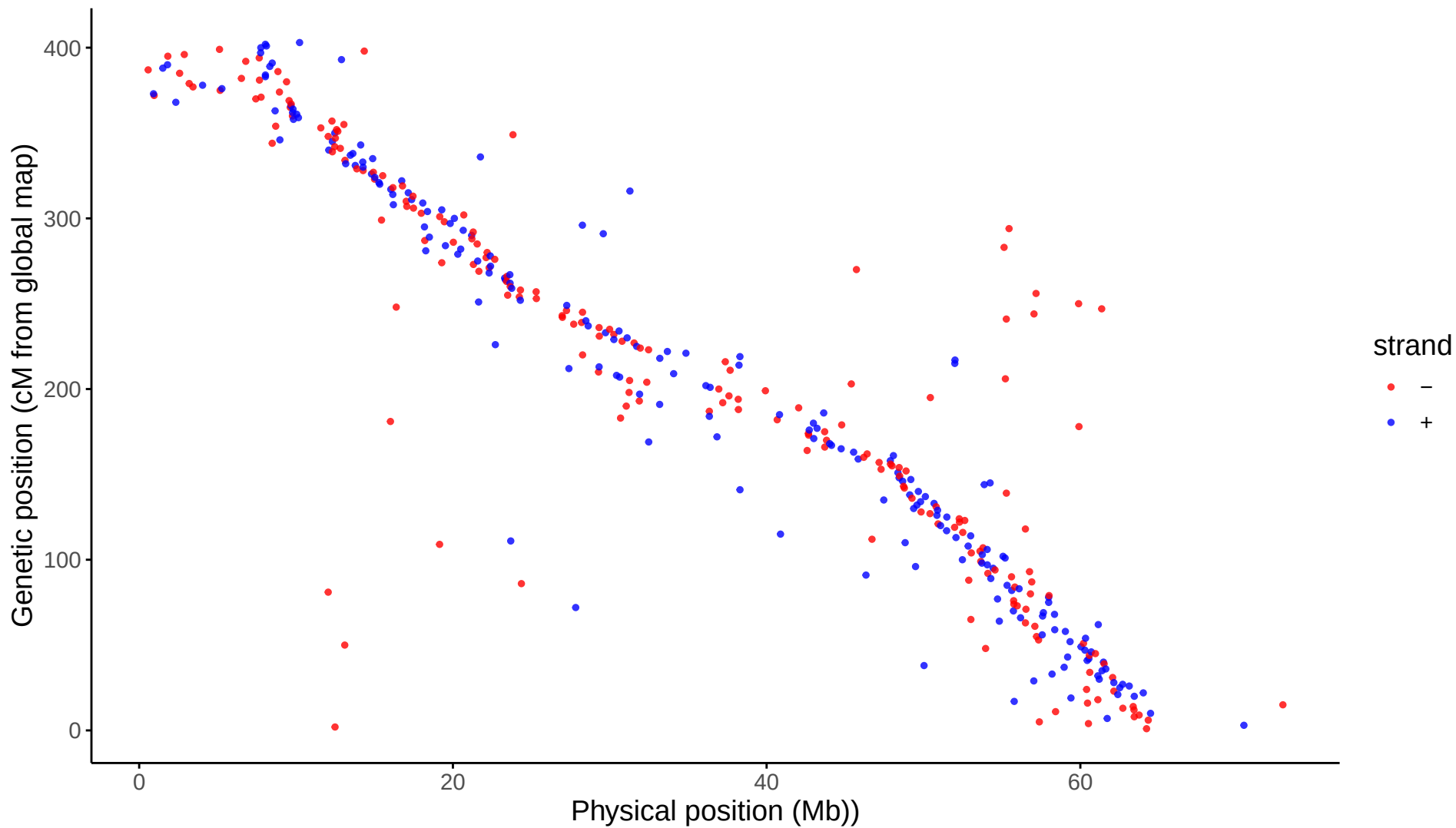
Global: LG15 markers aligned to Omy15
