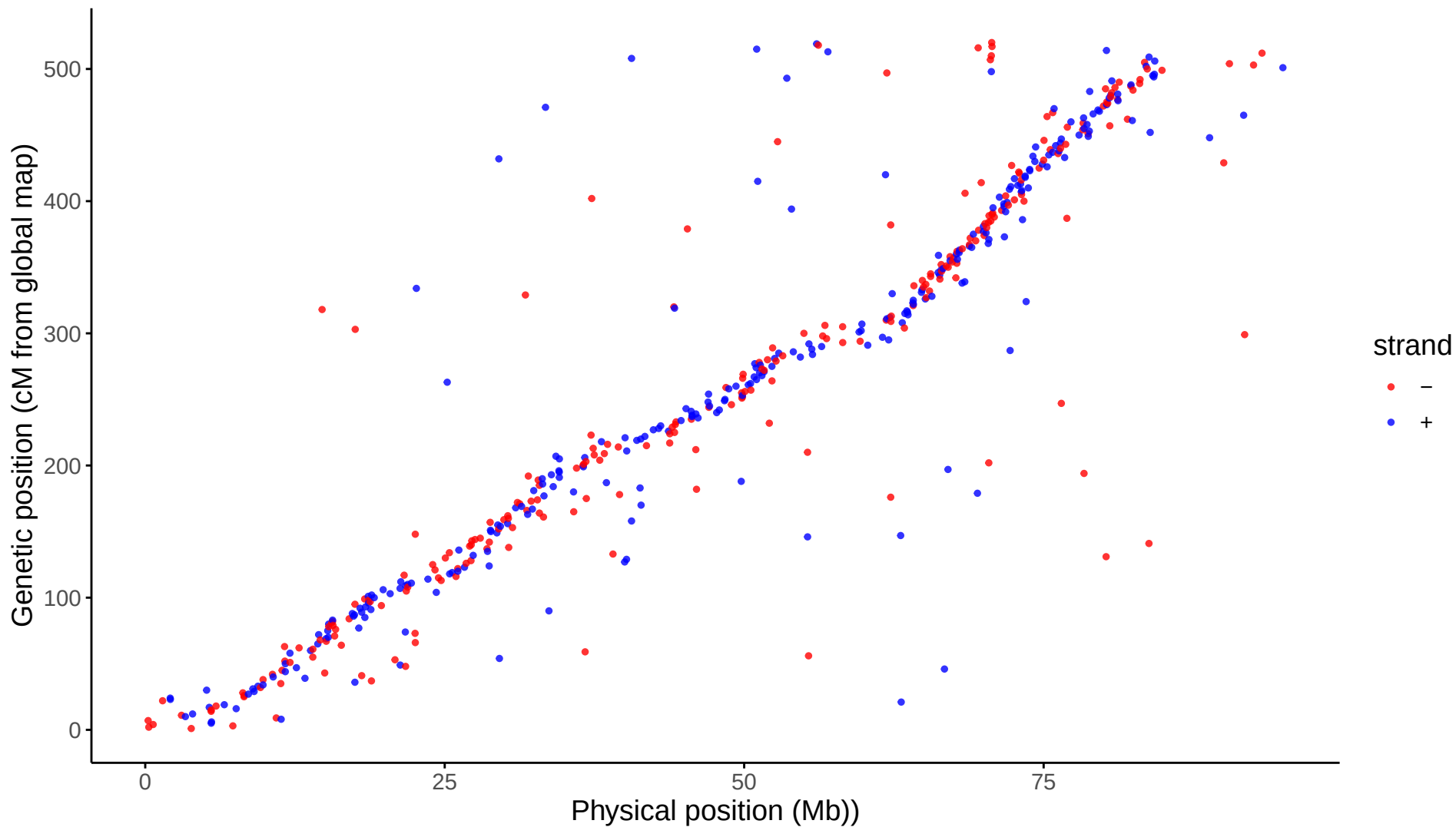
Global: LG12 markers aligned to Omy12
