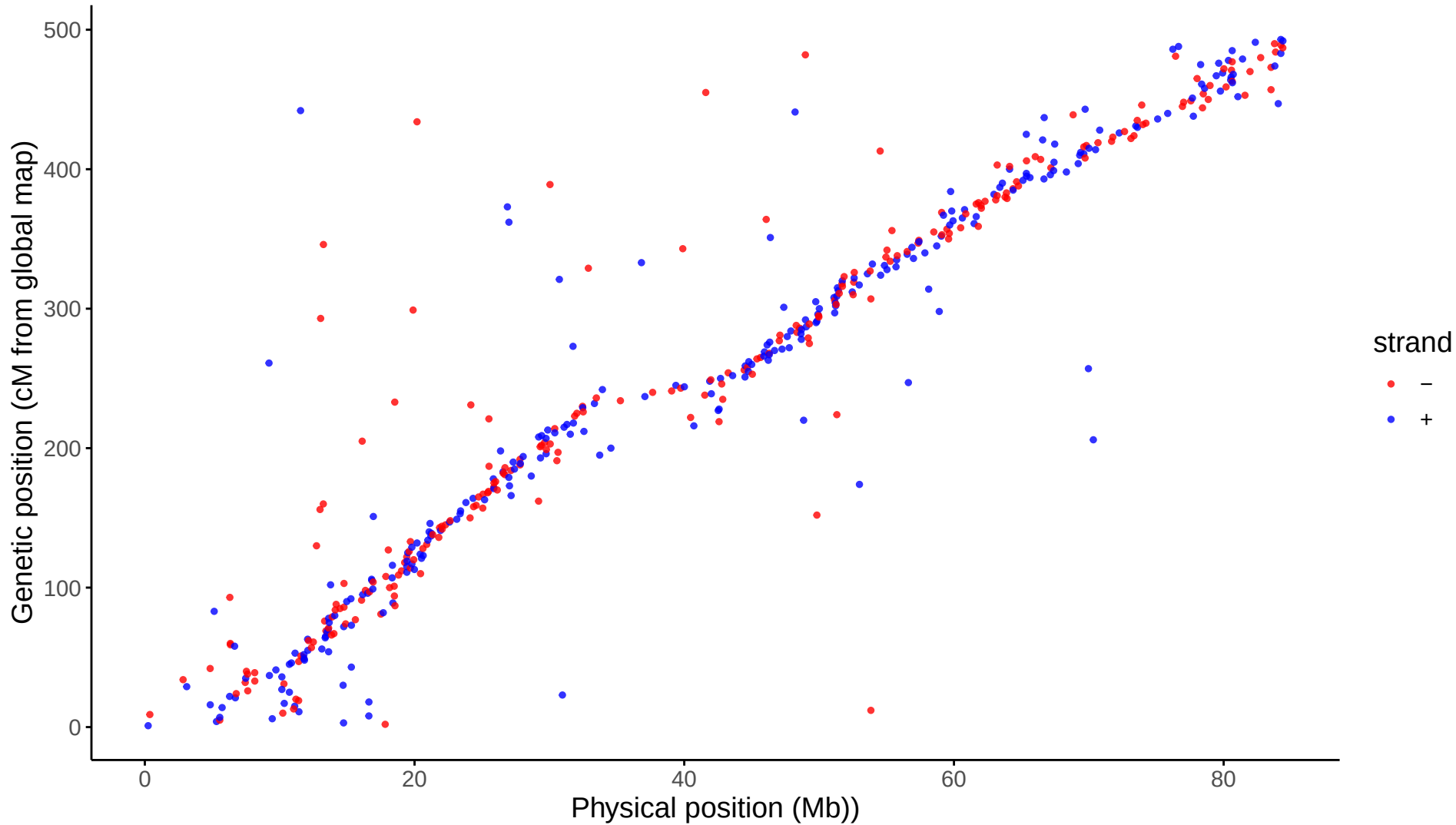
Global: LG03 markers aligned to Omy03
