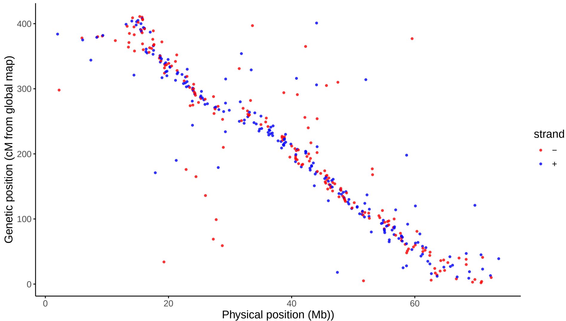
Global: LG18 markers aligned to Omy18
