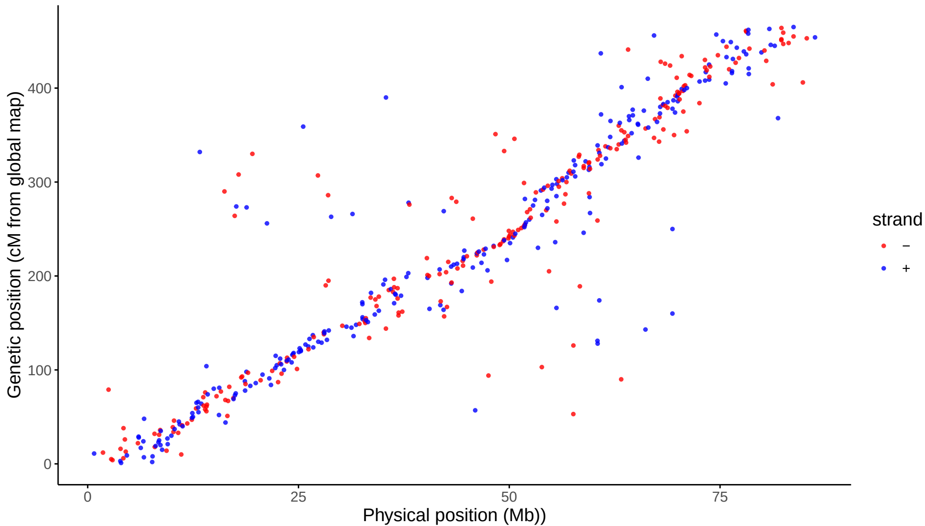
Global: LG11 markers aligned to Omy11
