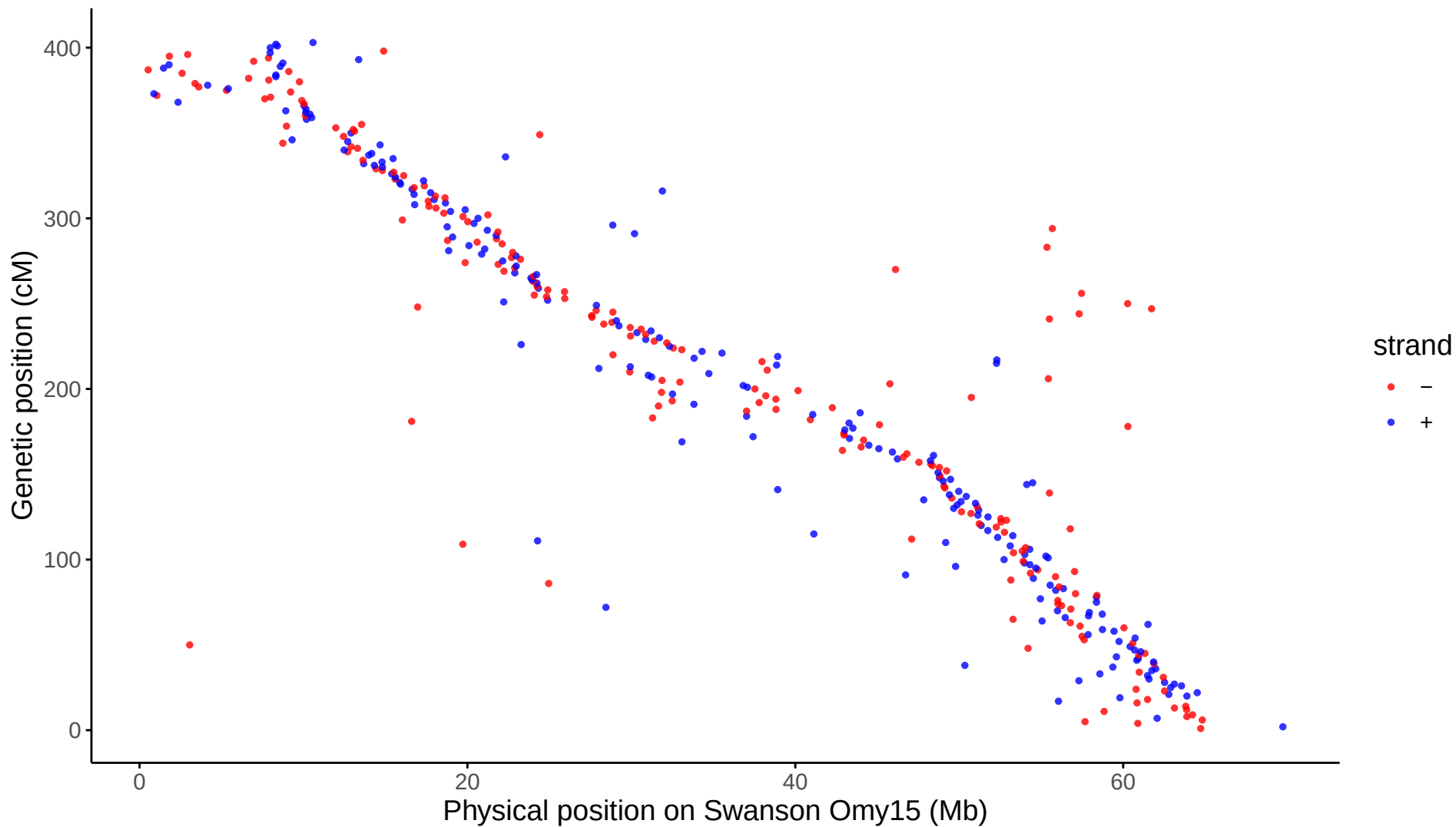
Global: LG15 aligned to Swanson Omy15
