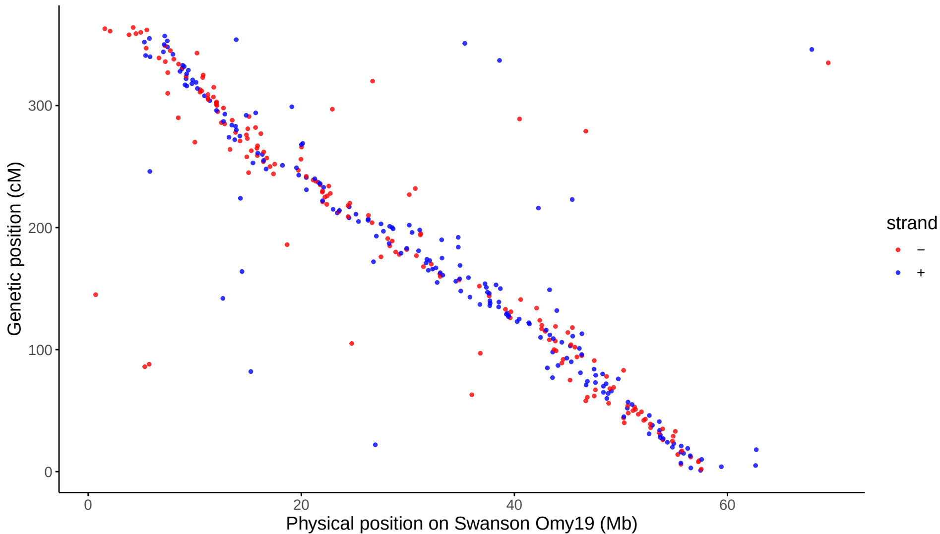
Global: LG19 aligned to Swanson Omy19
