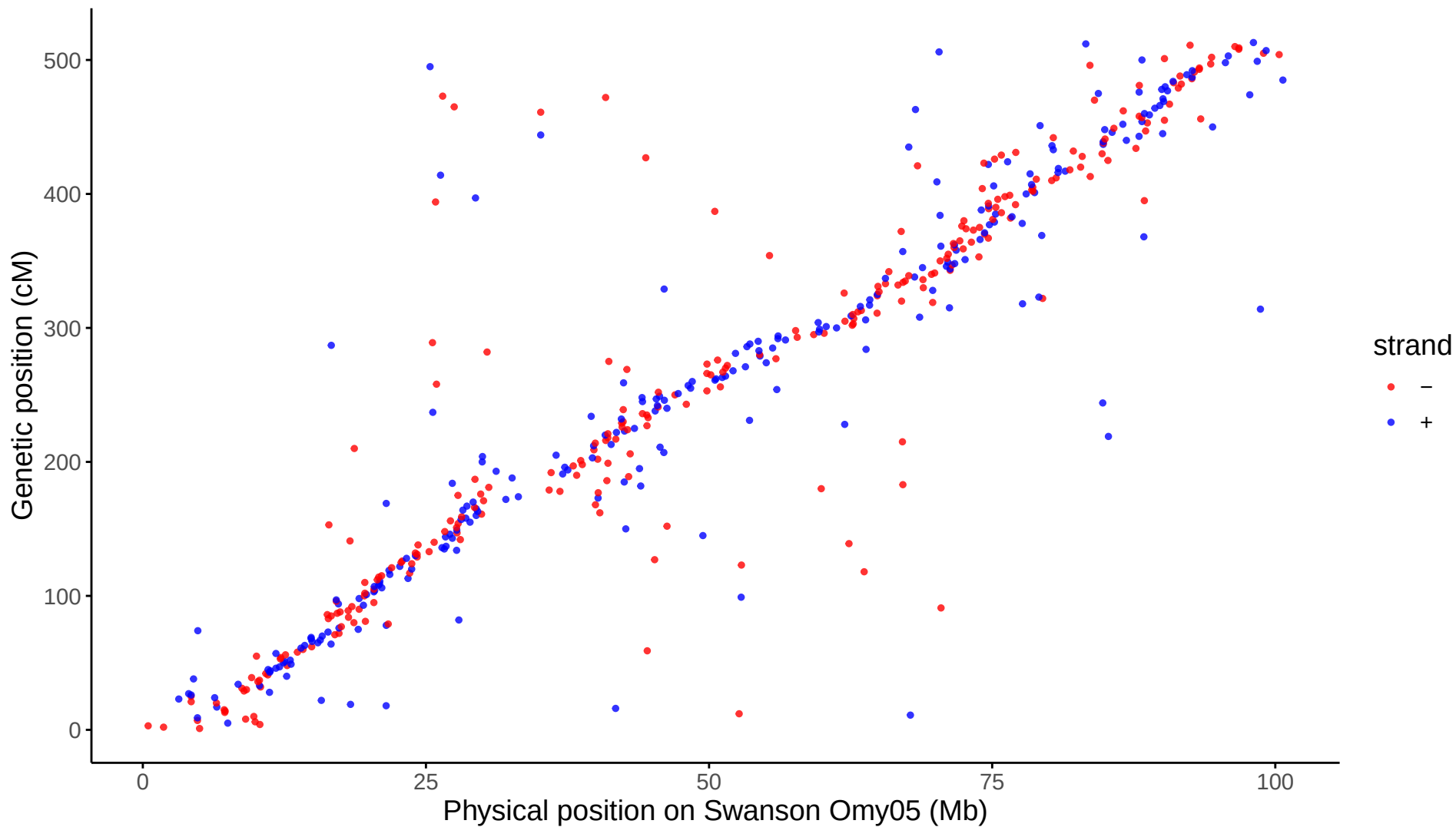
Global: LG05 aligned to Swanson Omy05
