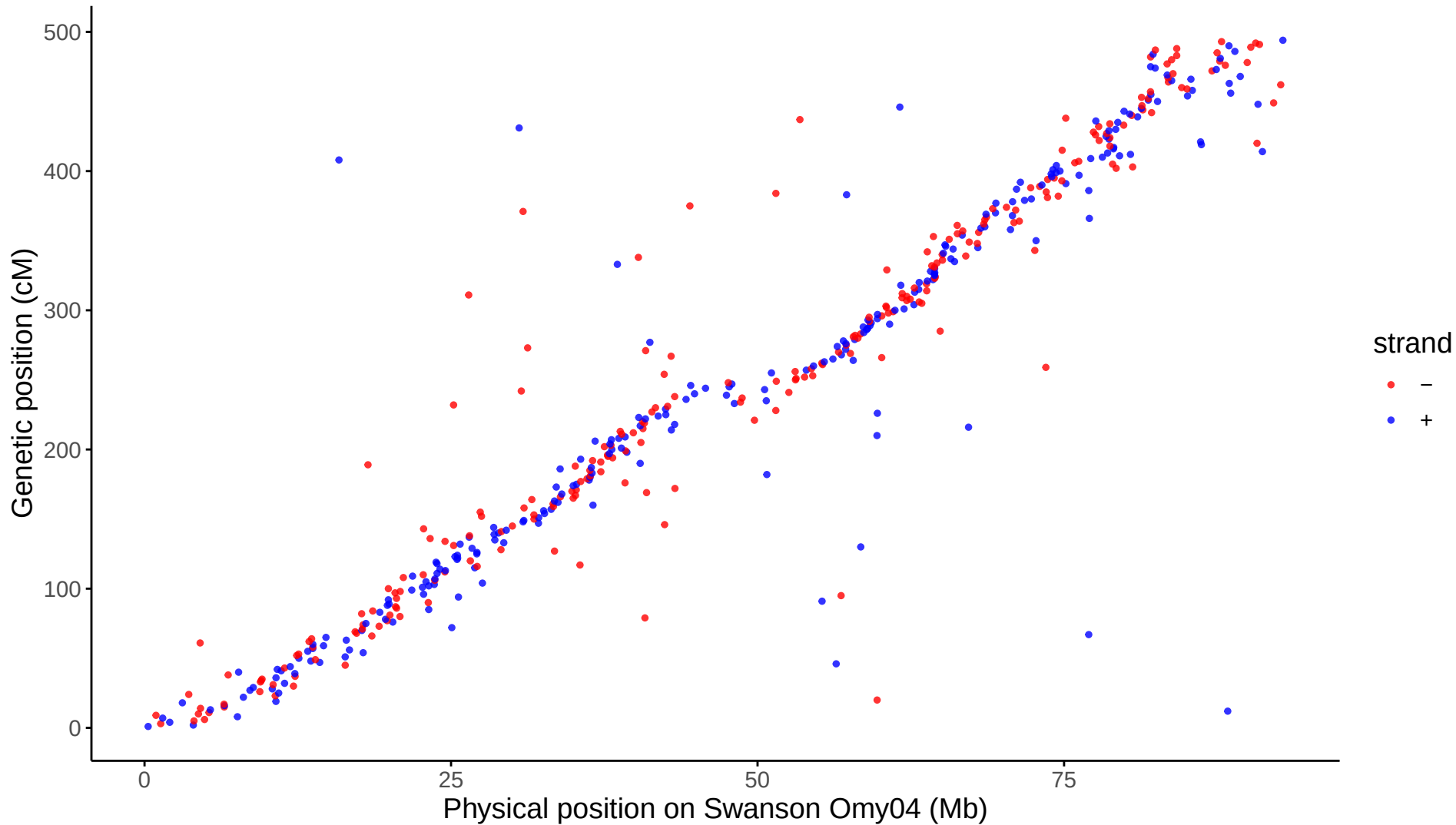
Global: LG04 aligned to Swanson Omy04
