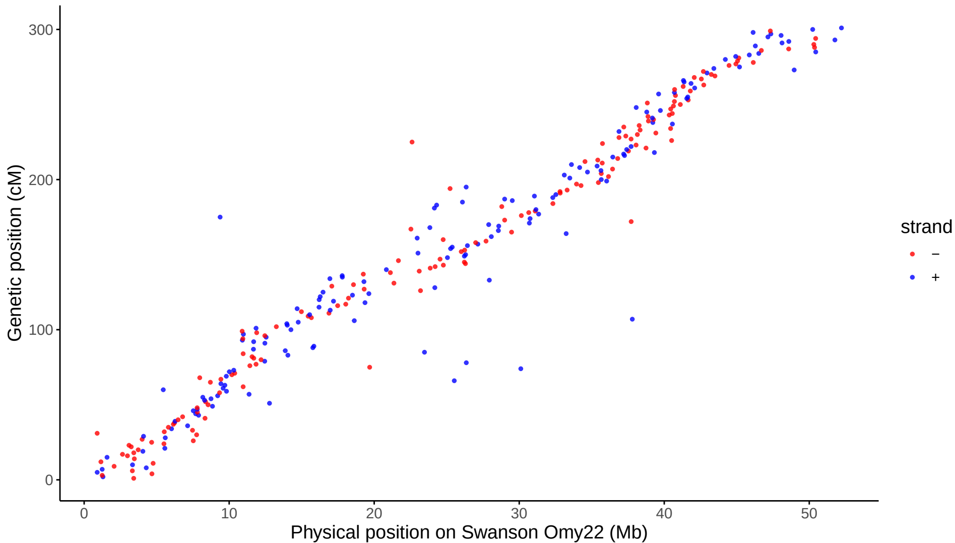
Global: LG22 aligned to Swanson Omy22
