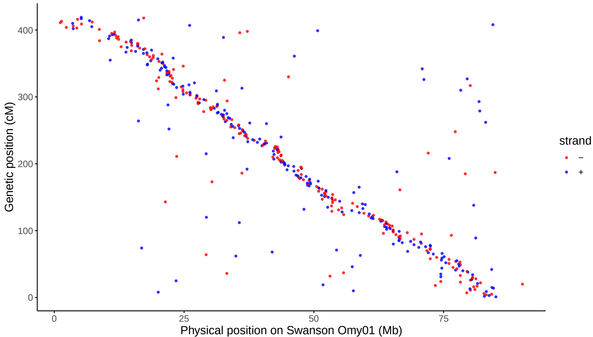
Global: LG01 aligned to Swanson Omy01
