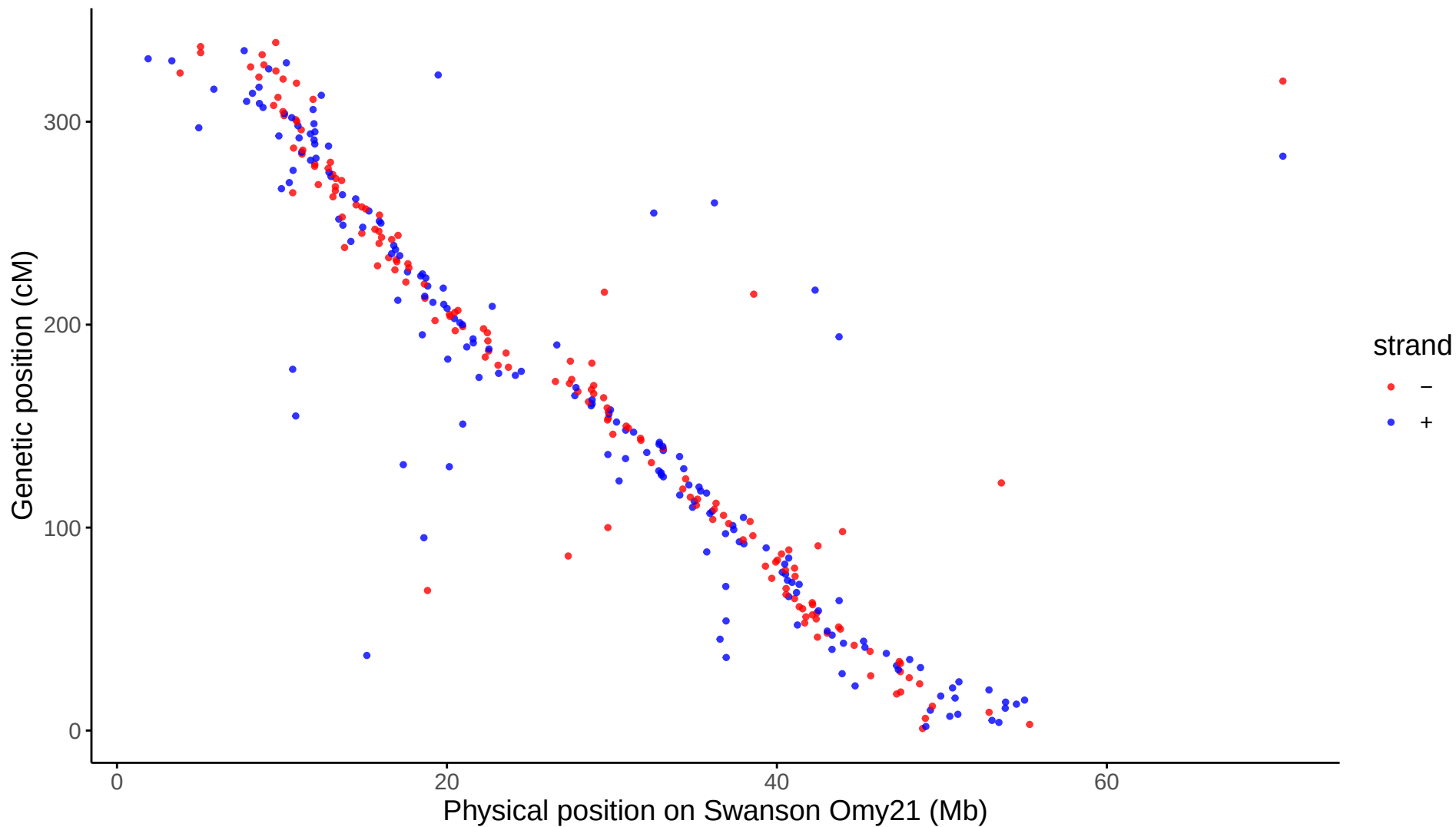
Global: LG21 aligned to Swanson Omy21
