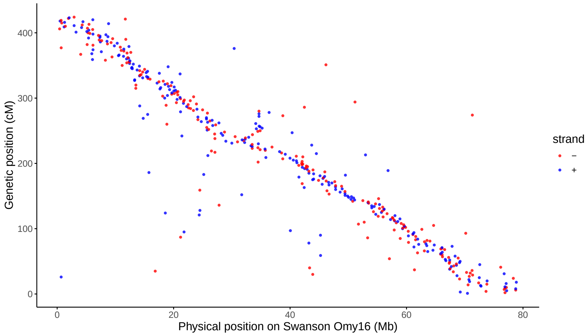
Global: LG16 aligned to Swanson Omy16
