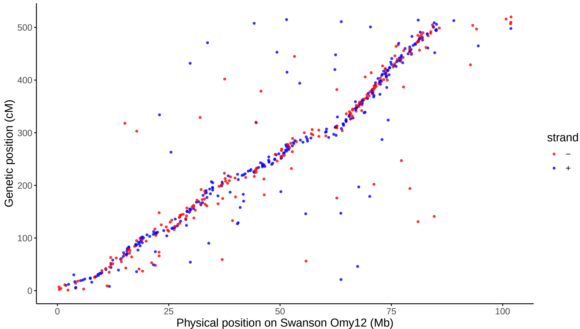
Global: LG12 aligned to Swanson Omy12
