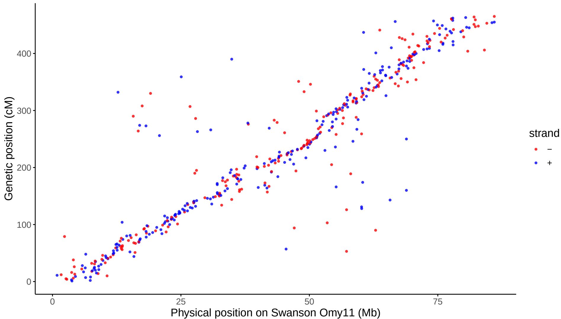
Global: LG11 aligned to Swanson Omy11
