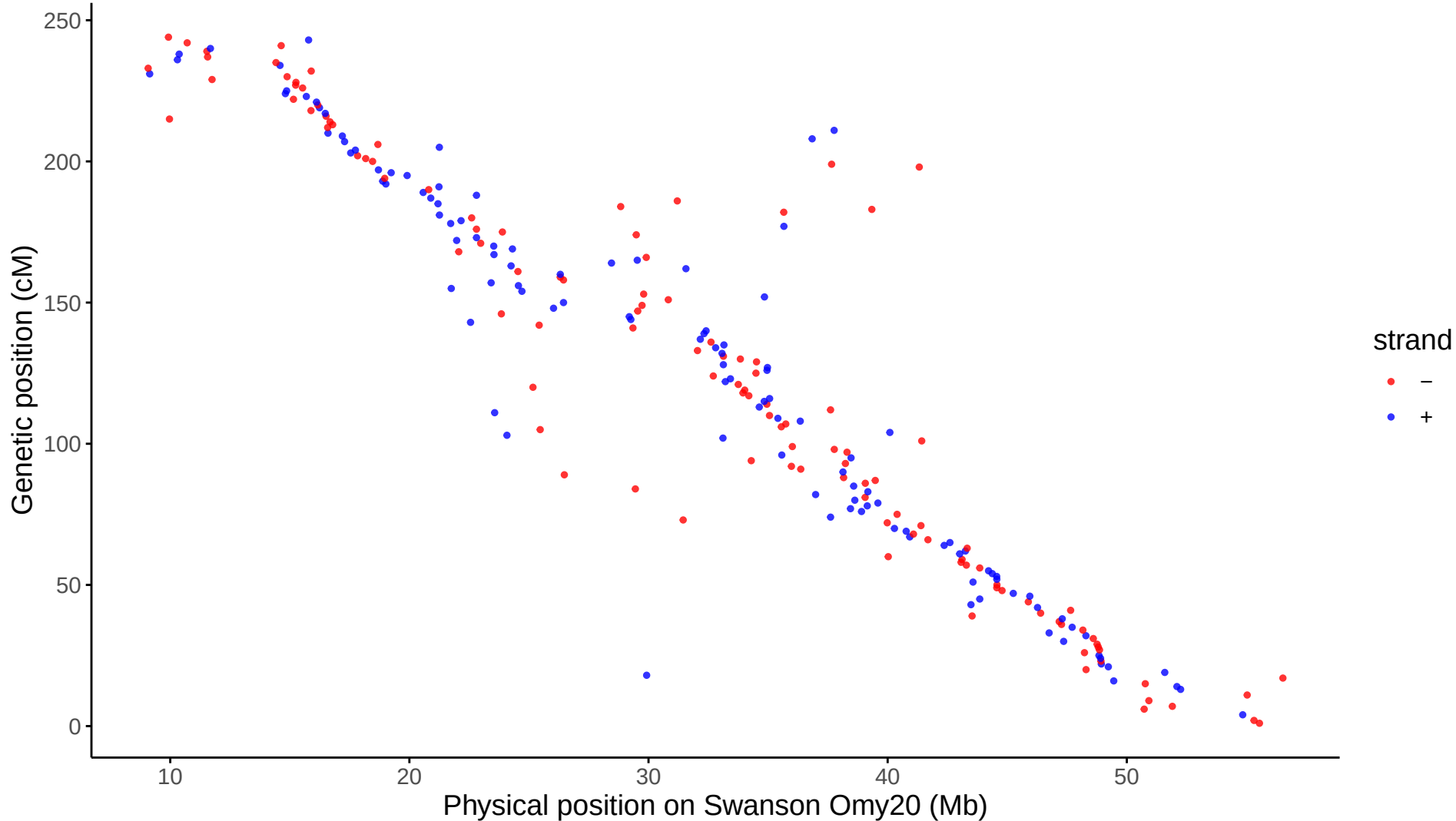
Global: LG20 aligned to Swanson Omy20
