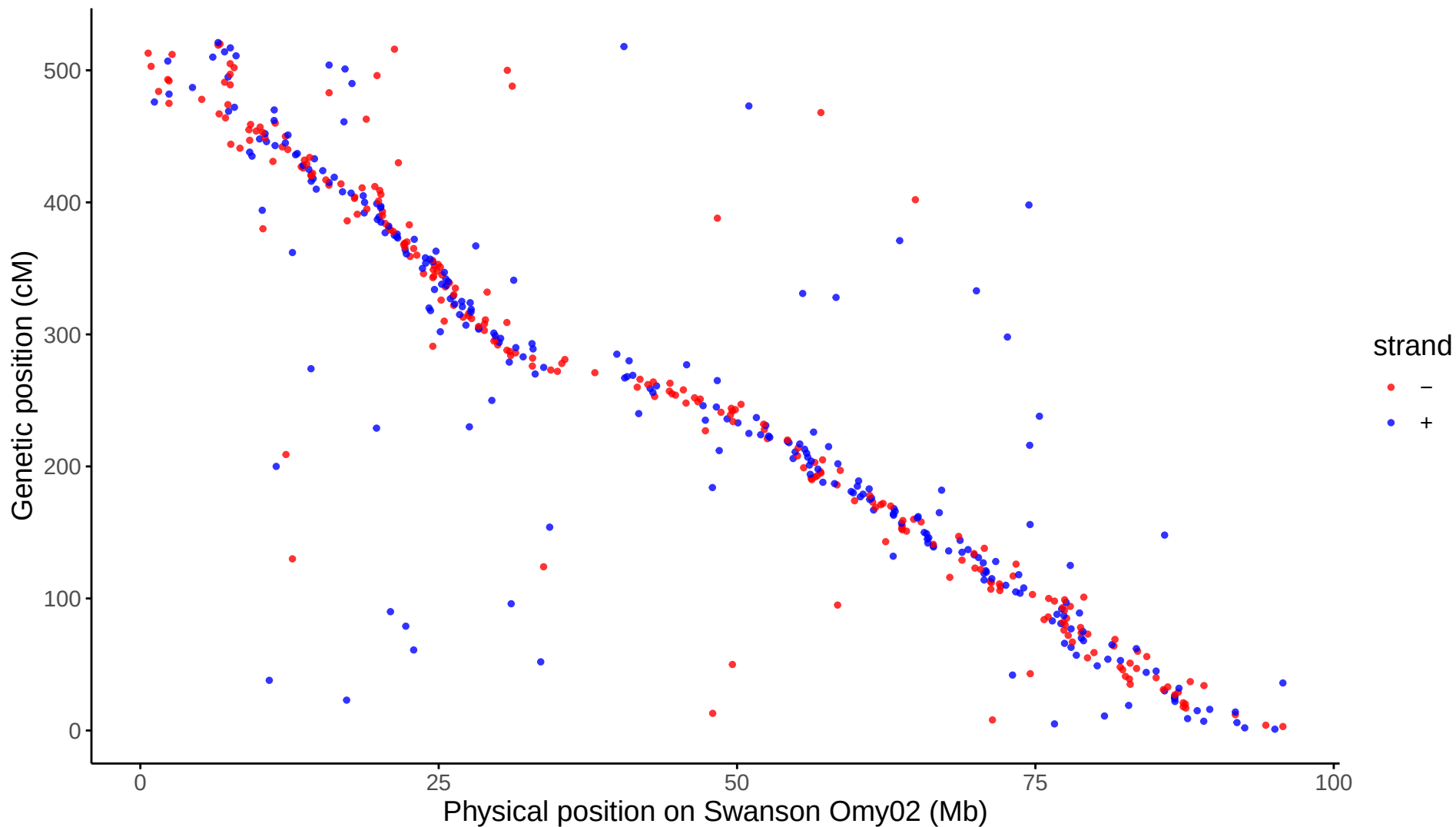
Global: LG02 aligned to Swanson Omy02
