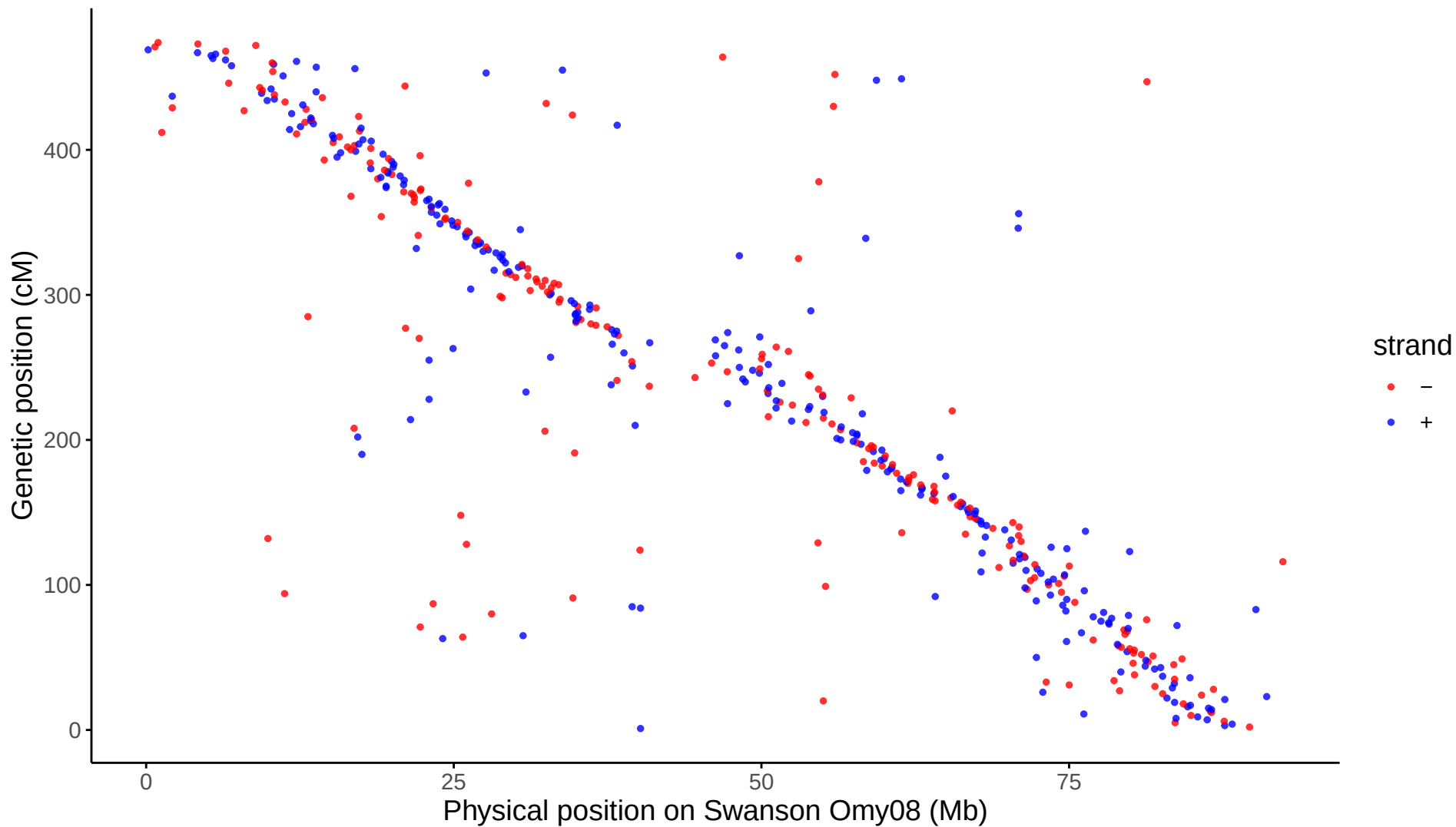
Global: LG08 aligned to Swanson Omy08
