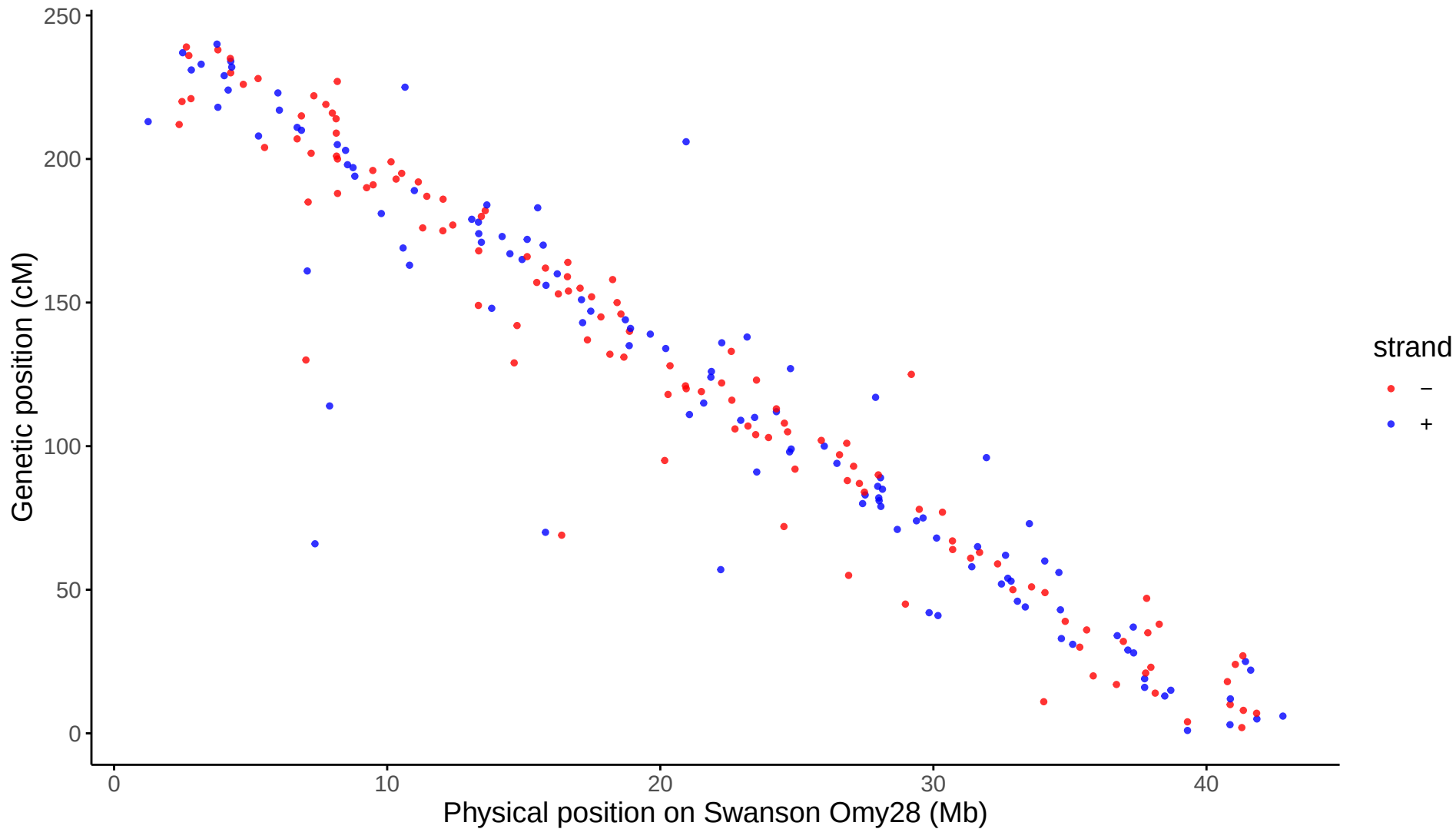
Global: LG28 aligned to Swanson Omy28
