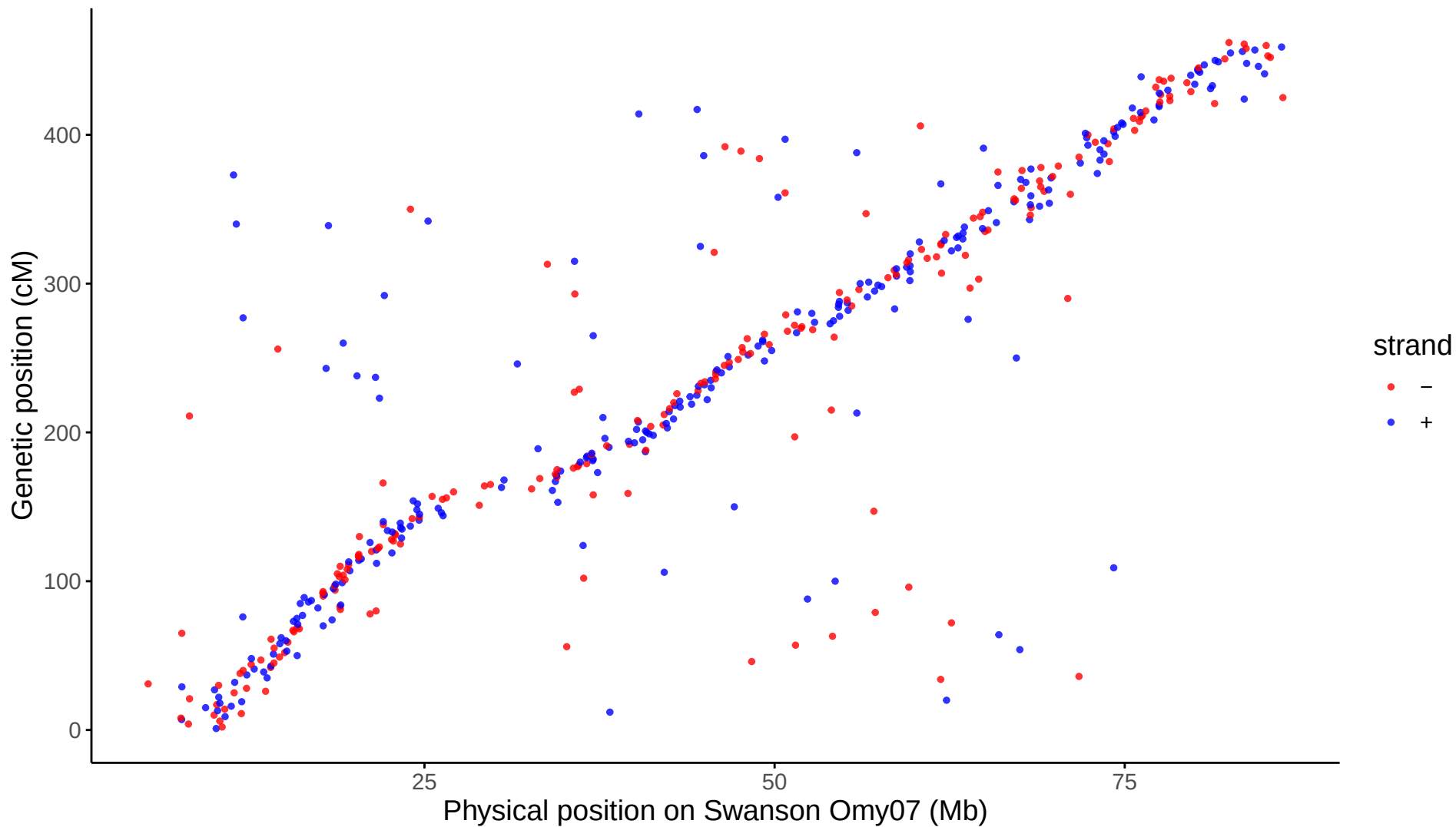
Global: LG07 aligned to Swanson Omy07
