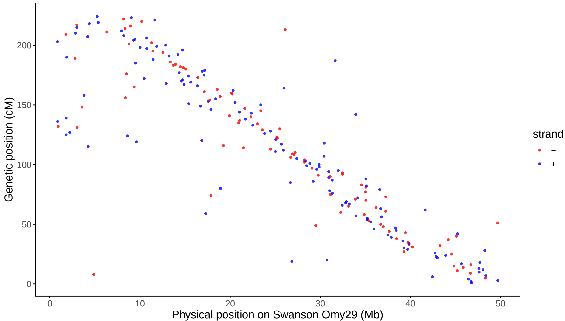
Global: LG29 aligned to Swanson Omy29
