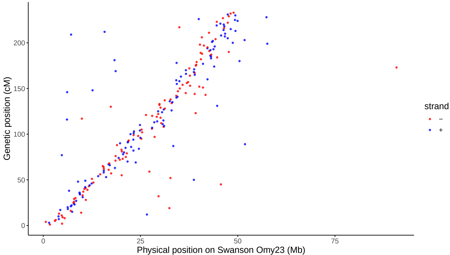
Global: LG23 aligned to Swanson Omy23
