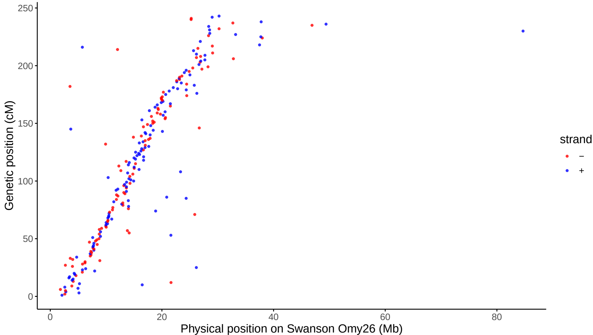
Global: LG26 aligned to Swanson Omy26
