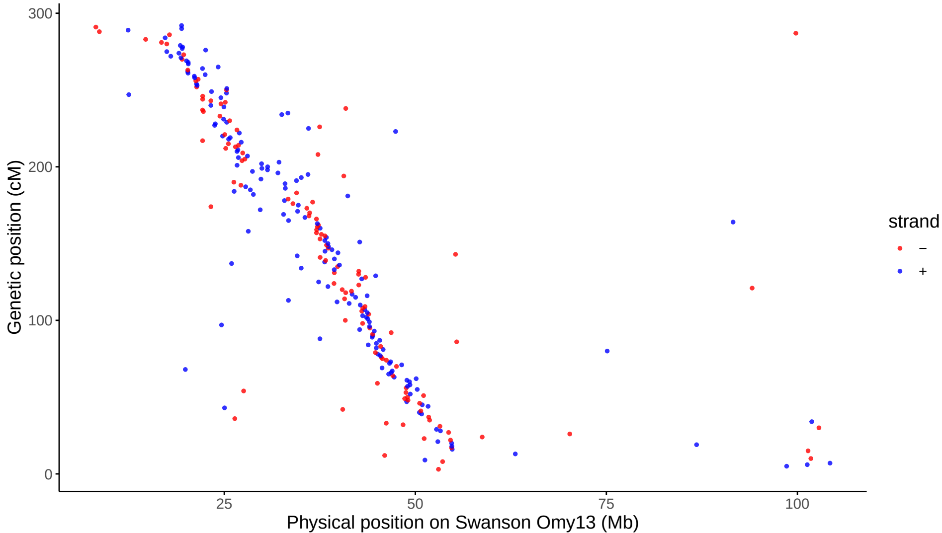
Global: LG13 aligned to Swanson Omy13
