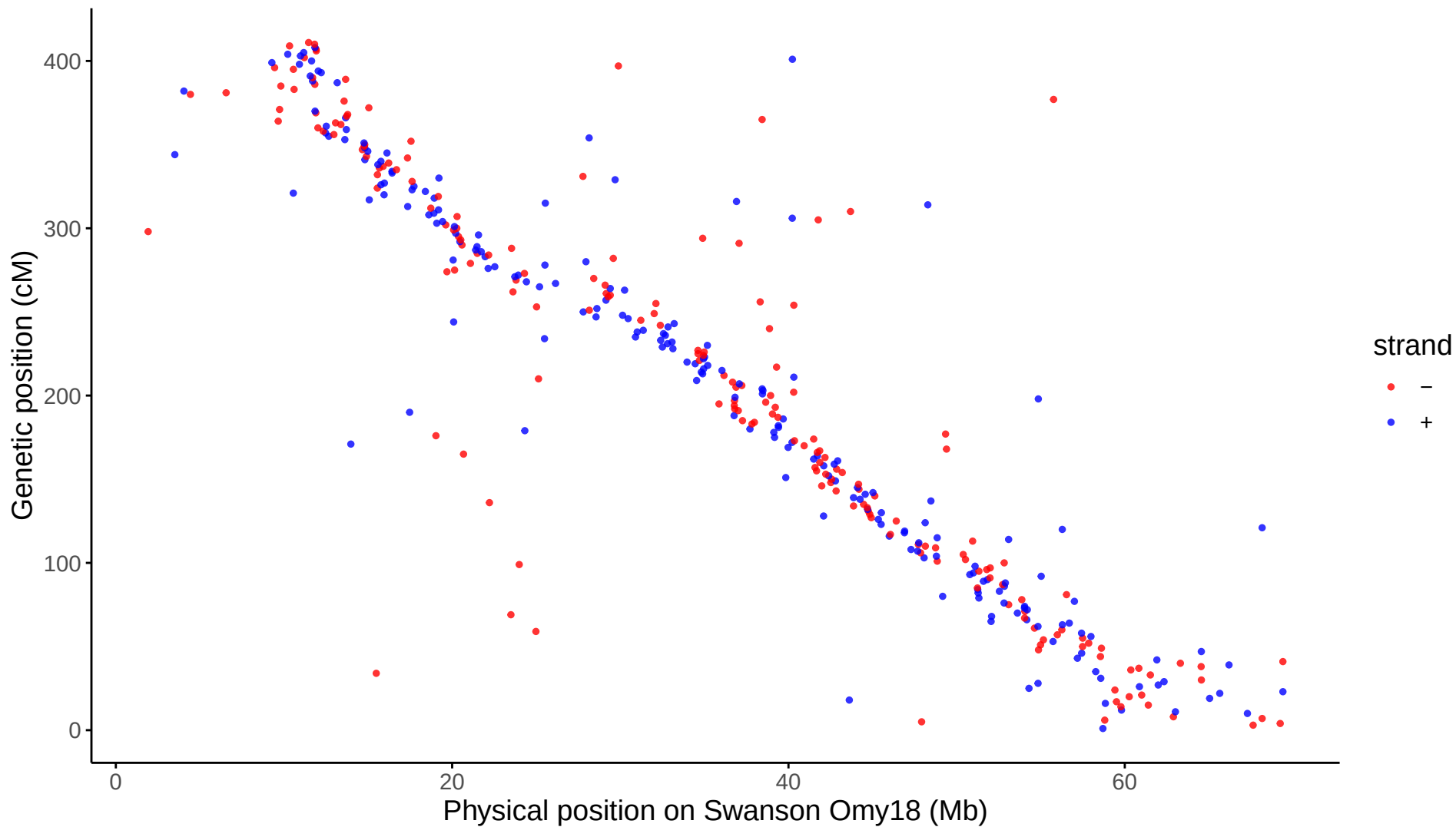
Global: LG18 aligned to Swanson Omy18
