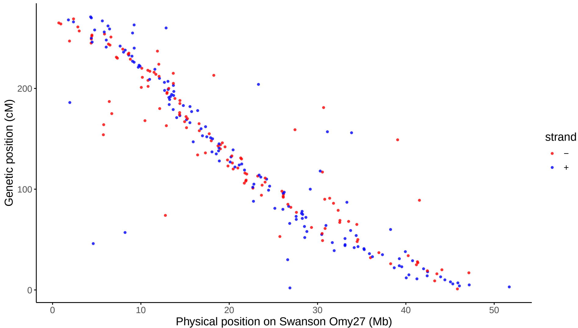
Global: LG27 aligned to Swanson Omy27
