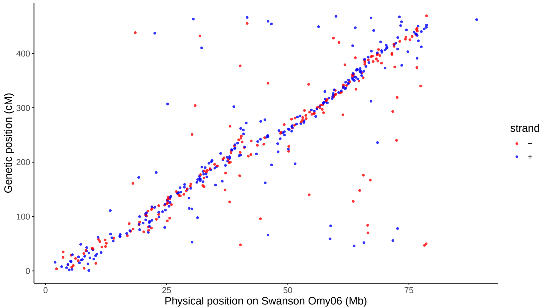
Global: LG06 aligned to Swanson Omy06
