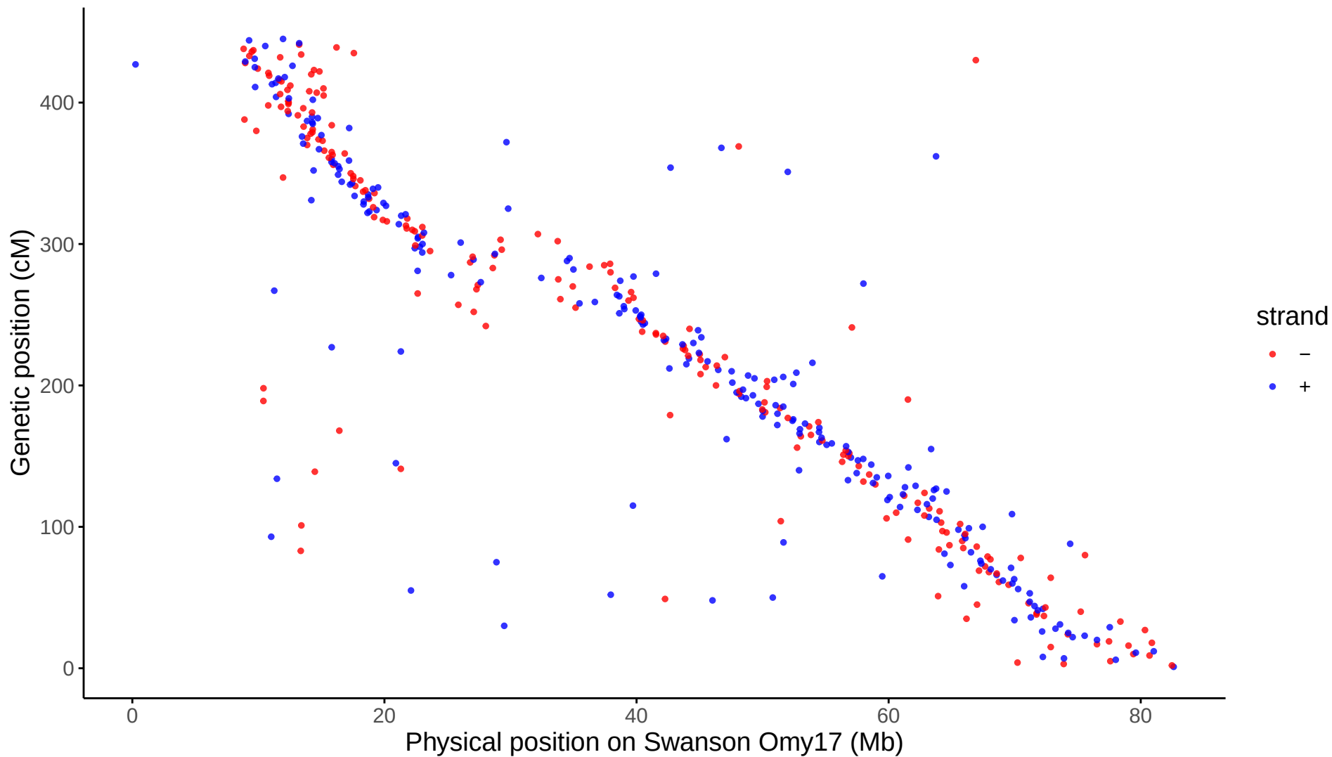
Global: LG17 aligned to Swanson Omy17
