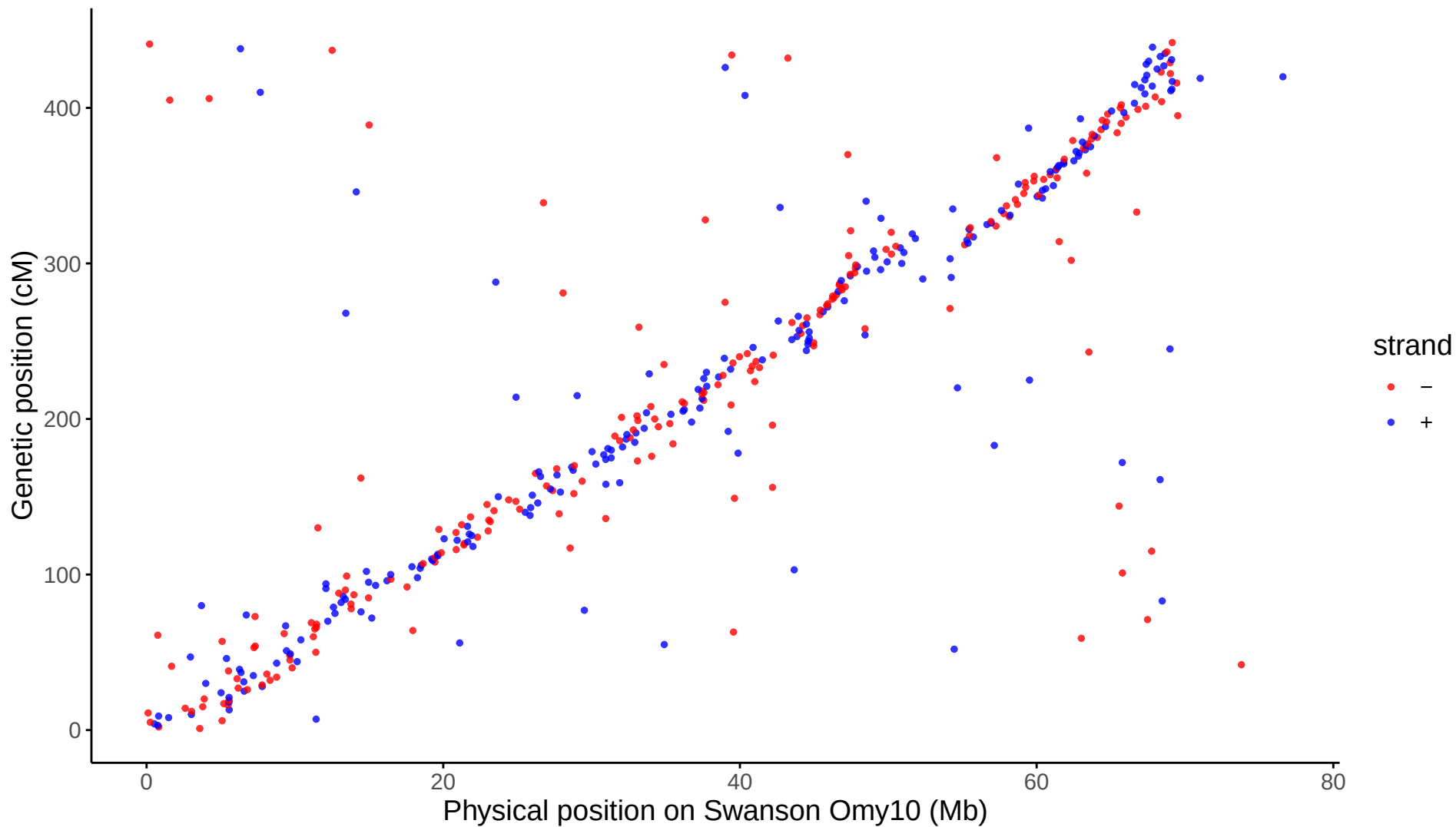
Global: LG10 aligned to Swanson Omy10
