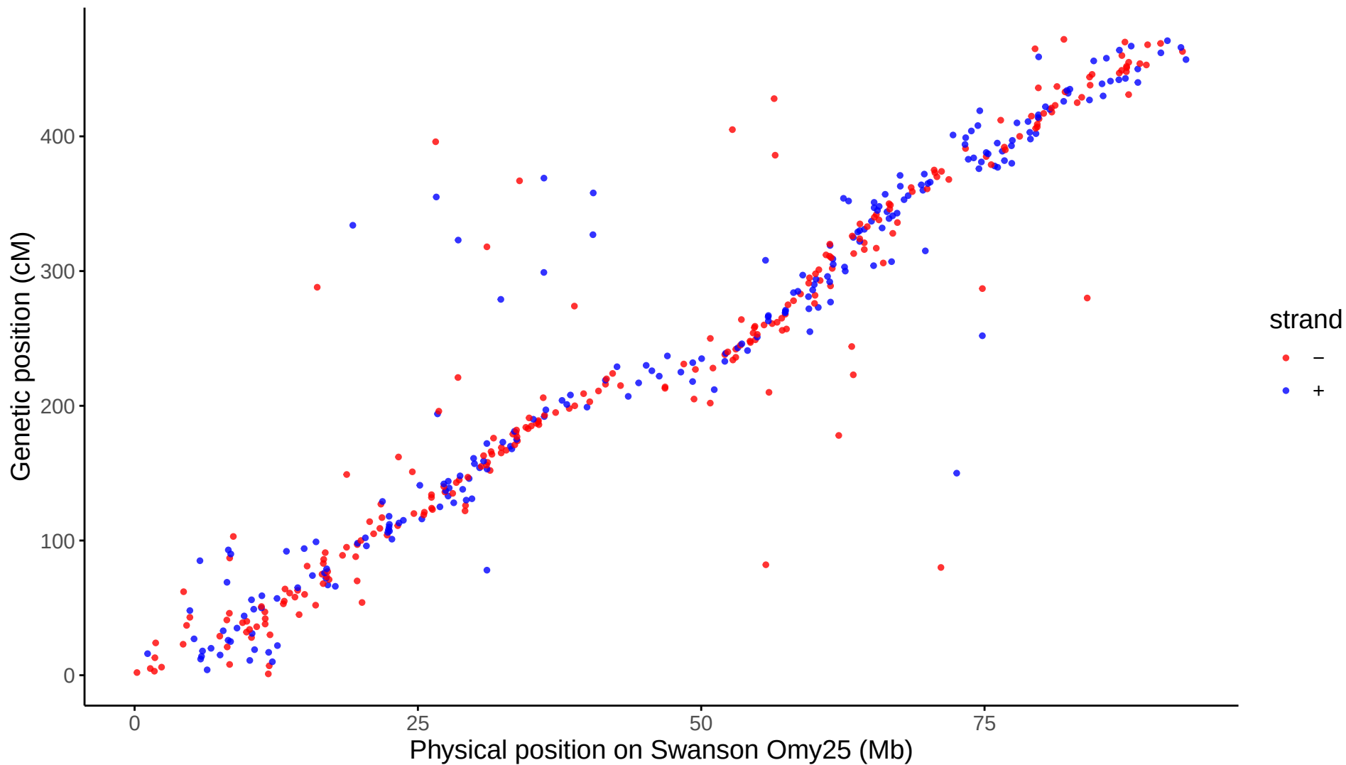
Global: LG25 aligned to Swanson Omy25
