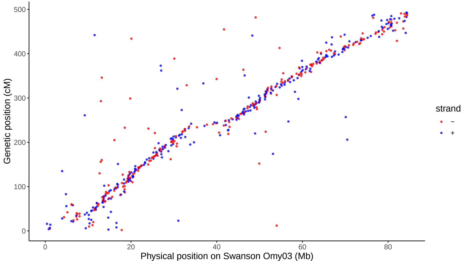
Global: LG03 aligned to Swanson Omy03
