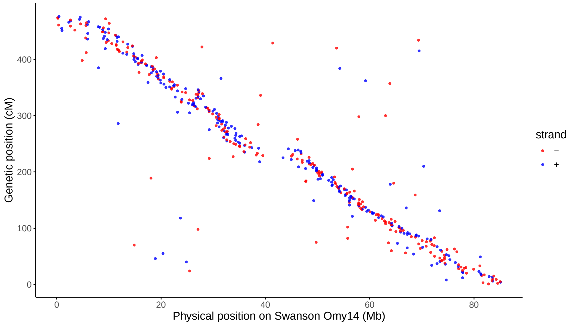
Global: LG14 aligned to Swanson Omy14
