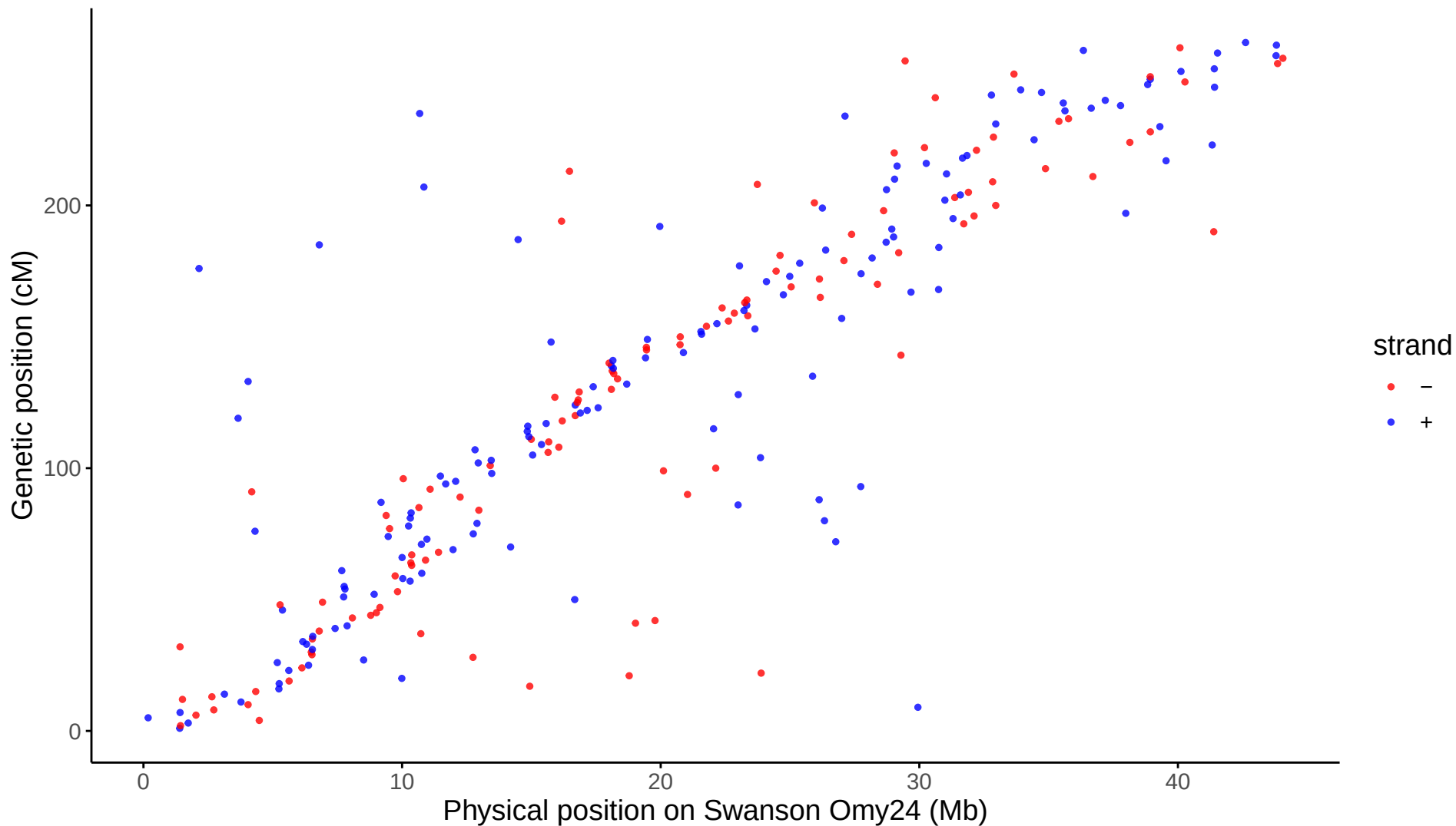
Global: LG24 aligned to Swanson Omy24
