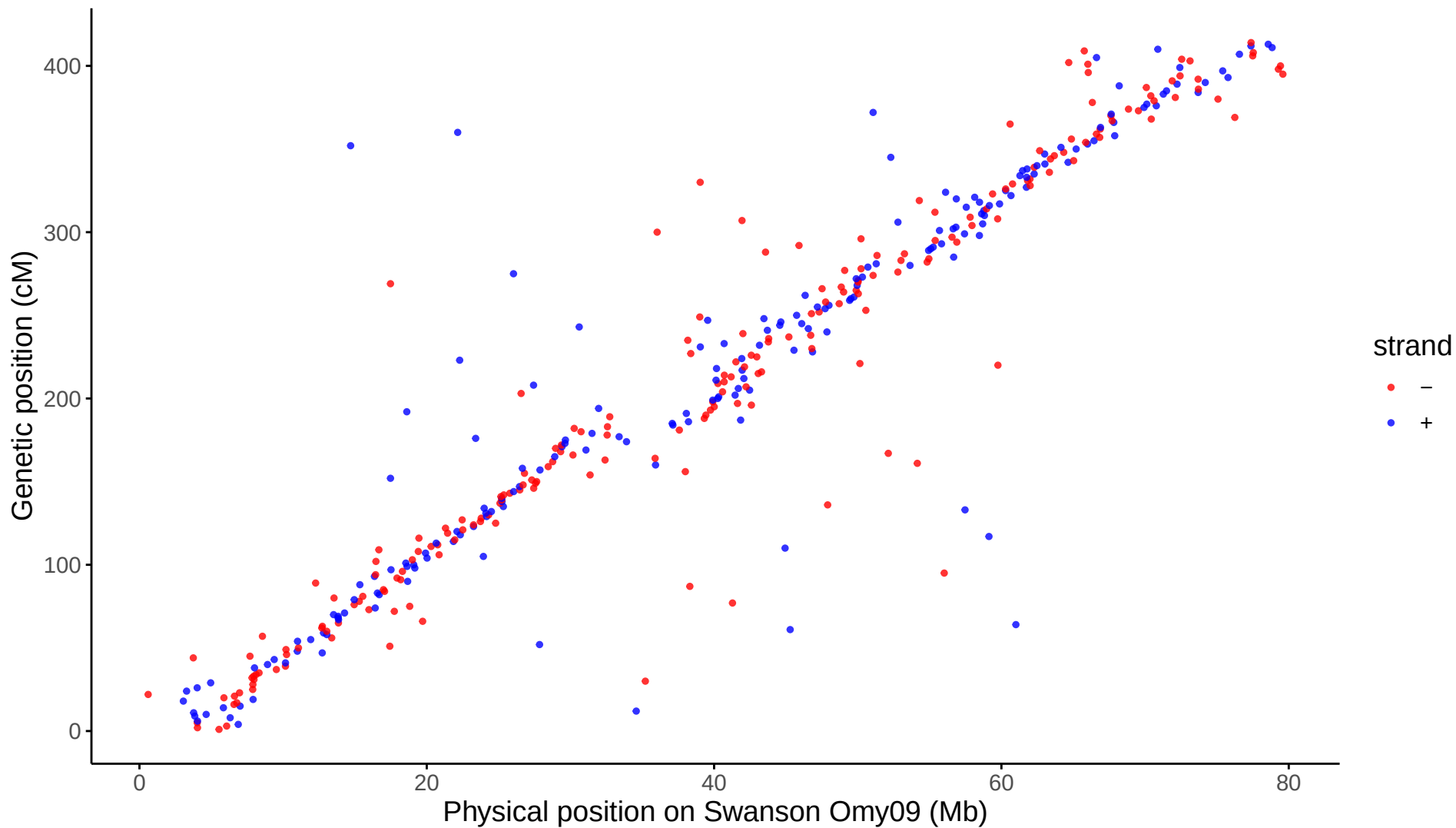
Global: LG09 aligned to Swanson Omy09
