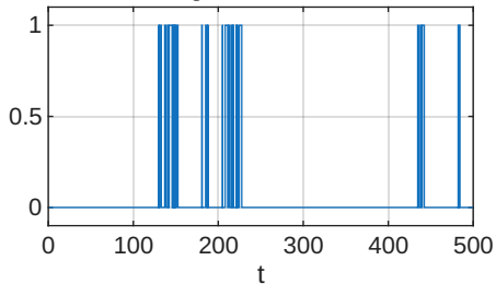
Queue isFull
