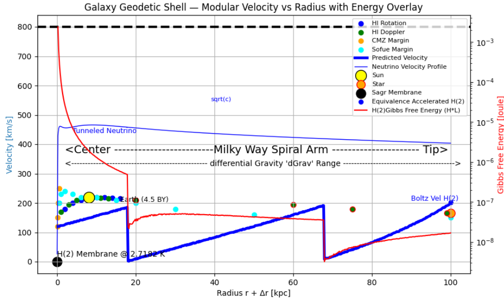
Figure 1 — Galaxy Geodetic Shell: Modular Velocity vs Radius with Energy Overlay
