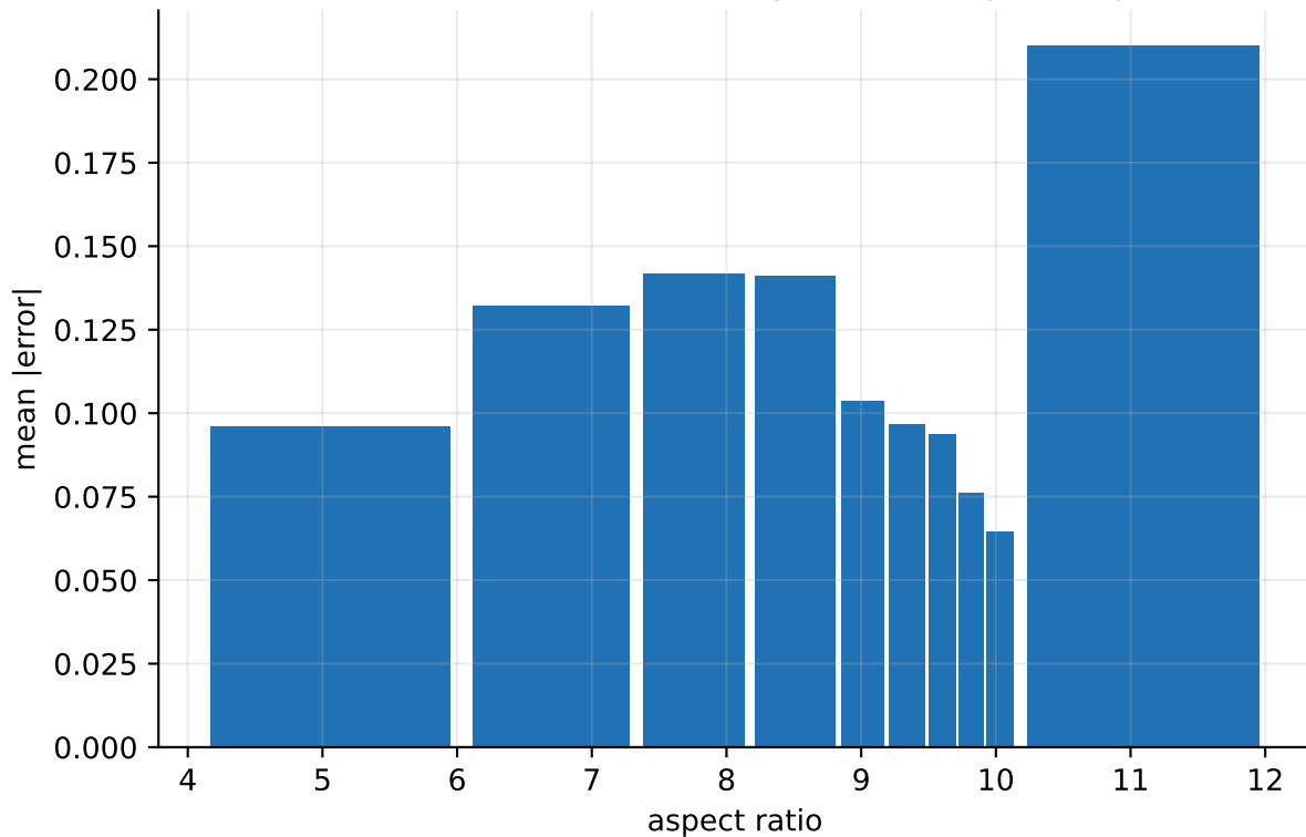
Prediction error tracks data density, before any surrogate exists
