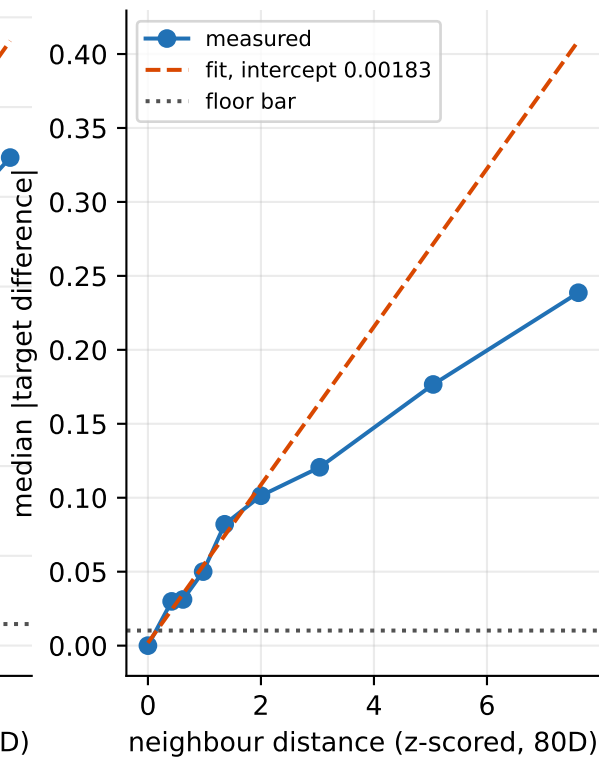
Near-identical shapes carry near-identical answers edge_rot_transform AT FLOOR log10_qf AT FLOOR
