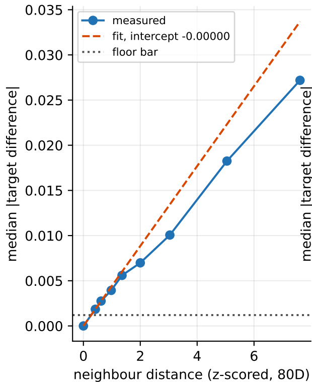
Near-identical shapes carry near-identical answers edge_rot_transform AT FLOOR log10_qf AT FLOOR
