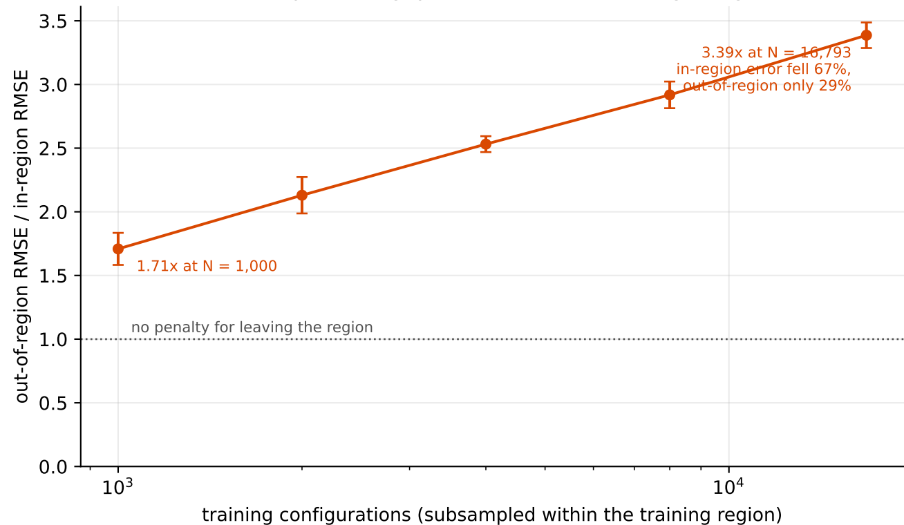
The extrapolation gap widens as the training set grows
