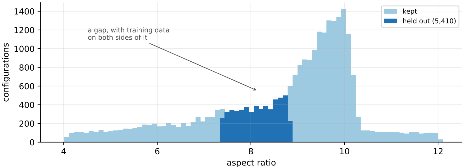
Hole: hold out a band at percentiles 20 to 40
