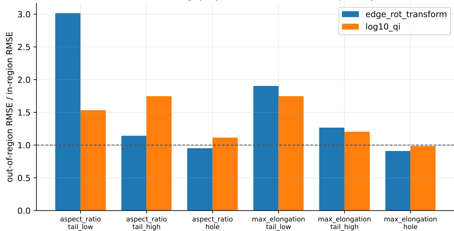
Generalization gap by axis and cut (1.0 = no penalty)
