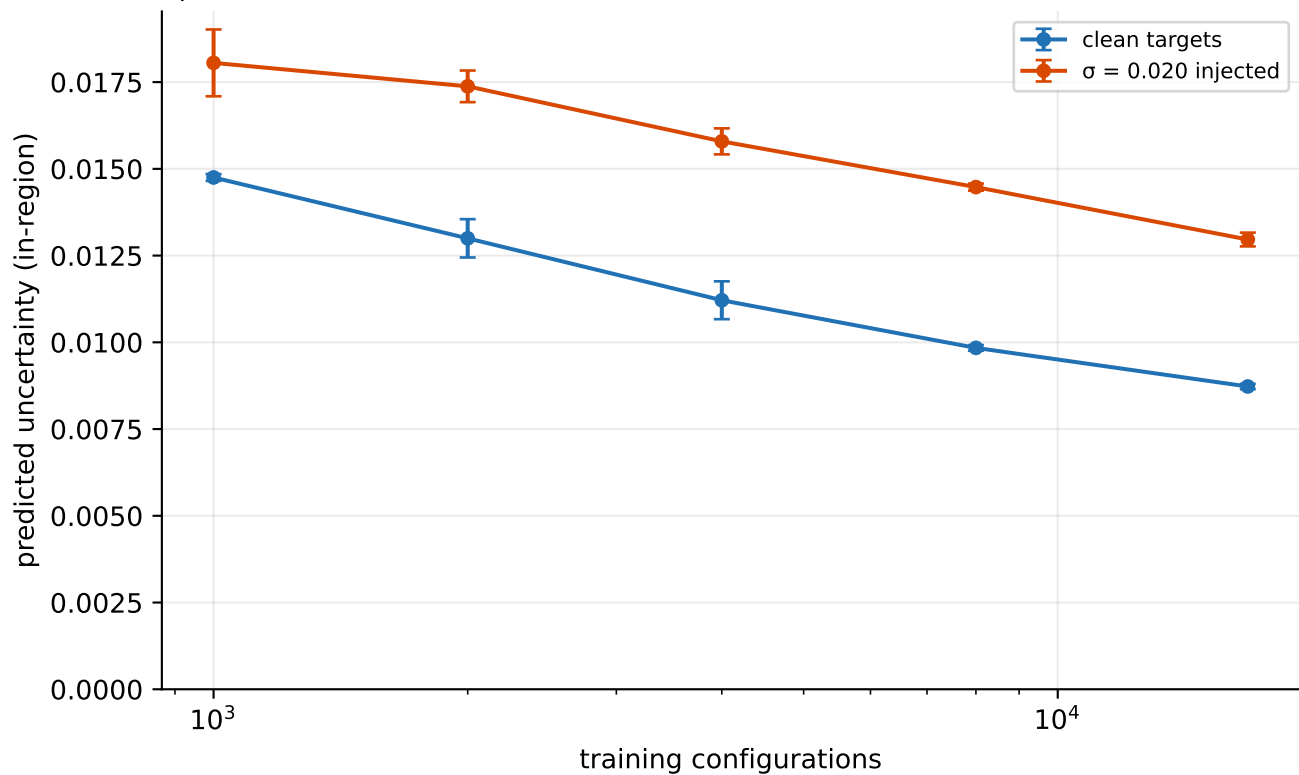
Epistemic shrinks with data
