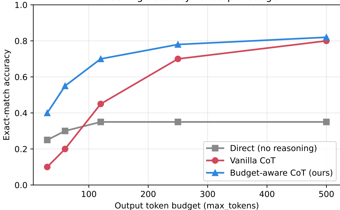
Reasoning accuracy vs. output budget
