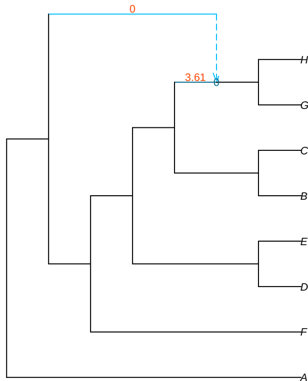
support for sister-hybrid relationships H1: st_1.0
