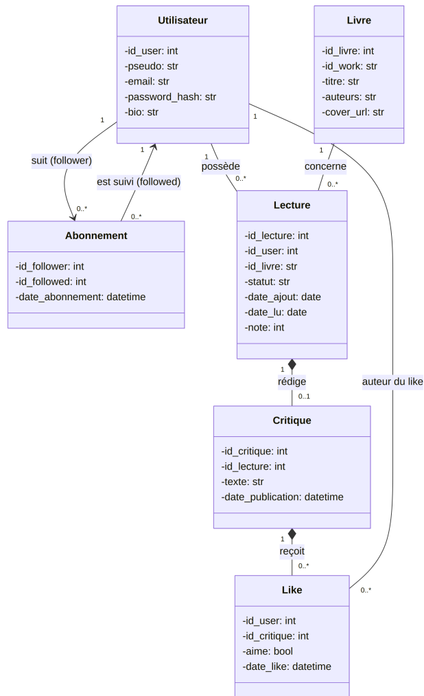
Figure 2: Diagramme de classes : Business Object
