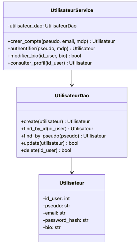
Figure 10: Diagramme de classes : authentication
