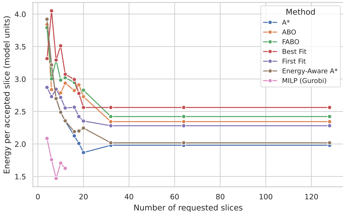
Energy efficiency vs load — 3 VNFs per slice
