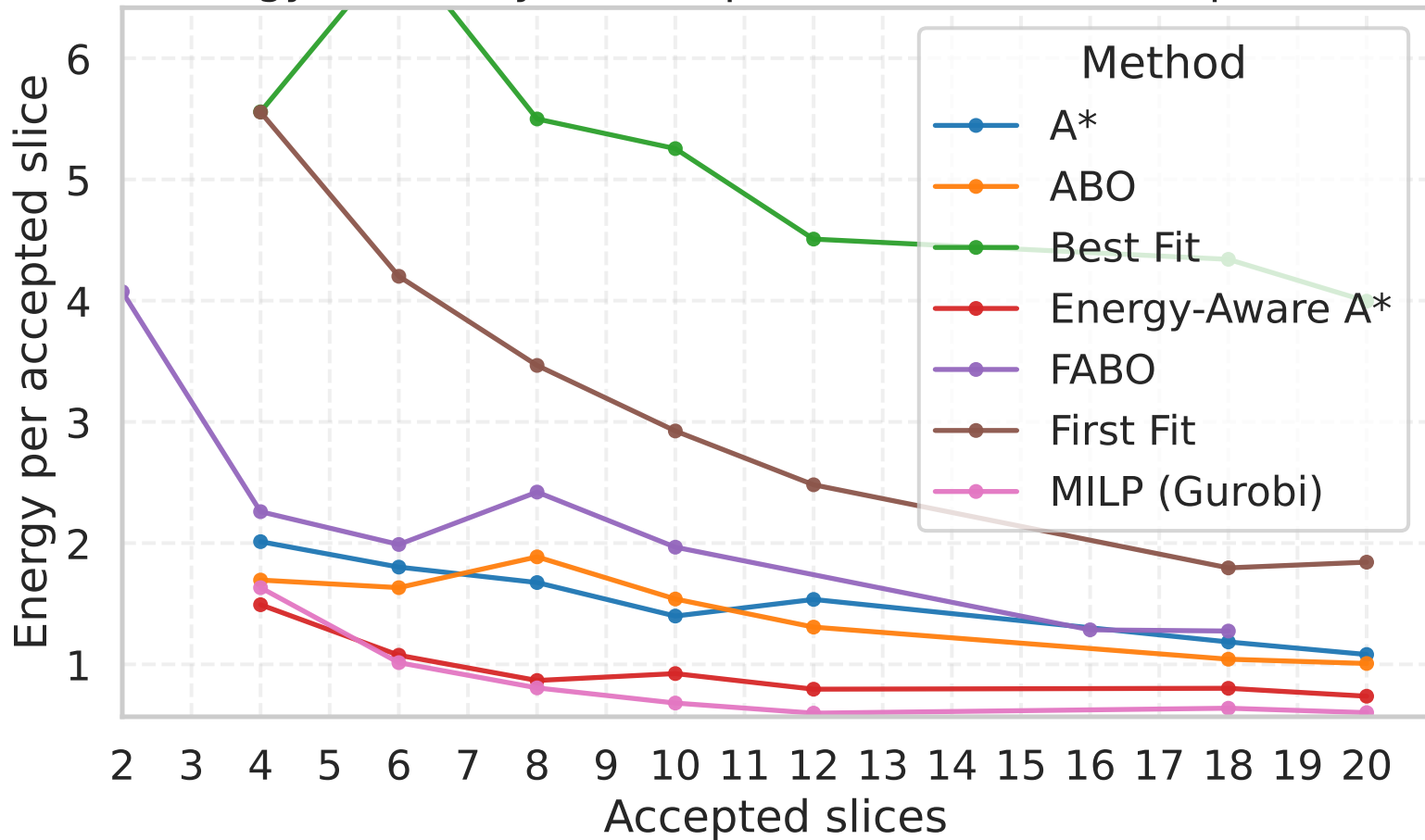
Energy Efficiency vs Accepted Slices — 3 VNFs per slice
