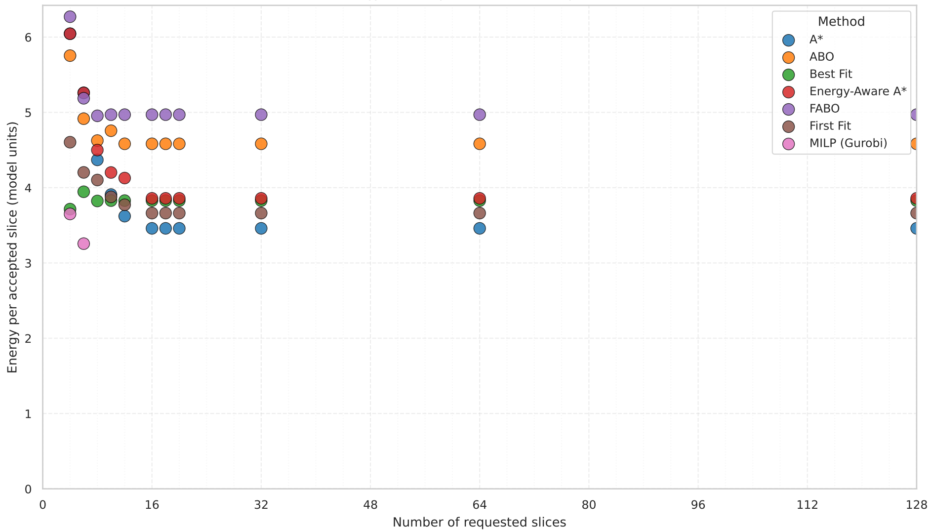
Energy Efficiency vs Load — 4 VNFs per slice
