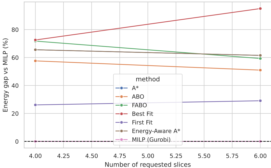
Energy optimality gap — 4 VNFs per slice
