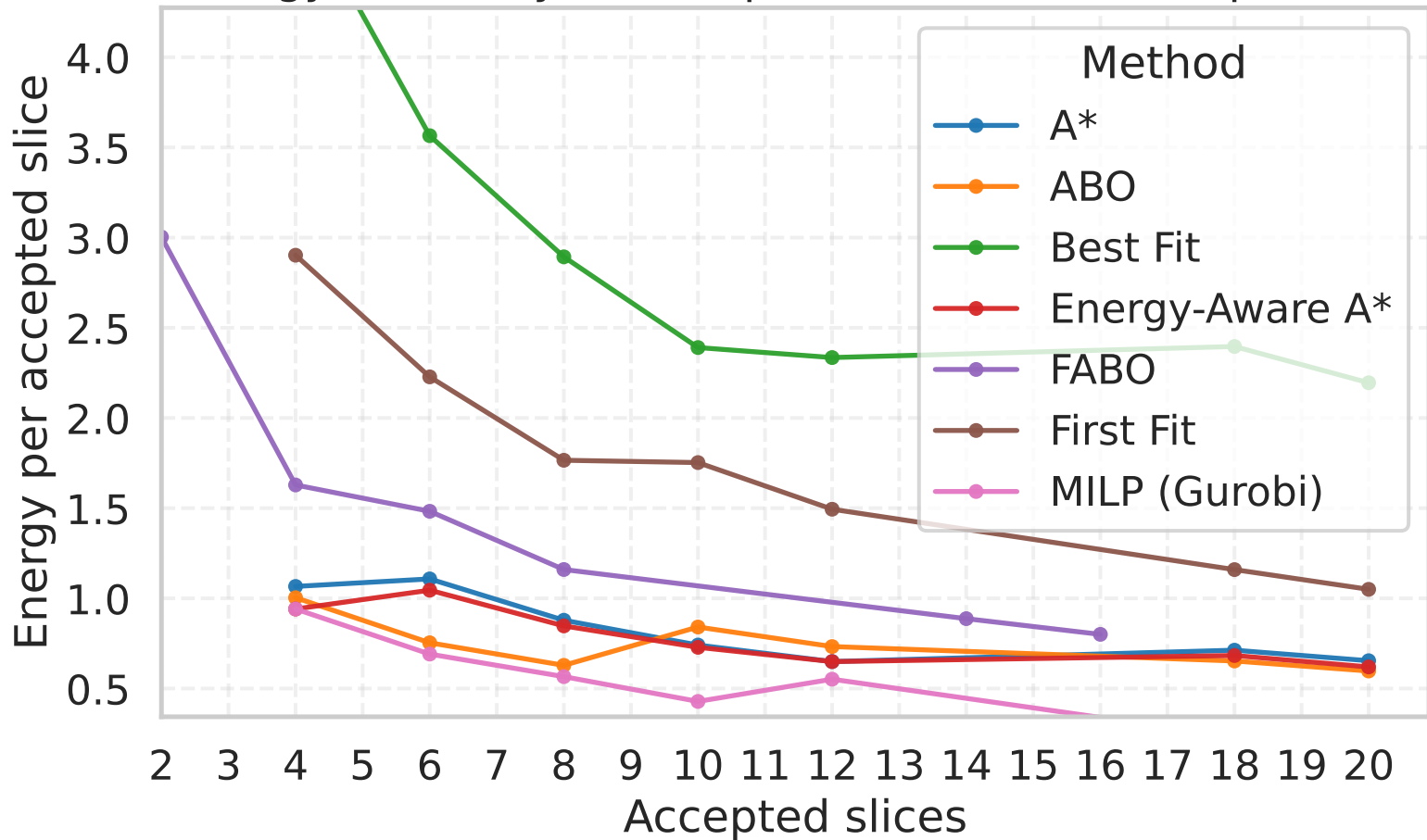
Energy Efficiency vs Accepted Slices — 2 VNFs per slice
