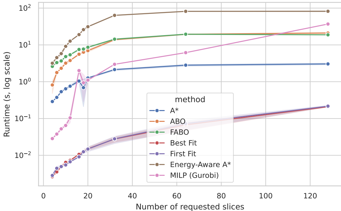
Runtime vs load — 4 VNFs per slice
