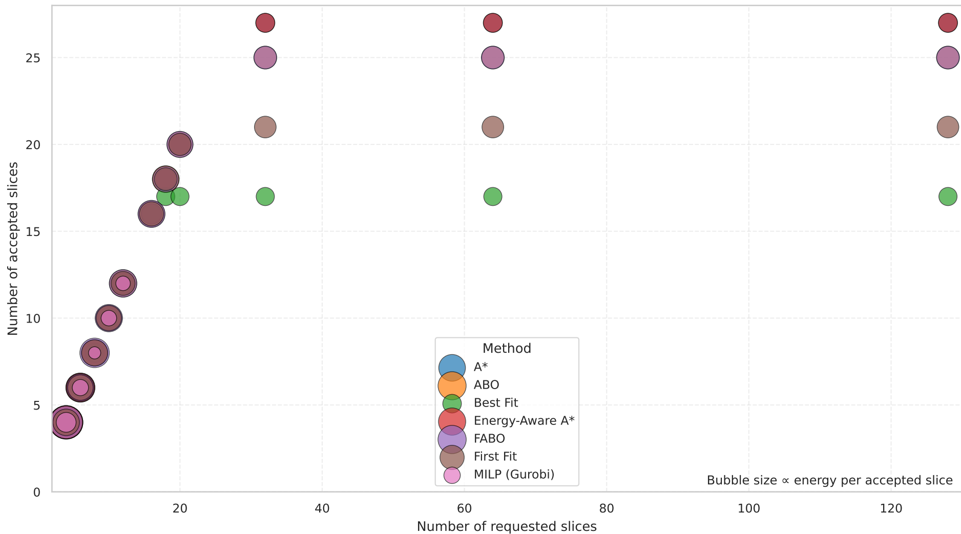
Bubble plot — Energy per accepted slice (size) 3 VNFs per slice
