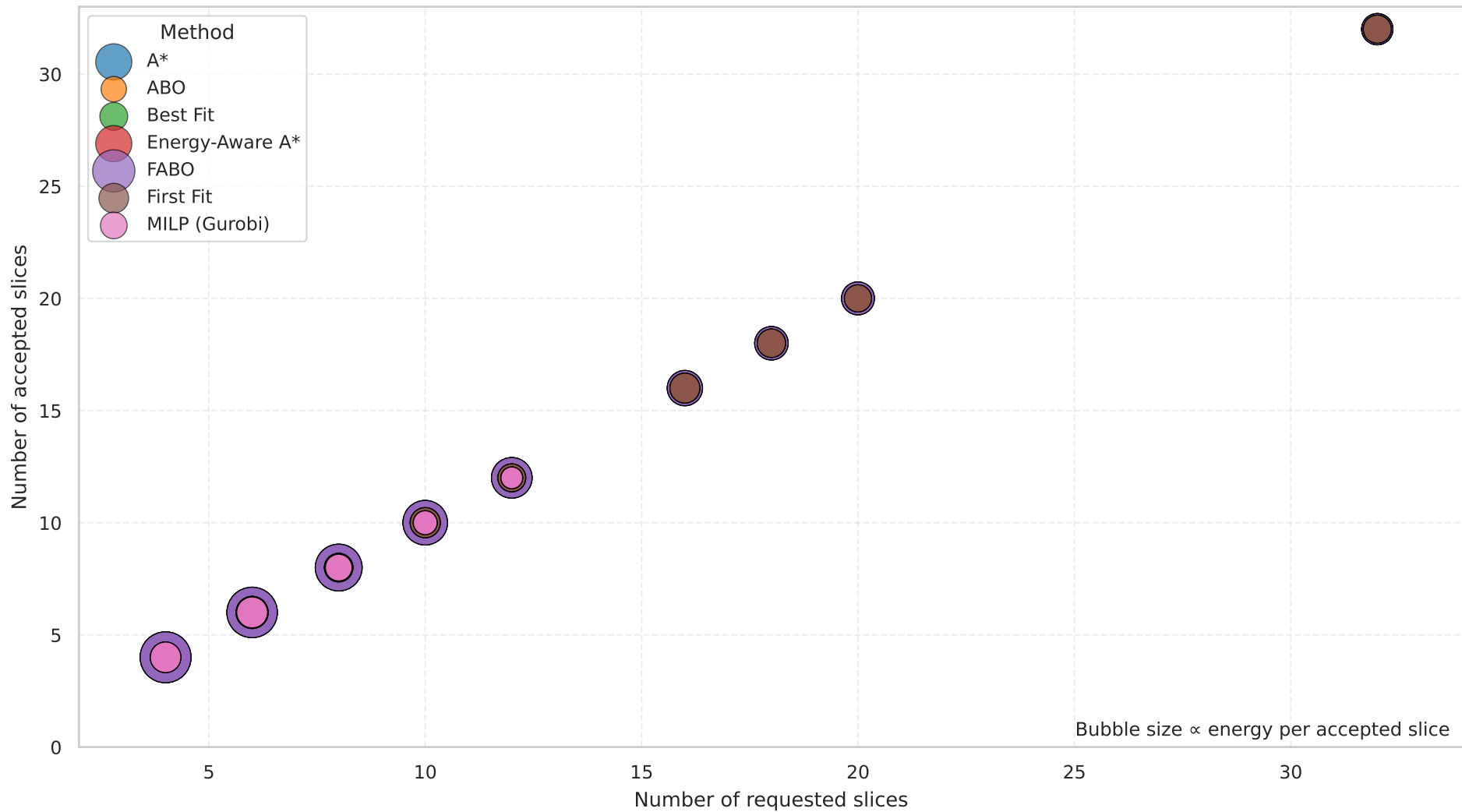
Bubble plot — Energy per accepted slice (size) 2 VNFs per slice
