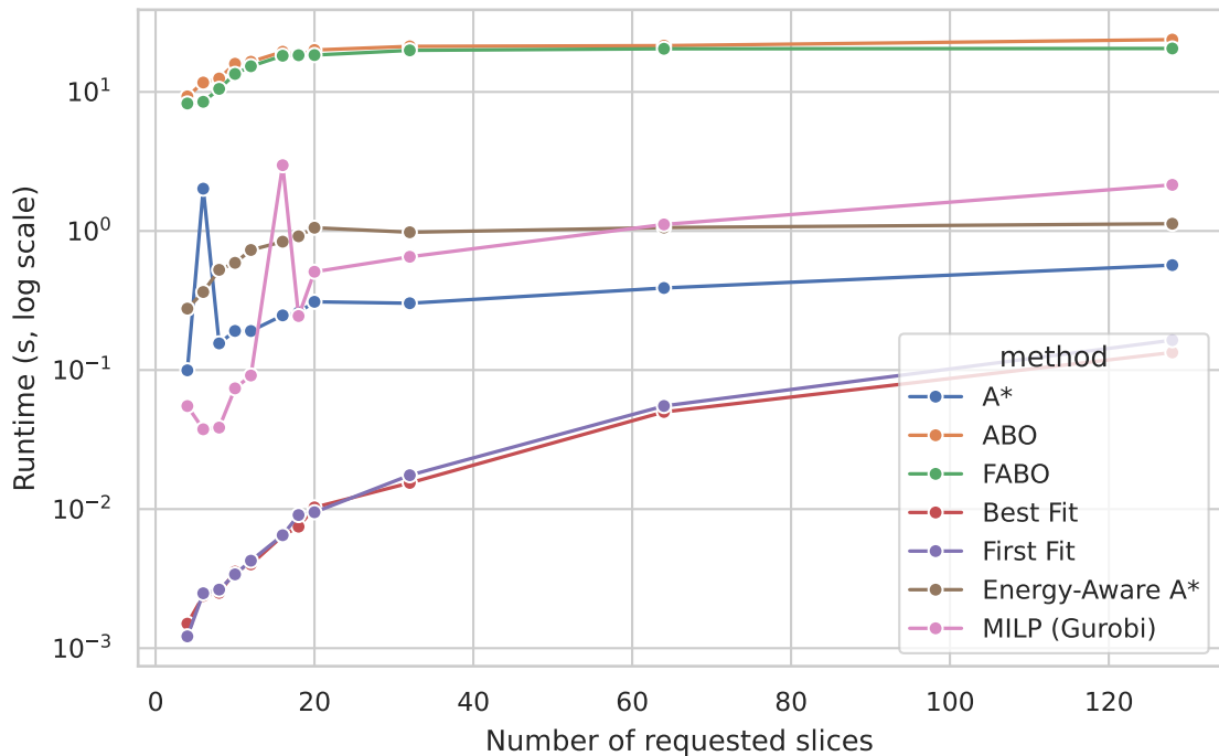
Runtime vs load — 3 VNFs per slice
