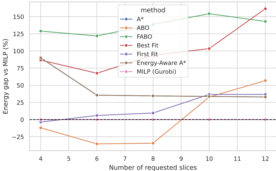
Energy optimality gap — 2 VNFs per slice
