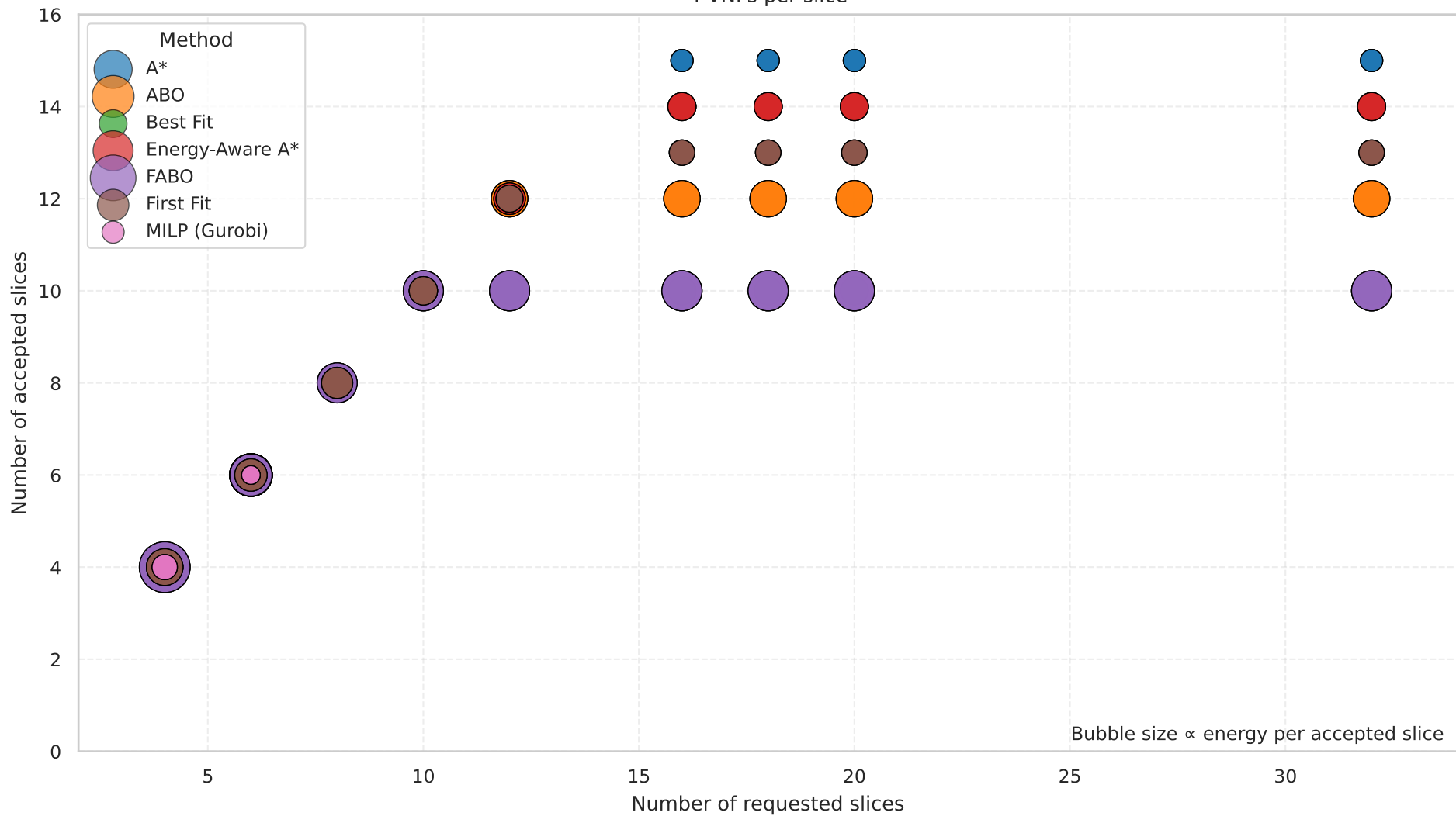
Bubble plot — Energy per accepted slice (size) 4 VNFs per slice
