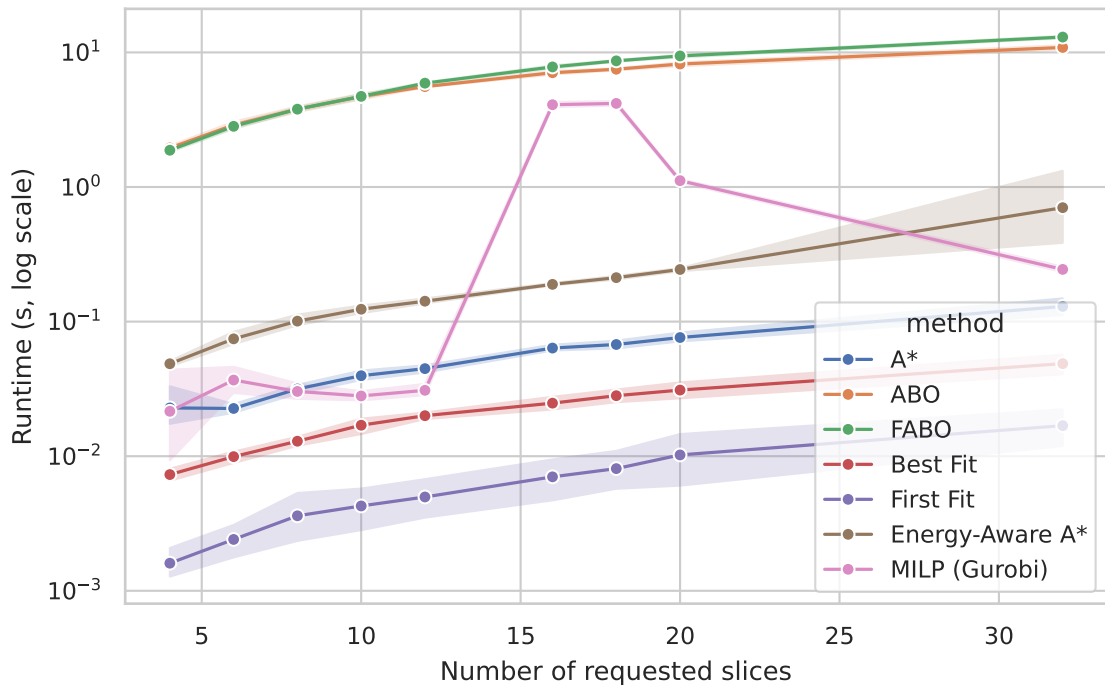
Runtime vs load — 2 VNFs per slice
