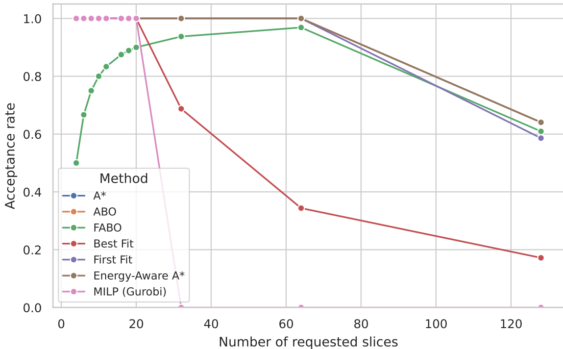
Acceptance vs Load — 3 VNFs per slice
