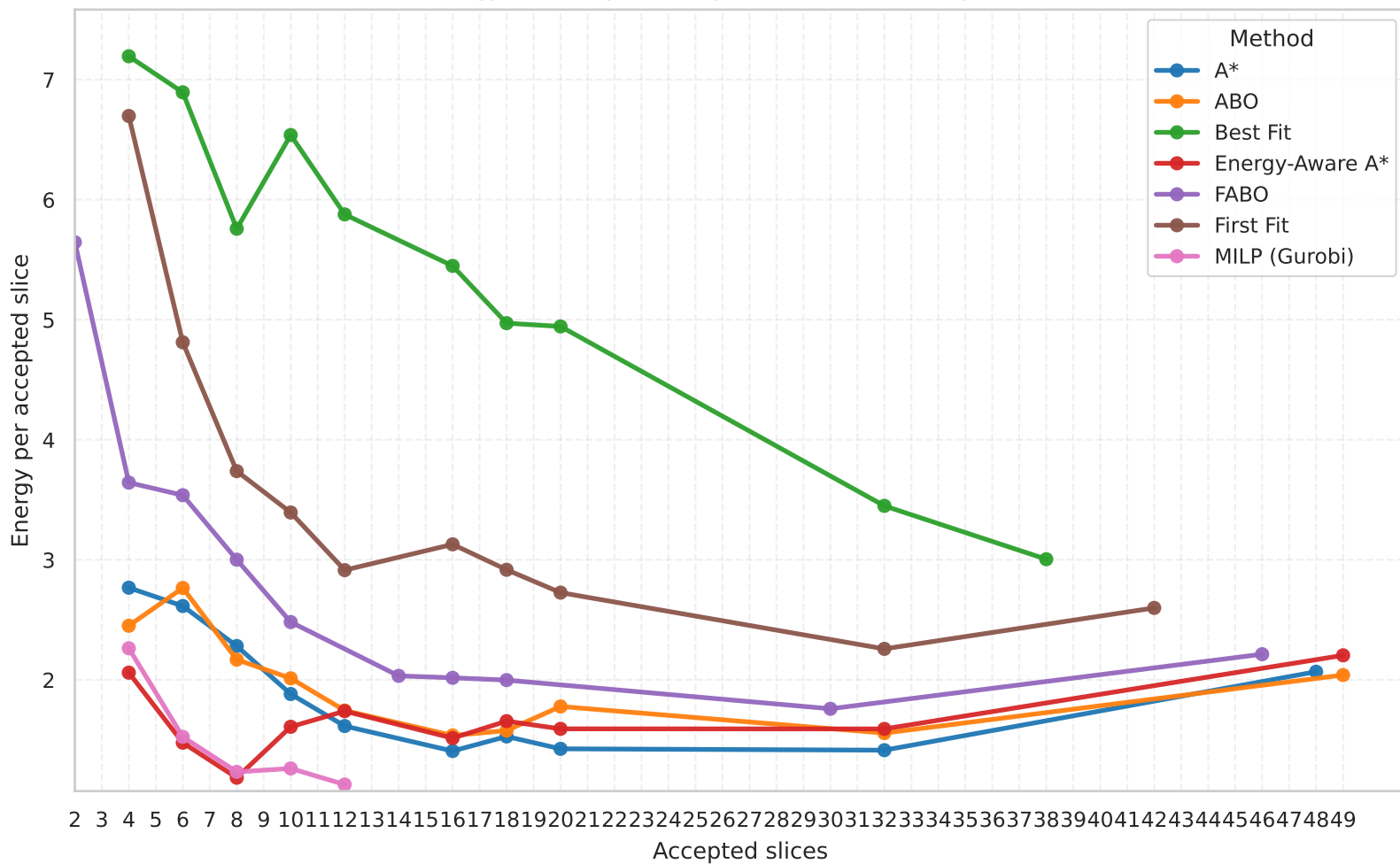
Energy Efficiency vs Accepted Slices — 4 VNFs per slice
