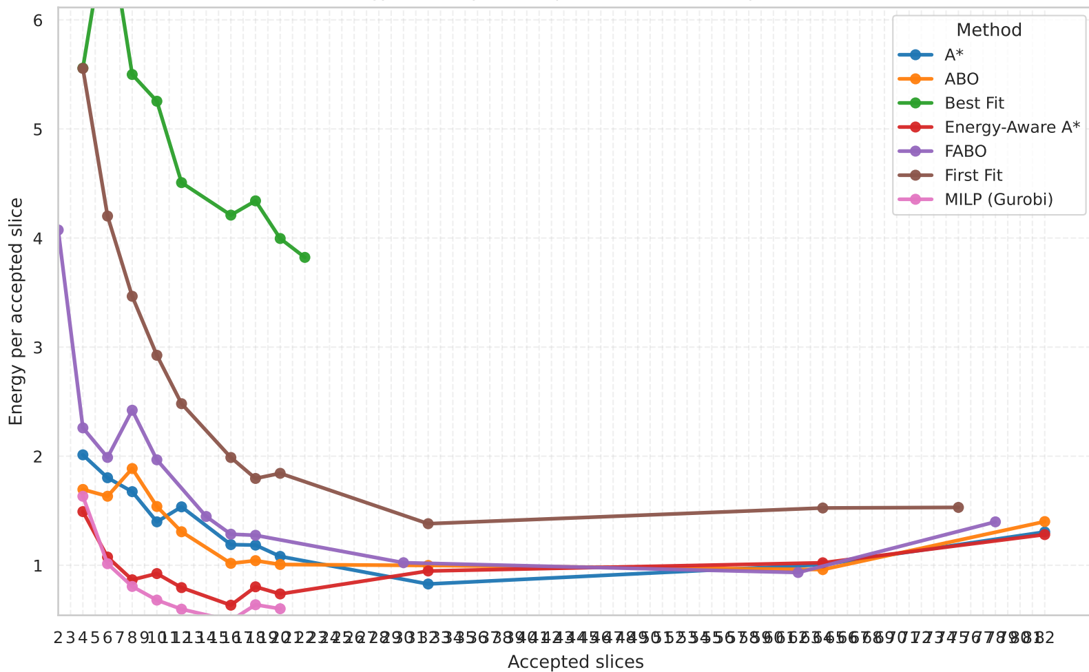
Energy Efficiency vs Accepted Slices — 3 VNFs per slice
