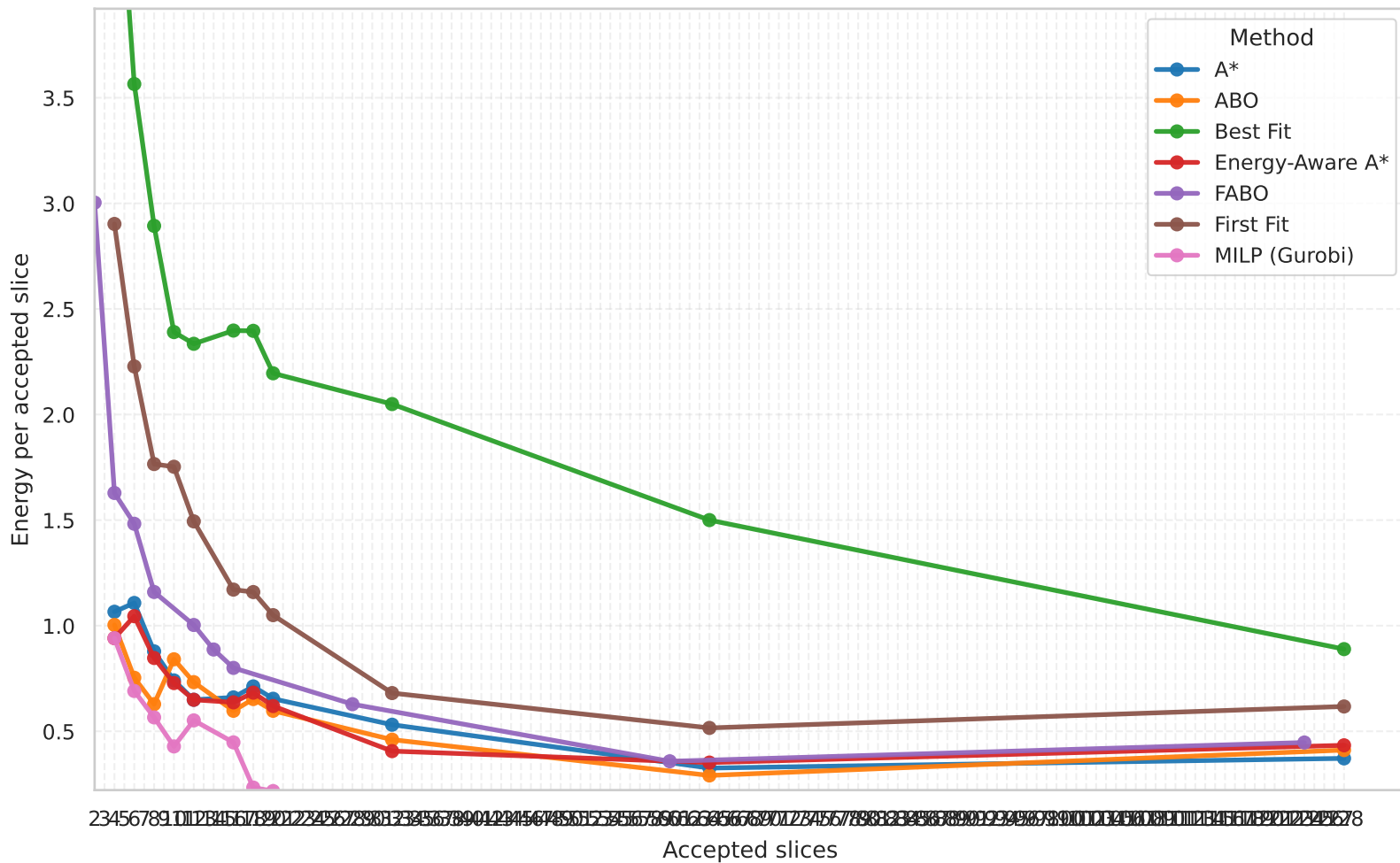
Energy Efficiency vs Accepted Slices — 2 VNFs per slice
