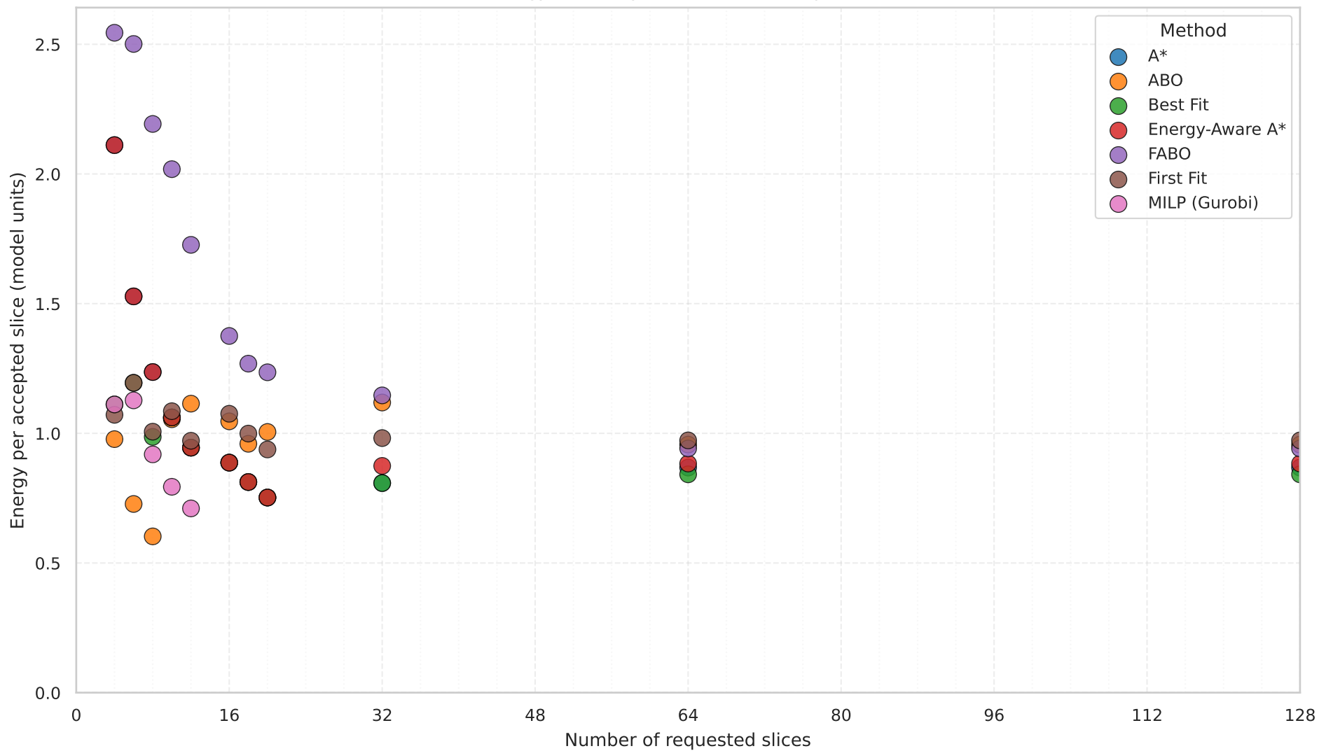
Energy Efficiency vs Load — 2 VNFs per slice
