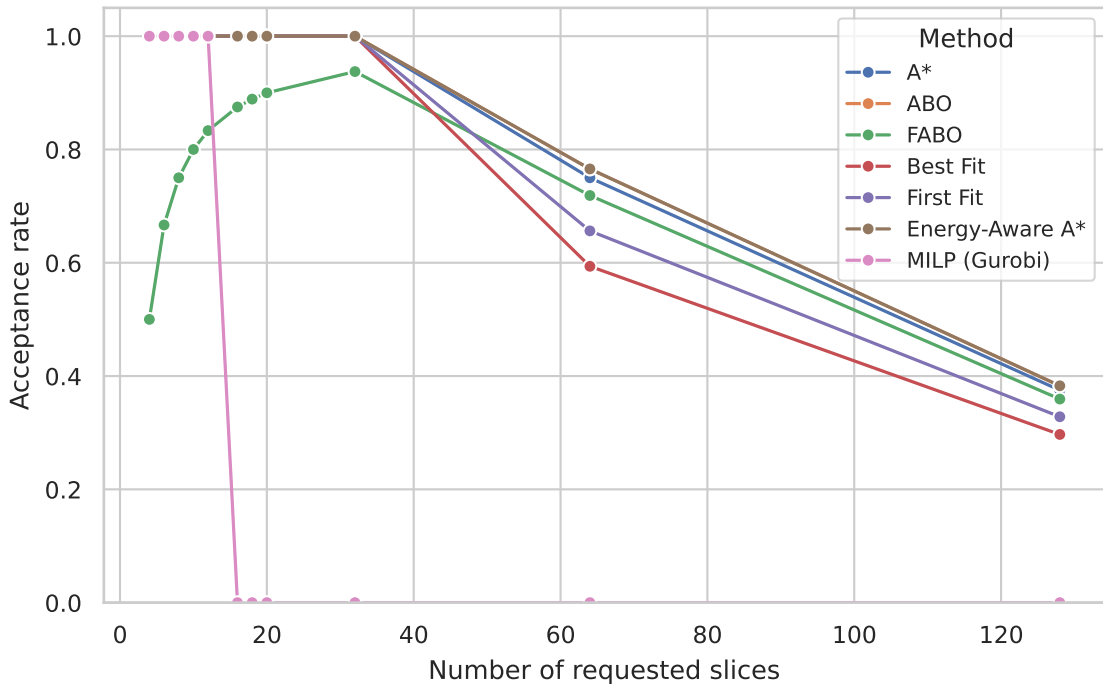
Acceptance vs Load — 4 VNFs per slice
