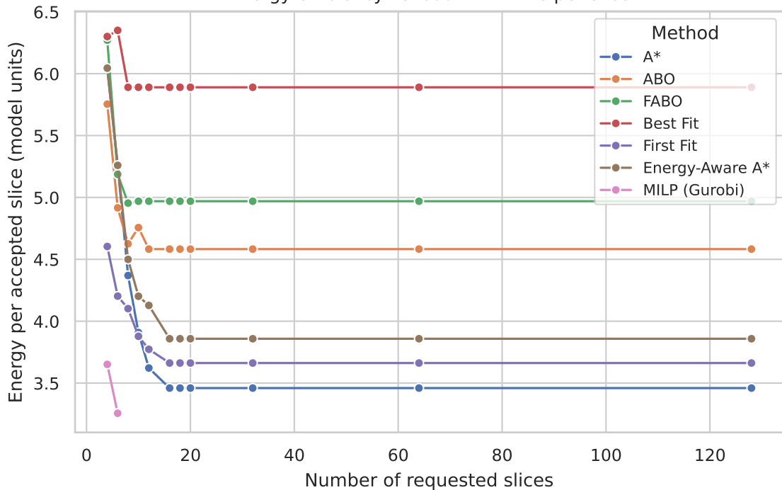
Energy efficiency vs load — 4 VNFs per slice
