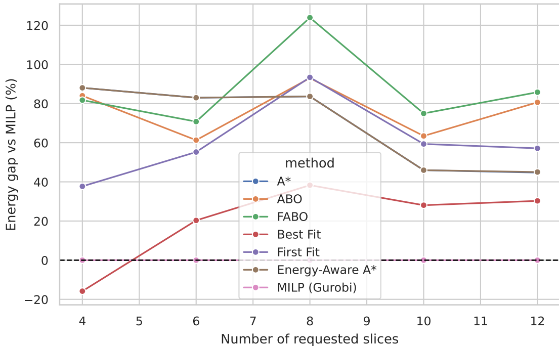
Energy optimality gap — 3 VNFs per slice
