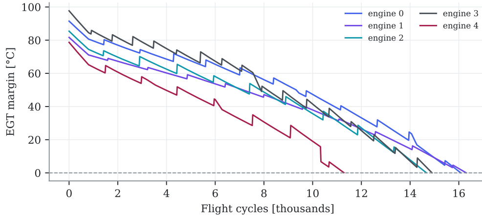
Figure 6.2: EGT-margin trajectories of five engines. Wash events produce the sawtooth recoveries; engine-to-engine spread comes from the hierarchical severity multipliers and the drawn new-engine margins. End of life is the zero crossing. Auto-generated from the fleet.
