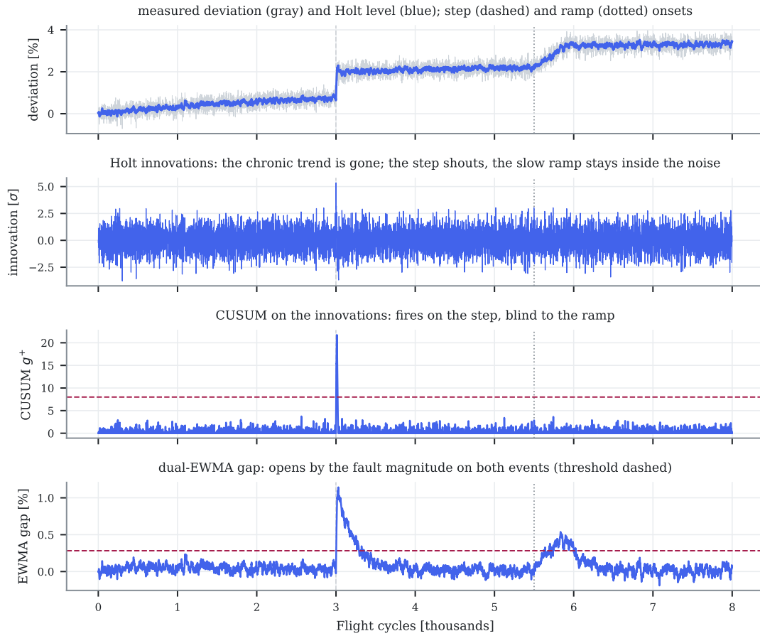
Figure 7.1: Anatomy of the detection stack on a synthetic deviation series with a chronic trend, an acute step (dashed) and a slow ramp (dotted), computed with the pipeline’s own Holt/CUSUM/EWMA primitives. The innovations (second panel) remove the chronic trend — lesson one; the CUSUM on them (third) catches the step but is blind to the ramp, which only the dual-EWMA gap (fourth) captures — lesson two. Auto-generated.
