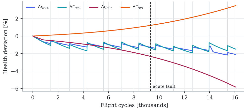
Figure 6.3: Ground-truth health parameters of one engine with an acute fault episode (dashed marker). Vertical gray lines are washes (visible as sawtooth in the HPC traces); the hot-section traces show the monotone efficiency loss and flow-capacity opening. Auto-generated.
