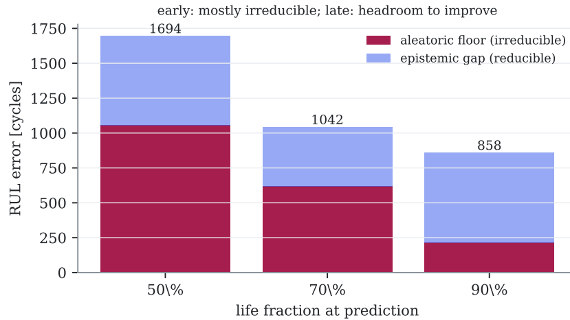
Figure 13.2: The prognostic floor (tag prereg-v11 ). Red: the ground-truth aleatoric floor — the RUL spread that survives conditioning on the engine's exact current health. Blue: the epistemic gap between the best achieved method (label) and that floor. Early in life the floor dominates; late in life a 4× reducible gap opens.
