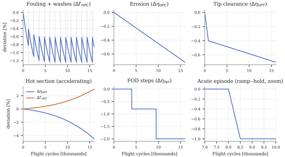
Figure 6.1: The six degradation time profiles at unit severity, drawn by evaluating the generator’s own trajectory code on the versioned fault catalog (norm N4): fouling with its wash sawtooth (Eq. (6.2)), linear erosion (Eq. (6.3)), bilinear tip clearance (Eq. (6.4)), accelerating hot section — efficiency down, flow capacity up (Eq. (6.5)) — FOD steps, and an acute ramp–hold episode (Eq. (6.6); zoomed, illustrative onset). Auto-generated.
