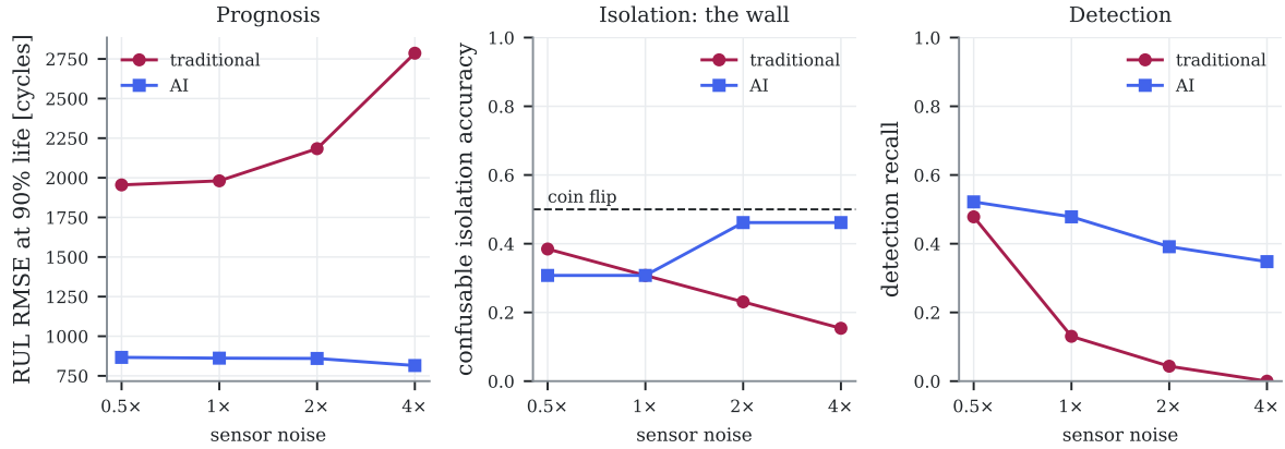
Figure 13.14: How the two tuned families degrade as sensor noise is scaled from half to four times its nominal value, on prognosis (left), confusable isolation (centre) and detection (right). The 1× point is the fleet every other chapter uses. Auto-generated.
