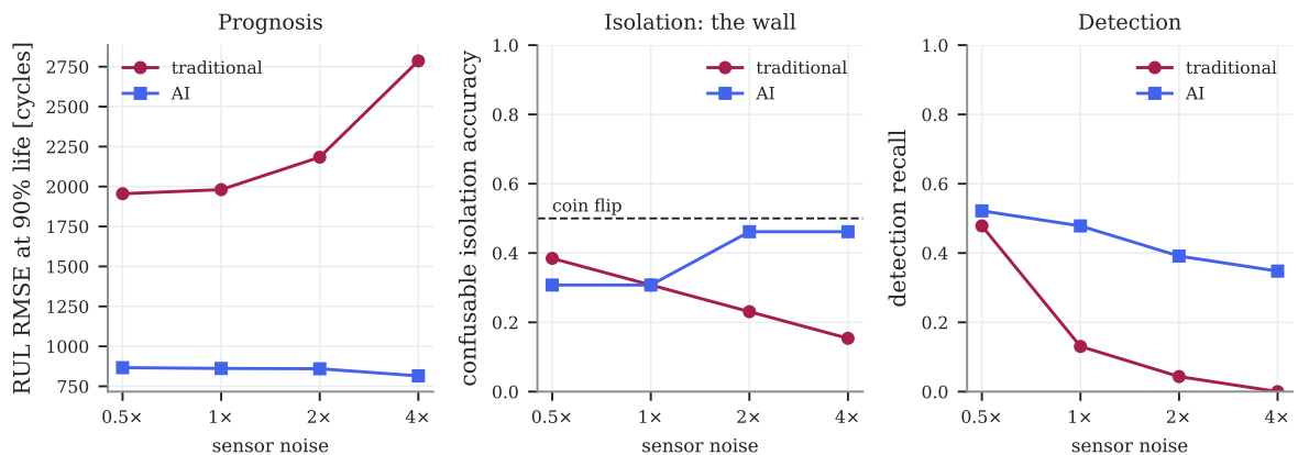
Figure 13.17: How the two tuned families degrade as sensor noise is scaled from half to four times its nominal value, on prognosis (left), confusable isolation (centre) and detection (right). The 1\times point is the fleet every other chapter uses. Auto-generated.
