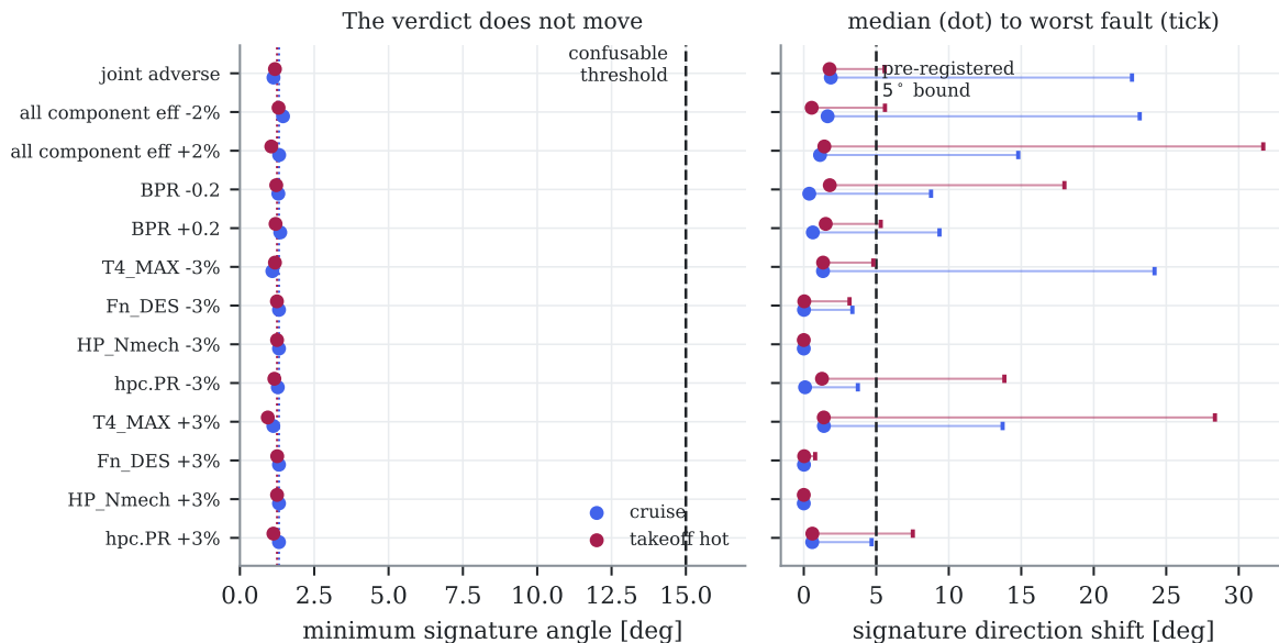
Figure 13.16: L-ICM. Left: the minimum cockpit signature angle under every calibration perturbation, at both snapshot conditions; dotted lines are the nominal values, the dashed line the 15^\circ confusability threshold. Right: how far each fault signature rotates (dot = median over the ten health parameters, tick = worst one) against the pre-registered 5^\circ bound. Auto-generated.
