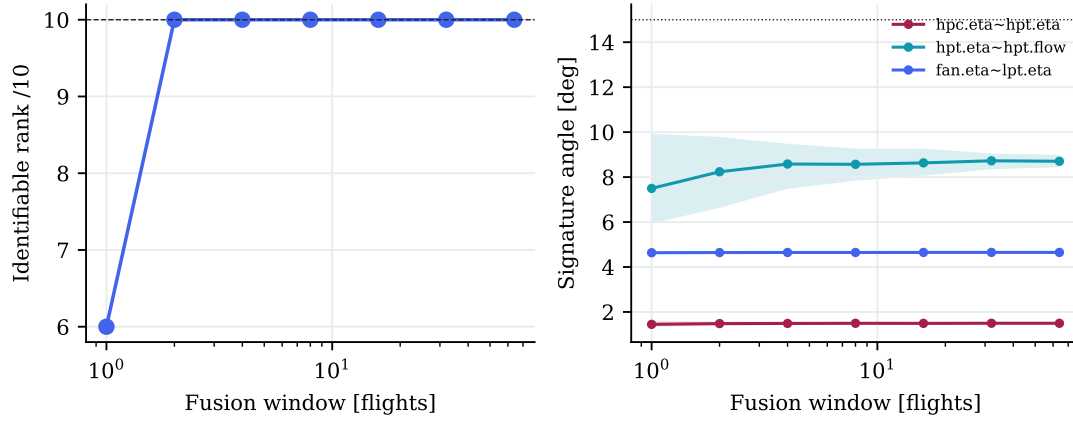
Figure 10.1: Observability under realistic in-service scatter (200 draws per window size). Left: identifiable rank recovers immediately. Right: signature angles saturate — free scatter is too narrow to keep paying. Auto-generated.
