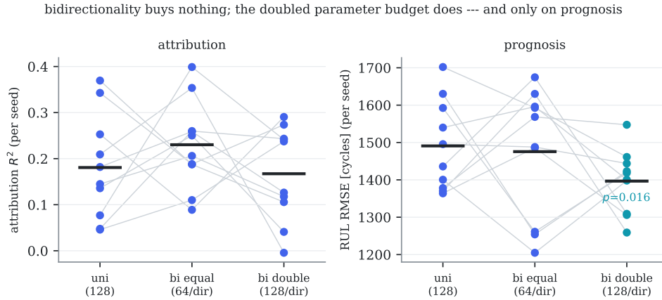
Figure 13.15: Direction against capacity on both tasks; grey lines join the same seed across arms, which is the pairing the statistics use. Auto-generated ( prereg-v21 ).
