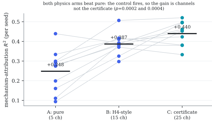
Figure 13.13: Per-seed attribution score for the three arms; grey lines join the same seed across arms, which is the pairing the statistics use. Auto-generated ( prereg-v20 ).
