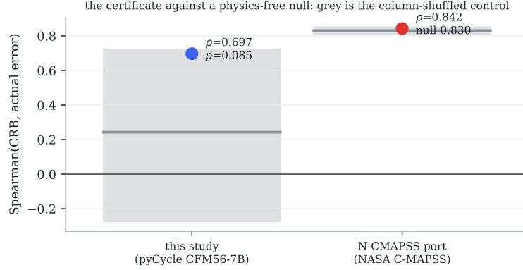
Figure 13.18: The honesty correlation against its own null. Grey spans the 5th–95th percentile of 200 column-shuffled draws, in which the influence matrix carries no physics. Auto-generated (prereg-v25).
