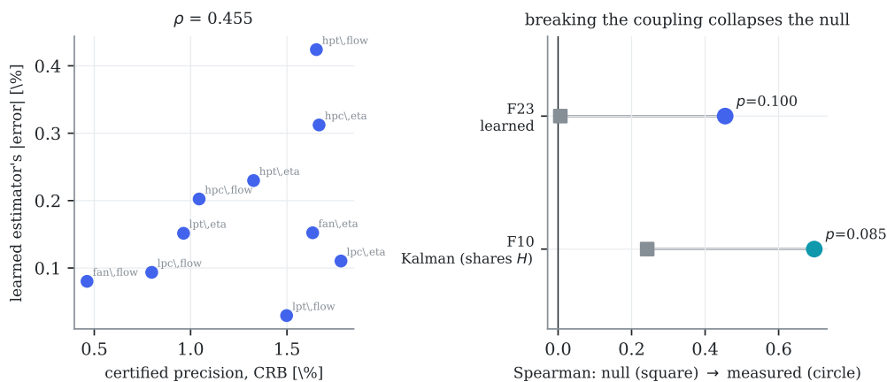
Figure 13.19: Left: certified precision against the learned estimator’s true per-direction error. Right: each test against its own null — square is the null, circle the measured value. Removing the shared matrix collapses the null from 0.242 to 0.006. Auto-generated ( prereg-v26 ).
