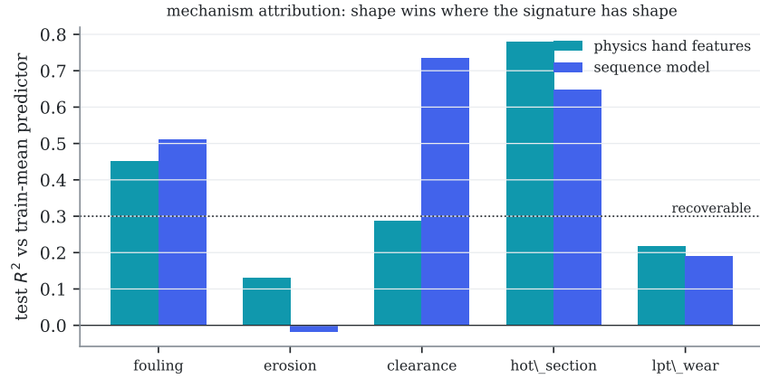
Figure 13.10: Per-mechanism attribution from the deviation trajectory, on held-out engines, under a symmetric tuning budget. The dotted line is the R^2 = 0.30 recoverability mark. Auto-generated (prereg-v16).
