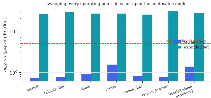
Figure 13.16: Confusable-pair angle at each calibrated operating point and over the whole measured envelope, noise-whitened, log scale. Auto-generated ( prereg-v19 ).
