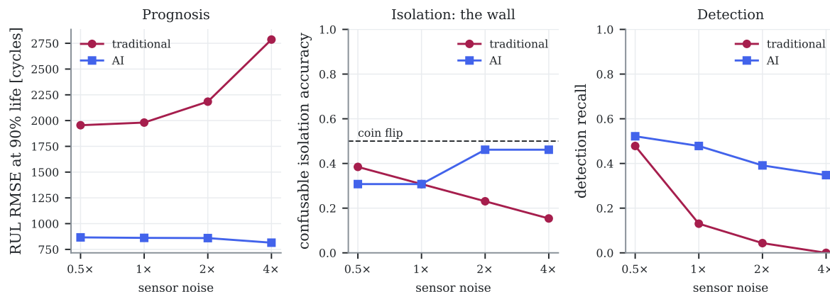
Figure 13.21: How the two tuned families degrade as sensor noise is scaled from half to four times its nominal value, on prognosis (left), confusable isolation (centre) and detection (right). The 1× point is the fleet every other chapter uses. Auto-generated.
