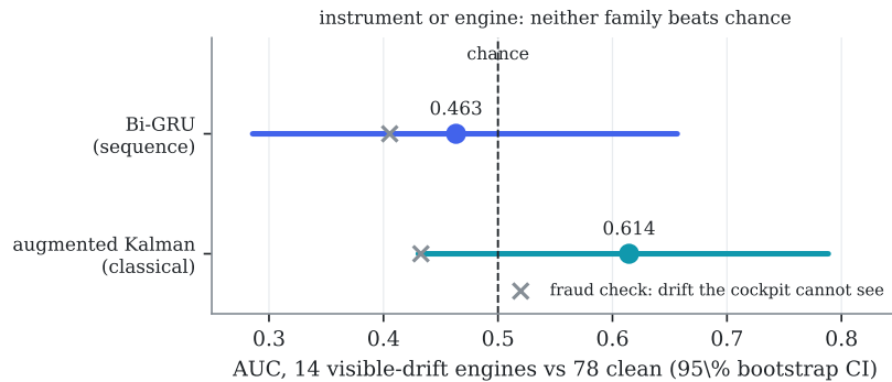
Figure 13.11: Separating a drifting sensor from a real fault, 14 visible-drift engines against 78 clean, bootstrap intervals grouped by engine. Crosses mark the fraud check: engines whose drift is on a channel the cockpit set cannot see. Auto-generated ( prereg-v18 ).
