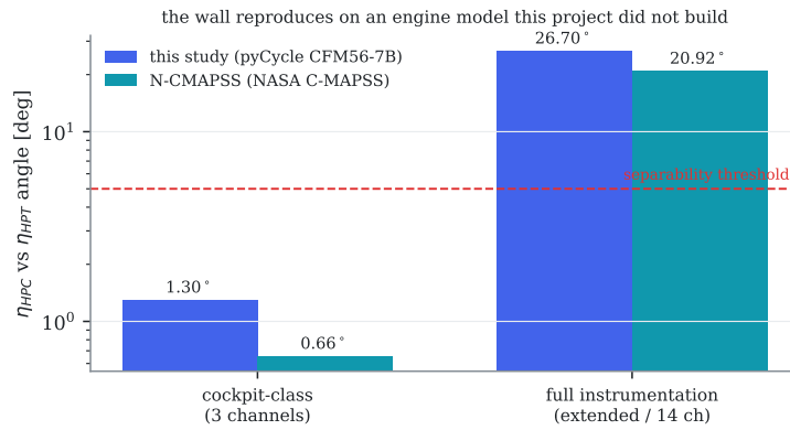
Figure 13.17: The \eta_{HPC} against \eta_{HPT} angle on two independent engine models, log scale. Cockpit-class channels are \{N_2, W_f, EGT\} here and their N-CMAPSS analogues \{N_c, W_f, T_{48}\} . Auto-generated ( prereg-v23 ).
