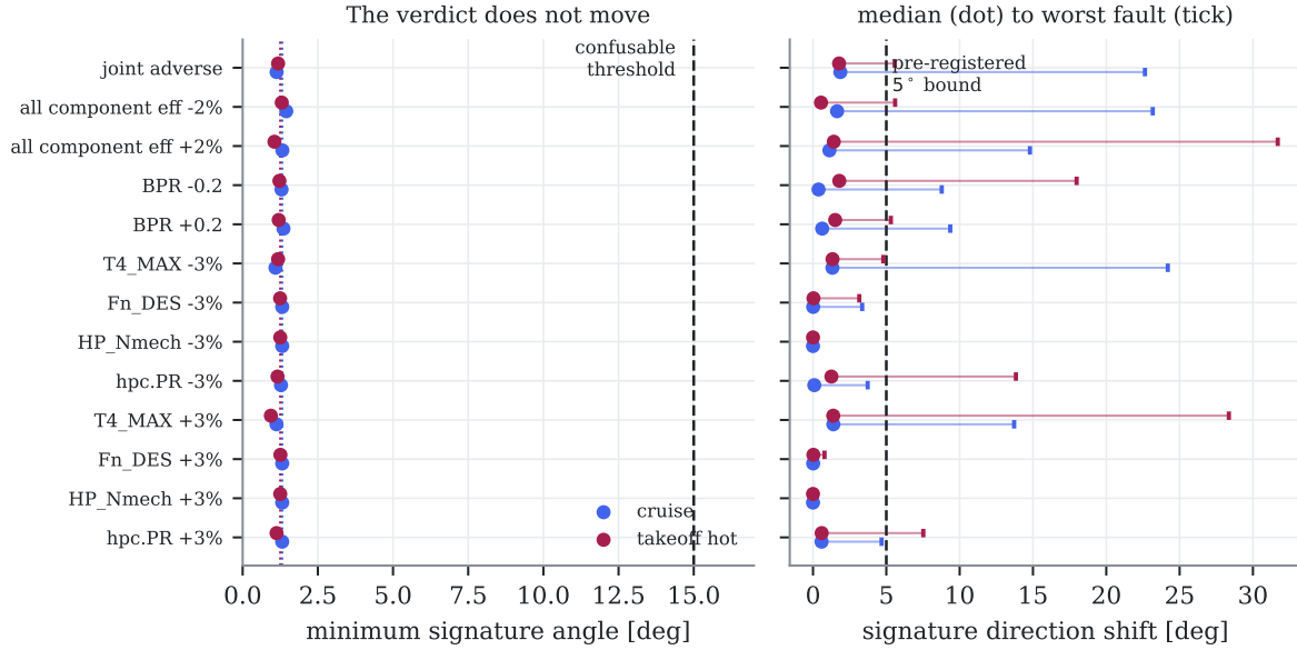
Figure 13.19: L-ICM. Left: the minimum cockpit signature angle under every calibration perturbation, at both snapshot conditions; dotted lines are the nominal values, the dashed line the 15^\circ confusability threshold. Right: how far each fault signature rotates (dot = median over the ten health parameters, tick = worst one) against the pre-registered 5^\circ bound. Auto-generated.
