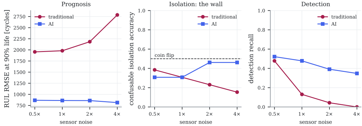
Figure 13.20: How the two tuned families degrade as sensor noise is scaled from half to four times its nominal value, on prognosis (left), confusable isolation (centre) and detection (right). The 1× point is the fleet every other chapter uses. Auto-generated.
