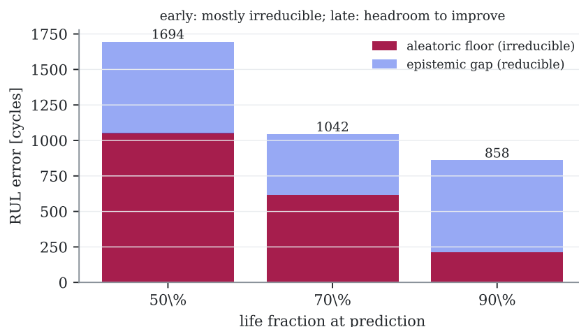
Figure 14.2: The prognostic floor (tag prereg-v11 ). Red: the ground-truth aleatoric floor — the RUL spread that survives conditioning on the engine’s exact current health. Blue: the epistemic gap between the best achieved method (label) and that floor. Early in life the floor dominates; late in life a 4\times reducible gap opens.
