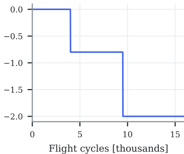
FOD steps ( \Delta\eta_{fan} )
