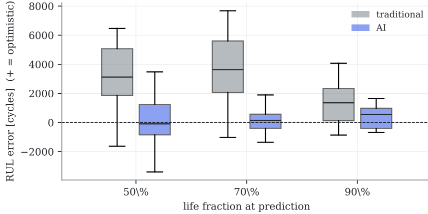
Figure 9.1: Per-engine confirmatory RUL error, traditional versus AI, at three life fractions (positive = optimistic; boxes span the interquartile range). The evidence is in the shape, not just the RMSE: the traditional errors are wide and skewed optimistic, the AI’s are tight and near-unbiased. Auto-generated from the tuned test-fleet predictions.
