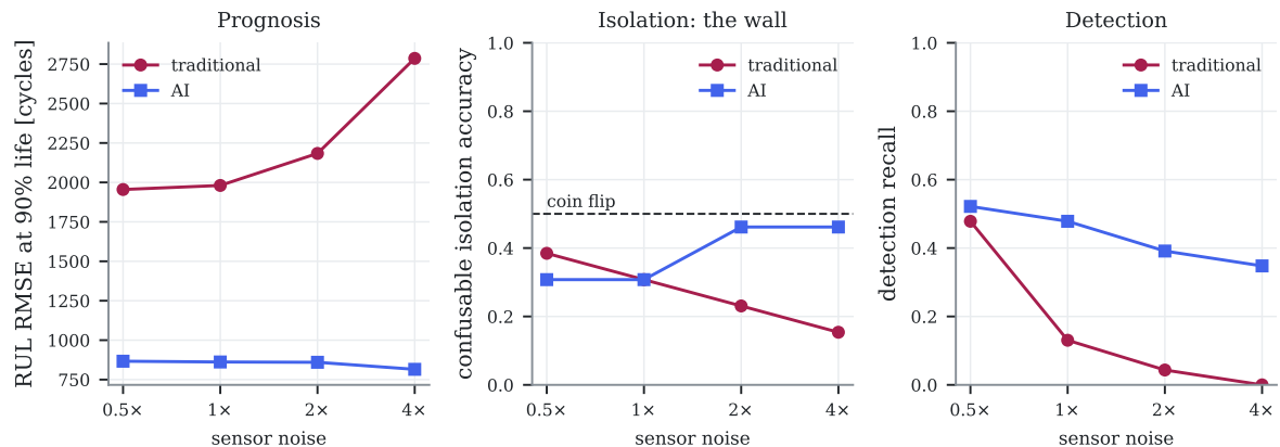
Figure 13.19: How the two tuned families degrade as sensor noise is scaled from half to four times its nominal value, on prognosis (left), confusable isolation (centre) and detection (right). The 1× point is the fleet every other chapter uses. Auto-generated.
