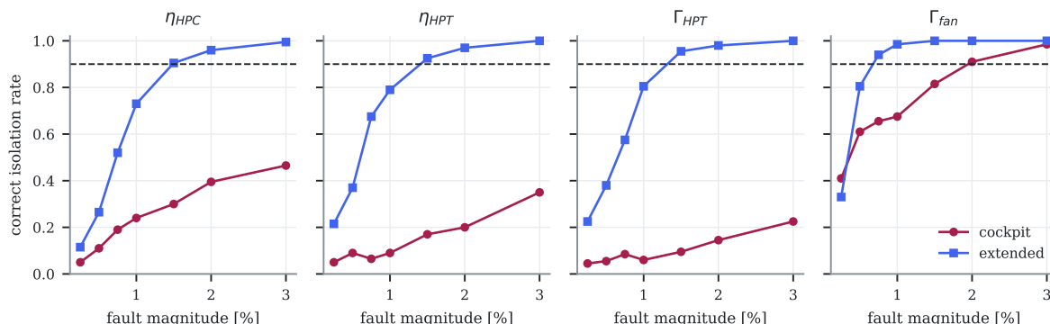
Figure 5.3: Correct-isolation rate against fault magnitude for four representative parameters, cockpit versus extended sensors; the dashed line is the 90 % criterion. The extended set crosses it between 0.75 and 1.5 % for most faults; the cockpit set mostly never does within the 3 % range swept. Auto-generated.
