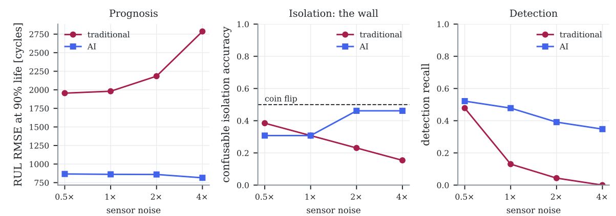
Figure 13.18: How the two tuned families degrade as sensor noise is scaled from half to four times its nominal value, on prognosis (left), confusable isolation (centre) and detection (right). The 1\times point is the fleet every other chapter uses. Auto-generated.
