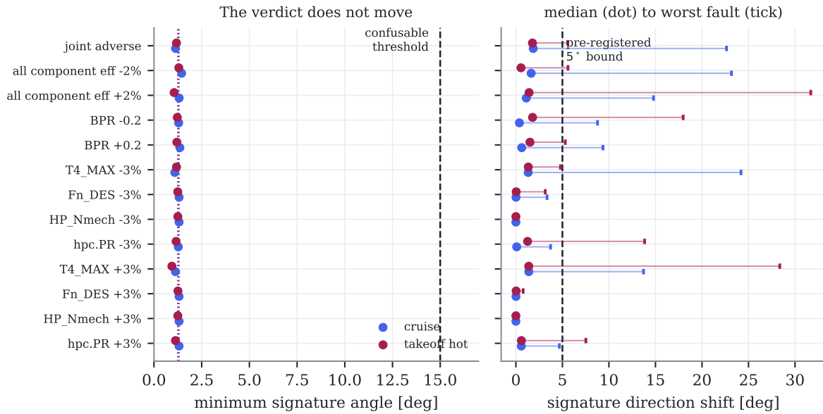
Figure 13.17: L-ICM. Left: the minimum cockpit signature angle under every calibration perturbation, at both snapshot conditions; dotted lines are the nominal values, the dashed line the 15^\circ confusability threshold. Right: how far each fault signature rotates (dot = median over the ten health parameters, tick = worst one) against the pre-registered 5^\circ bound. Auto-generated.
