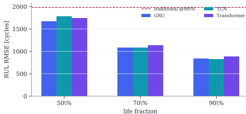
Figure 12.4: L5: RUL RMSE (mean of three seeds) for three AI architectures under equal effort; all sit far below the tuned traditional baseline at 90 % life (dashed). The advantage is the learning, not the architecture. Auto-generated.
