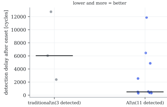
Figure 9.1: Detection lead time: one dot per detected episode, with the median bar. The AI detects far more episodes (11 vs 3) and far sooner (median 499 vs 6033 cycles after onset) at equal false alarms. Auto-generated.
