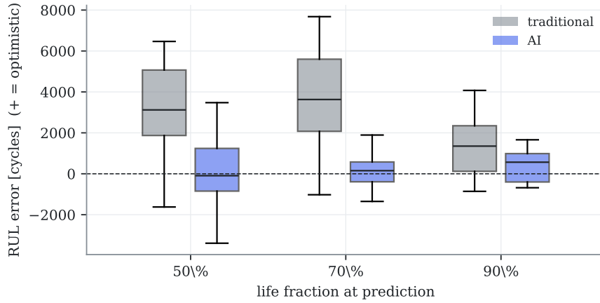
Figure 9.3: Per-engine confirmatory RUL error, traditional versus AI, at three life fractions (positive = optimistic; boxes span the interquartile range). The evidence is in the shape, not just the RMSE: the traditional errors are wide and skewed optimistic, the AI’s are tight and near-unbiased. Auto-generated from the tuned test-fleet predictions.
