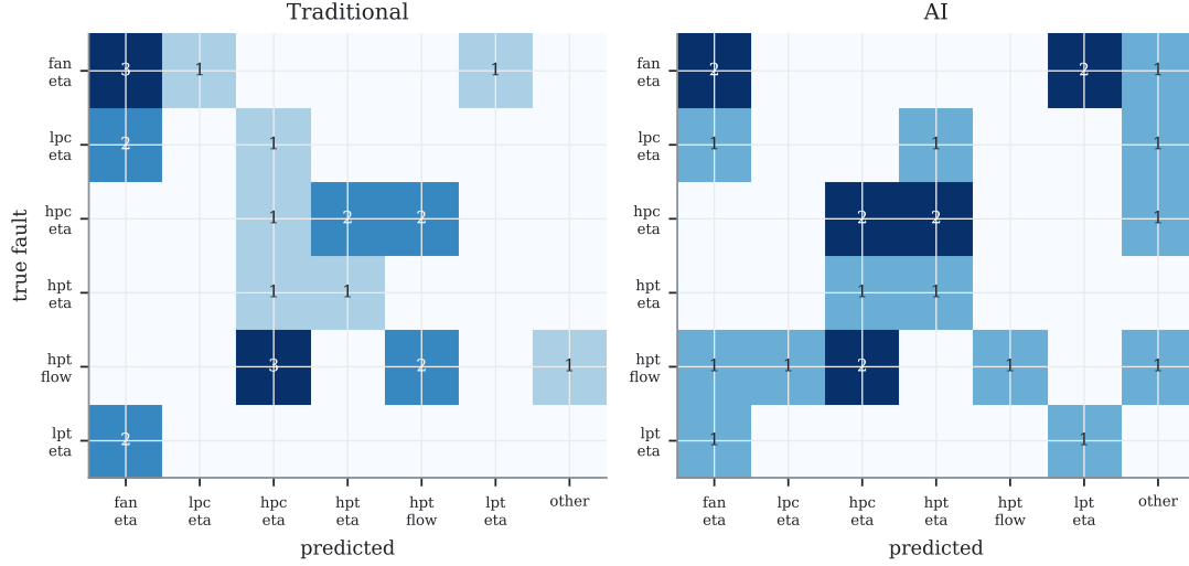
Figure 9.2: Isolation confusion matrices on the test episodes: true fault (rows) versus predicted (columns), traditional (left) and AI (right). Neither concentrates on the diagonal — both scatter faults onto confusable neighbours (e.g. toward fan.eta and hpc.eta ), the mechanism behind the H2 tie. Auto-generated.
