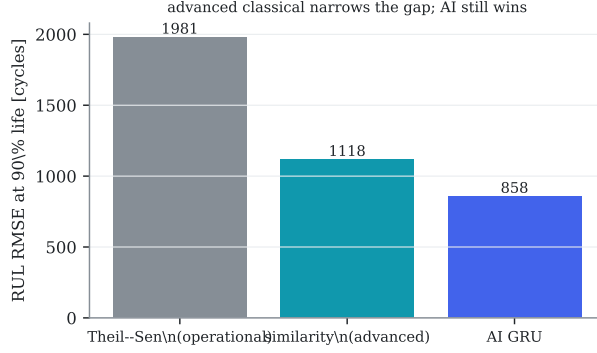
Figure 13.7: RUL error at 90 % life for the operational (Theil-Sen), advanced classical (similarity-based) and AI prognostics. The advanced method closes most of the gap to the AI, which still leads. Auto-generated.
