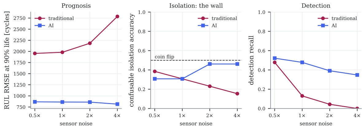
Figure 13.9: How the two tuned families degrade as sensor noise is scaled from half to four times its nominal value, on prognosis (left), confusable isolation (centre) and detection (right). The 1× point is the fleet every other chapter uses. Auto-generated.
