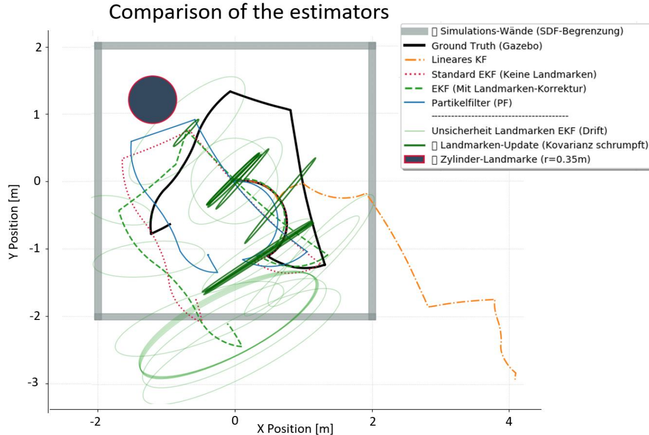
Figure 9: Example run ( Q = 1.0 , R = 0.01 ) where the EKF's estimated the Robot to drive through walls.
