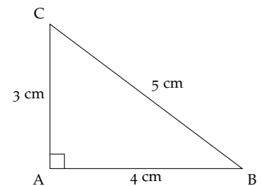
FIGURE 2.1: Un triangle rectangle
