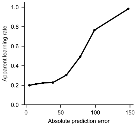
Change-point model (no prob. resp.)
