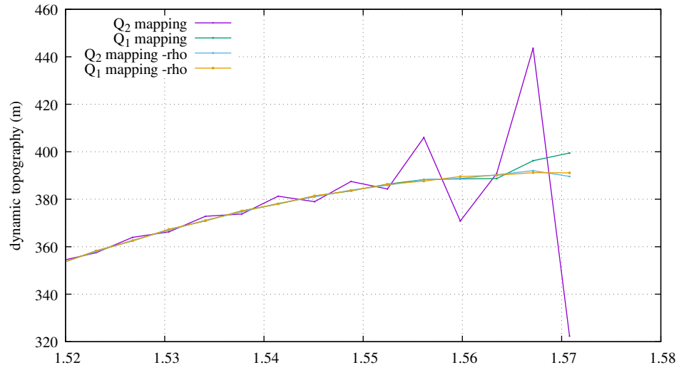
axisymmetric - res 428x64 - top surface
