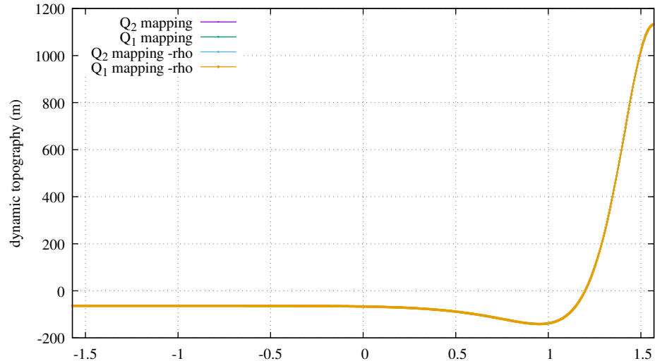
plane strain - res 428x64 - bottom surface
