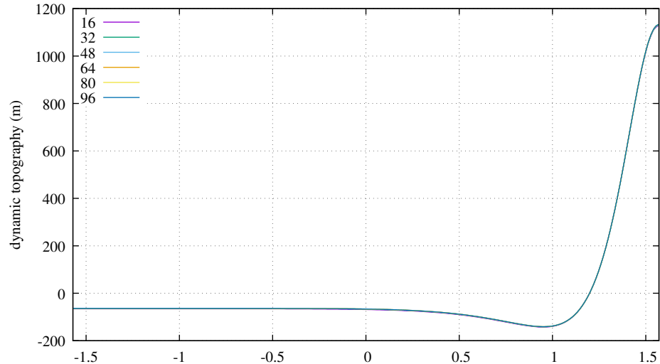
plane strain - bottom surface
