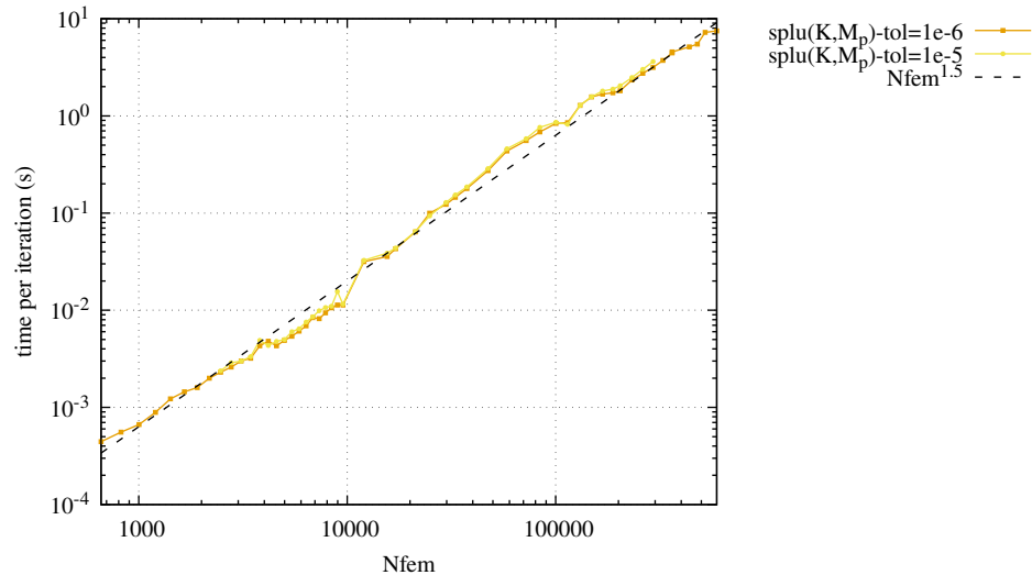
Stokes solve (time per iteration)
