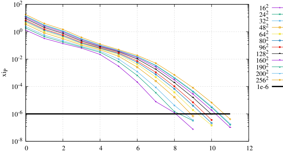
pressure convergence
