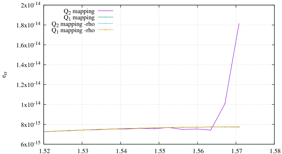
axisymmetric - res 428x64 - bottom surface
