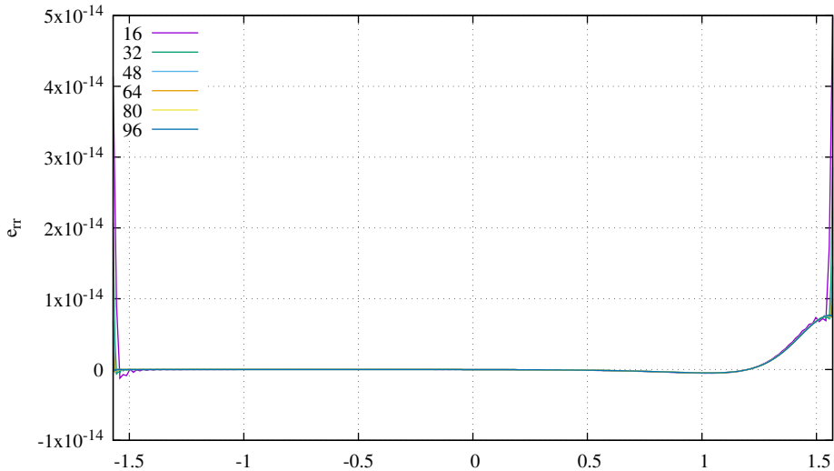
axisymmetric - bottom surface
