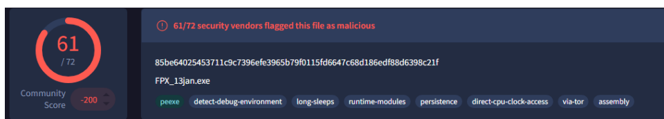
Figure 66: Malware 3
