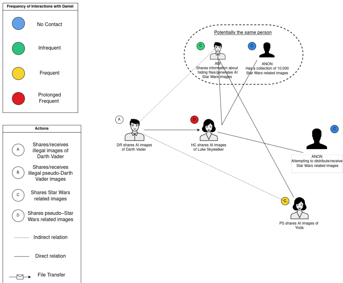
Figure 58: Relationship Chart
