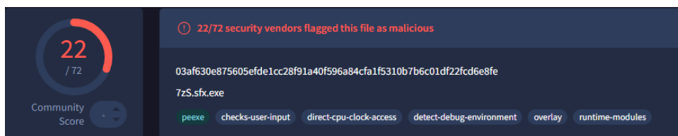
Figure 67: Malware 1
