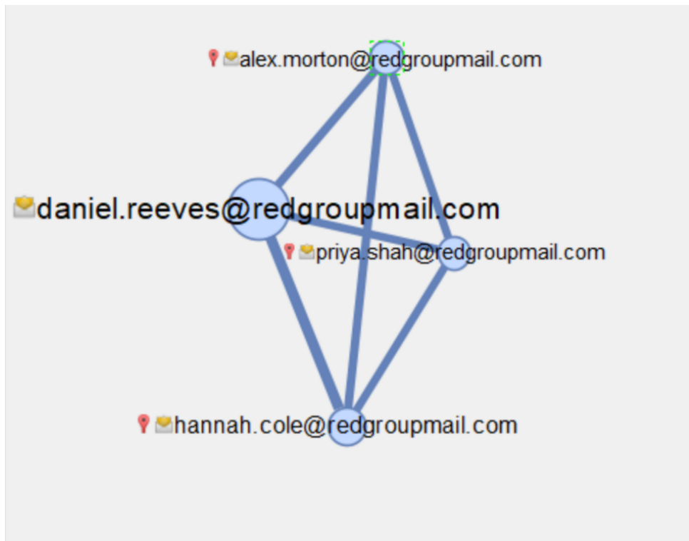
Figure 59: Relationship Chart 2
