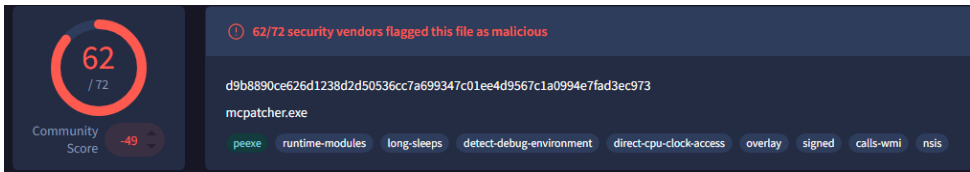
Figure 64: Malware 4
