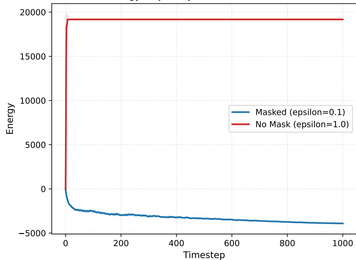
Energy Trajectory (G1, mean \pm 95% CI)
