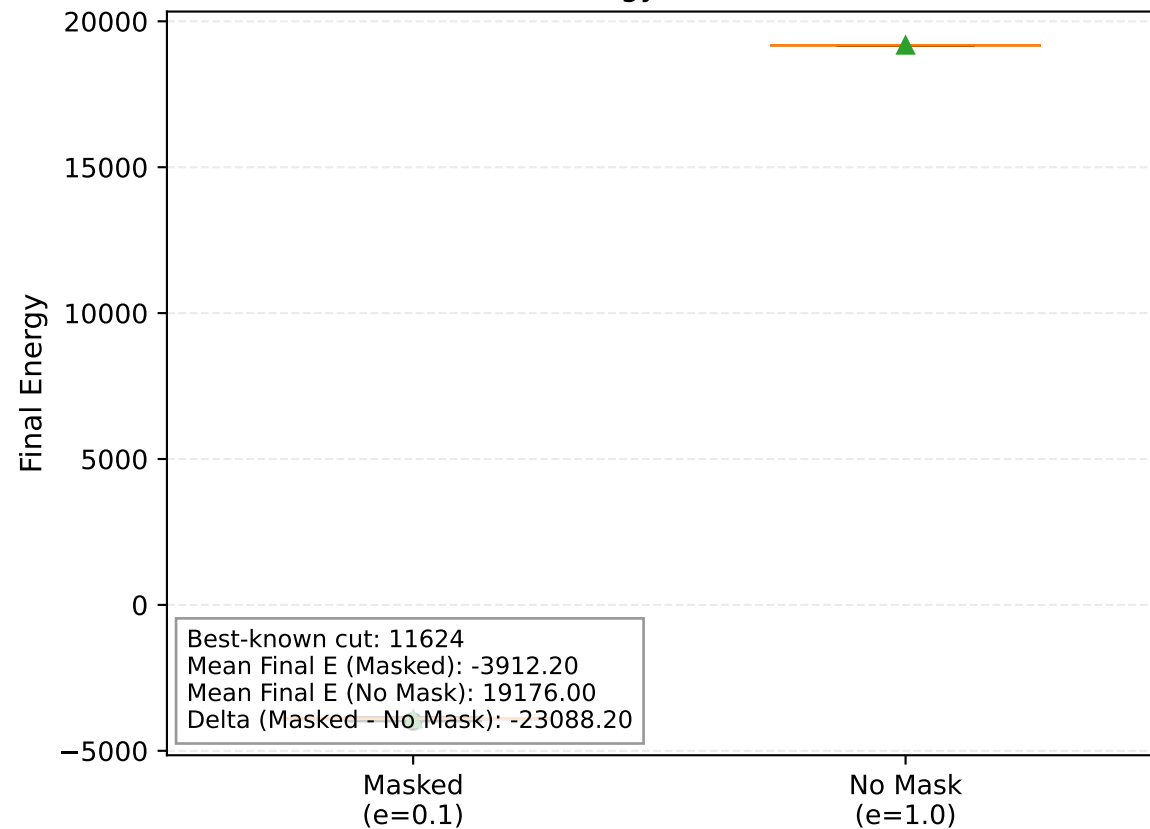
Final Energy Distribution
