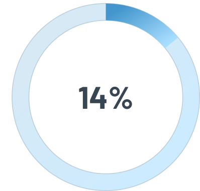
Virginica
