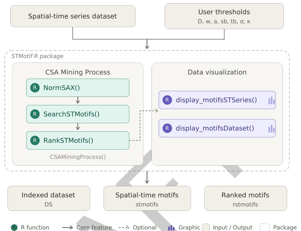
Figure 1: Figure 1: Main functionalities of STMotif, including normalization and SAX indexing, motif search, ranking, and visualization.
