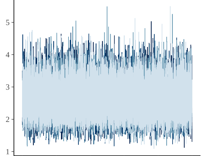
gamma[24]
