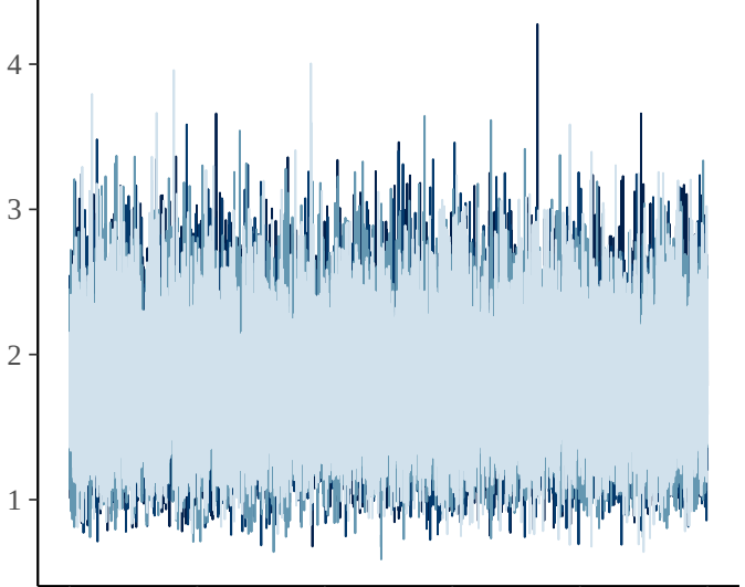
gamma[102]
