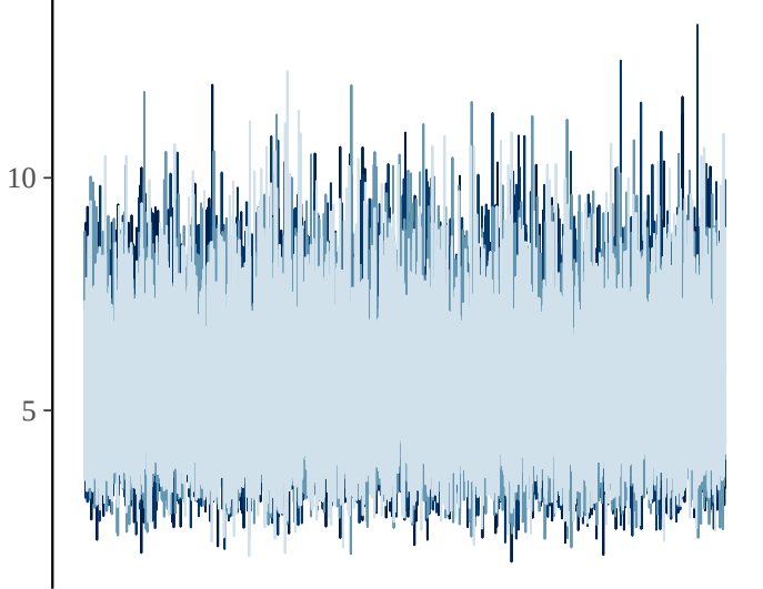
gamma[47]
