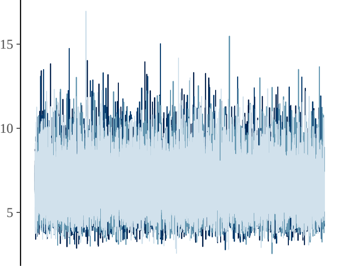
gamma[36]
