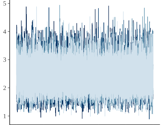
gamma[13]
