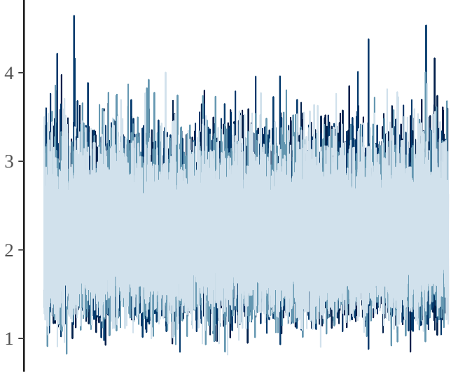
gamma[11]
