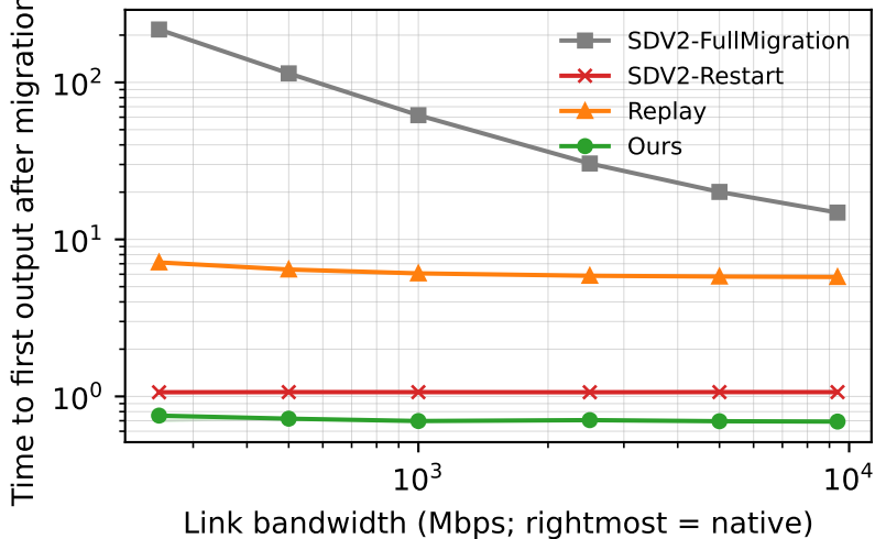
Execution handoff latency vs. bandwidth (median, p25-p75)
