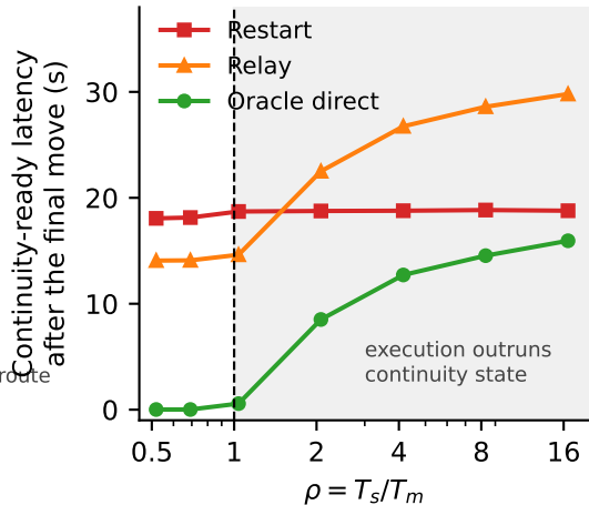
(b) Measured, A \rightarrow B \rightarrow C at 1 Gbps
